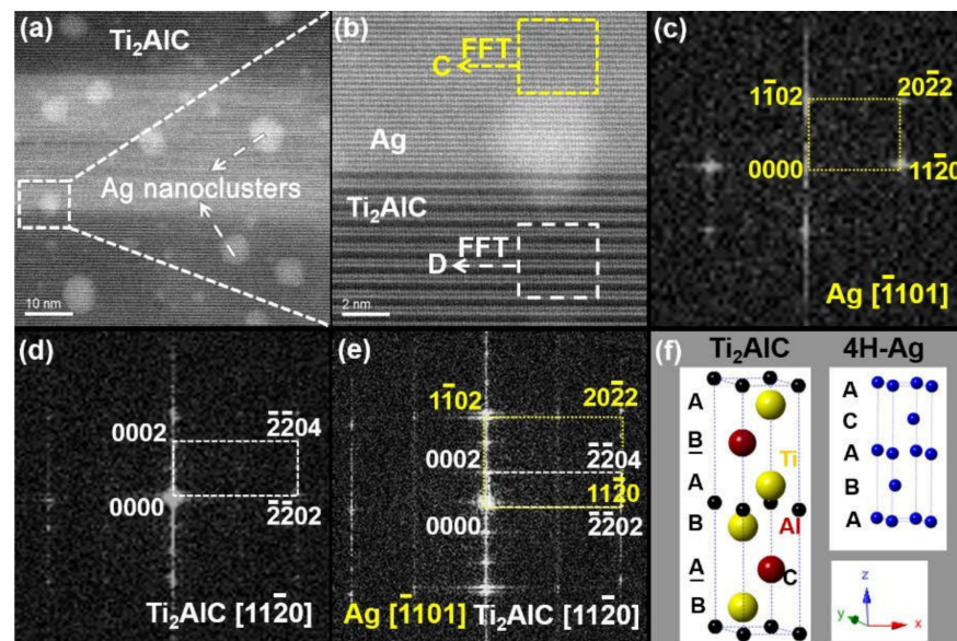
Figure 3. TEM results of the Ag– \text{Ti}_2\text{AlC} interaction zone along the crystallographic orientation of [\bar{1}1\bar{2}0]_{\text{Ti}_2\text{AlC}} : (a) HAADF–STEM image; (b) magnified white box in (a); (c,d) FFT (fast Fourier transformation) results of the Ag and \text{Ti}_2\text{AlC} in (b); (e) FFT result of the Ag– \text{Ti}_2\text{AlC} interface in (b); (f) schematic drawings of the crystal structures of 4H–Ag and \text{Ti}_2\text{AlC} .
