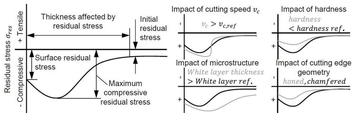
Figure 2. Stresses induced by hard turning and the qualitative impacts of the tool, process and initial material parameters [20, (reproduced from [21], with permission from authors, 2011)].
