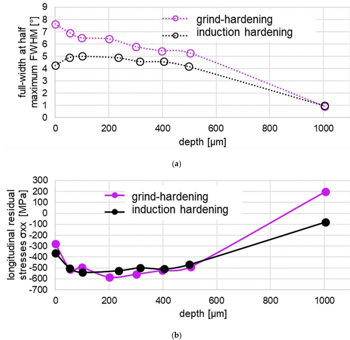
Figure 12. Longitudinal residual stress (a) and FWHM depth profiles (b) for thermally dominated processes: induction hardening and grind-hardening.
