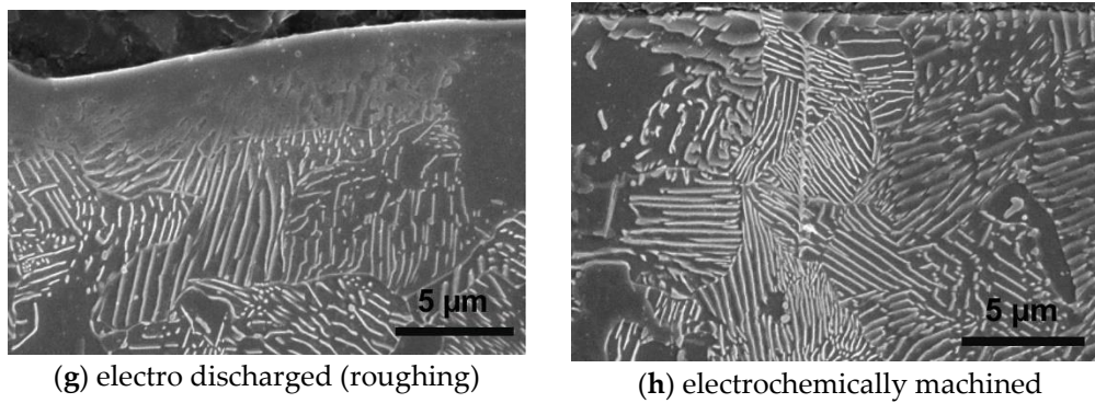
Figure 6. SE-micrographs of (a) deep rolled surface, (b) grinded strengthened surface, (c) turned surface, (d) grind hardened surface, (e) induction hardened surface (f) pulsed ( \mu s) laser processed surface, (g) electro discharged (roughing) machined surface and (h) electrochemically machined surface.
