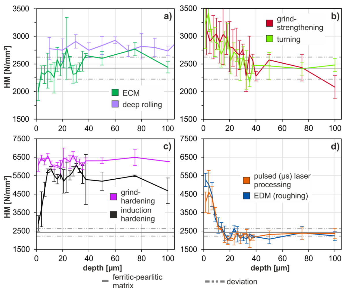
Figure 5. Martens hardness depth profiles of (a) ECM and deep rolled surface, (b) grind-strengthened and turned surface, (c) grind-hardened and induction hardened surface, and (d) pulse laser processed and EDM (roughened) surface.
