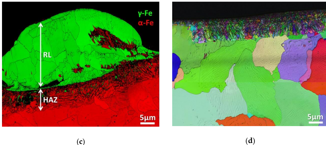
Figure 8. (a) SE image of surface of ECM sample, (b) BF image of FIB lamella cut from ECM surface, (c) EBSD Image Quality Map with overlaid Phase Map of cross section of EDM (roughing) sample, (d) EBSD Image Quality Map with overlaid Inverse Pole Figure Map of pulsed ( \mu s) laser processed cross section.
