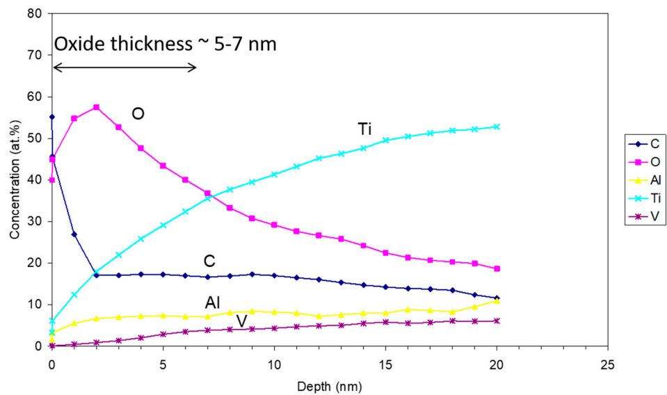
Figure S1: XPS depth profile of as-received Ti-6Al-4V sample.
