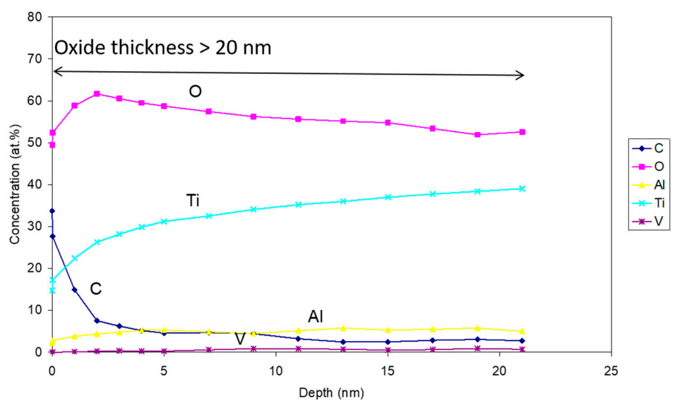
Figure S2: XPS depth profile of laser-textured Ti-6Al-4V sample with \Delta x = 100 \mu\text{m} .
