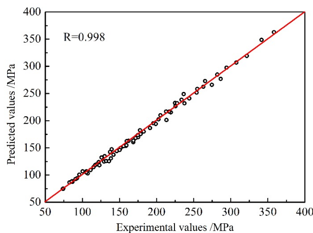
Figure 24. Correlation between predicted values and experimental values.
