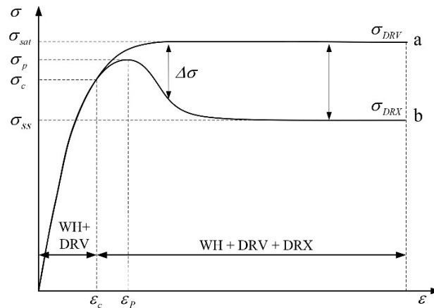
Figure 7. Flow stress–strain curves with different softening mechanisms.
