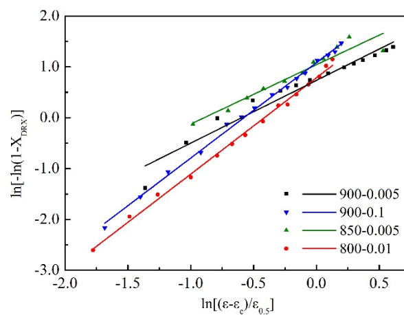
Figure 21. Relationship between \ln[-\ln(1 - X_{DRX})] and \ln[(\varepsilon - \varepsilon_c) / \varepsilon_{0.5}] .
