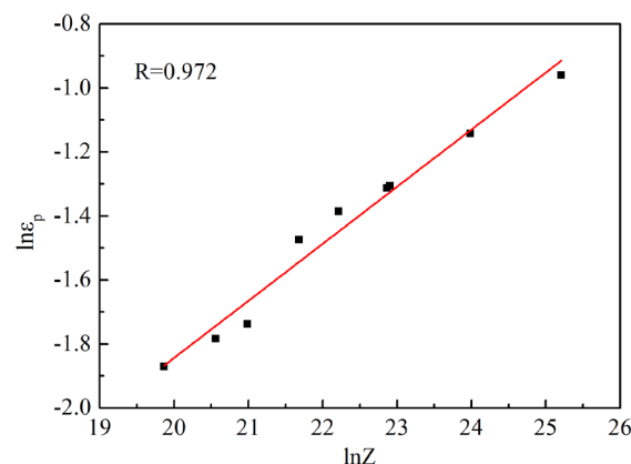
Figure 18. Relationship between \ln \varepsilon_p and \ln Z .
