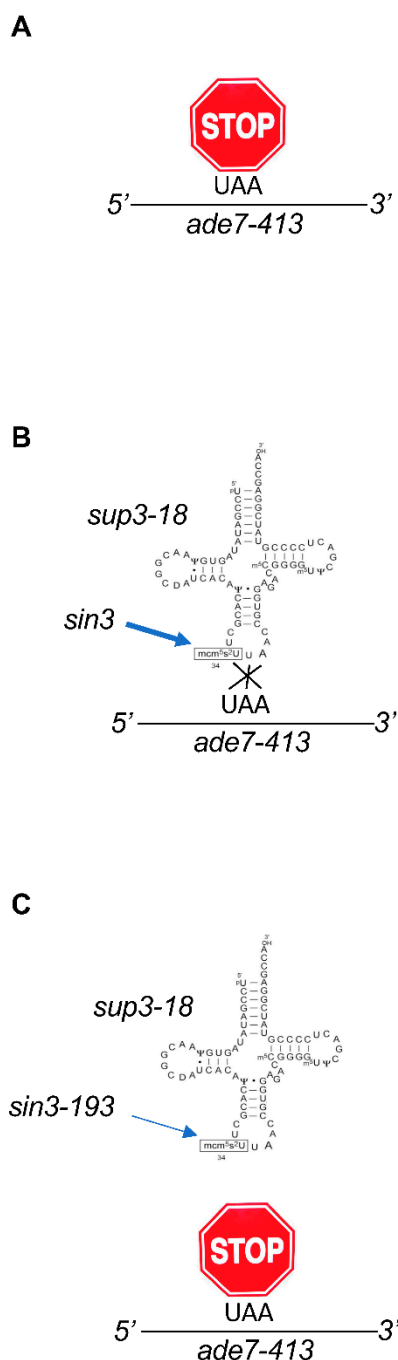
Figure 2. Identification of the antisuppressor sin3-193 mutant as an allele of Elp3 in fission yeast. (A) The ade7-413 allele of the fission yeast ade7 gene contains an ochre STOP codon (UAA). The mutation results in adenine auxotrophy and red color (not shown). (B) The suppressor tRNA sup3-18 contains an anticodon mutation able to read the UAA STOP codon and incorporate a serine, which suppresses adenine auxotrophy and red color (not shown). The sin3 (Elp3) gene product is required for both the anticodon modification ( \text{mcm}^5\text{s}^2 ) and efficient suppression. Note the consistent 5'-3' polarity of the tRNA and mRNA molecules, resulting in the reverse orientation of the codon and the anticodon. (C) The sin3-193 allele of sin3 (Elp3) is a loss-of-function allele and results in anti-suppression. Therefore, despite the presence of the suppressor tRNA, the strain is red and an auxotroph for adenine (not shown), which are easily followed phenotypes.
