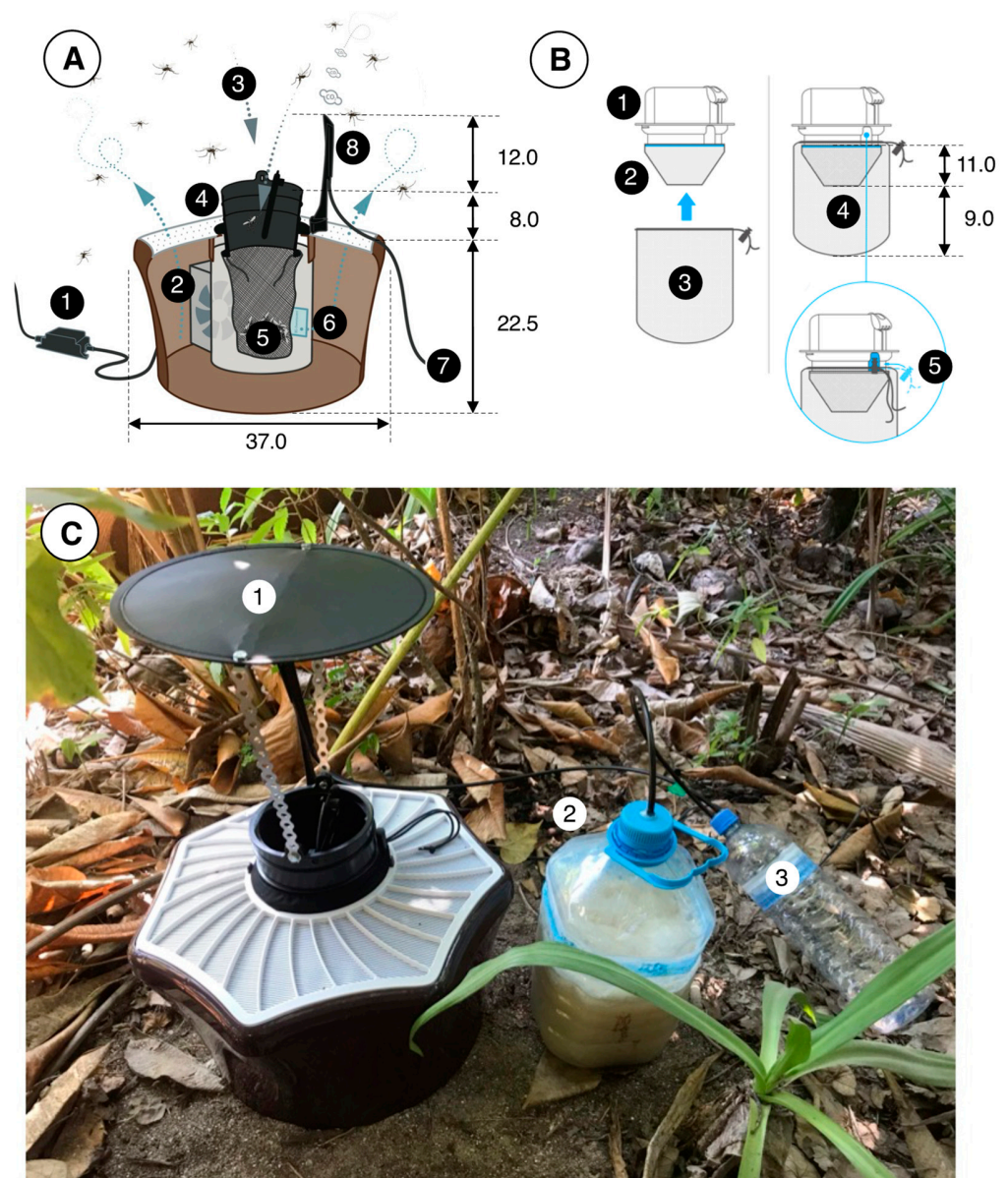
Figure 3. The BG-MosquitaireCO 2 trap and its operation. (A): An adapter (1) converts power from the mains to 12 V DC (0.3 A, 3.6 W), which provides power to a fan (2) located inside the trap. Suction (ca. 3 m/sec) by the fan creates an inward airflow (3) through the black trap inlet (4) and the catch bag (5, see (B)) and odor-laden air (with lactic and hexanoic acid emanating from a sachet) (6) leaves the trap via its perforated white top. Carbon dioxide is provided through 6 mm plastic tubing (7) and released from a nozzle at the top of the trap (8). (B): The inlet (1) of the trap has two netting bags attached to it, a so-called funnel bag (2), which prevents mosquitoes from flying upwards, and the catch bag (3). Both bags (4) are fitted on the inlet (5) using an elastic string. (C): A trap in the field, fitted with a roof (1) to prevent rain from entering the trap. The 5 L water bottle (2) that contains 3 L of water, 700 g of sugar and 20–40 g of yeast to produce CO 2 is located next to the trap. A 1.5 L overflow bottle (3) prevents liquid/foam from this mixture from entering the tubes and nozzle, which might otherwise become clogged and disrupt the flow of CO 2 . Tubes were fitted to the polyethylene bottle tops using hot glue. All dimensions are in cm. Image source: (A,B) Biogents AG, Germany; (C) B.G.J.K.
