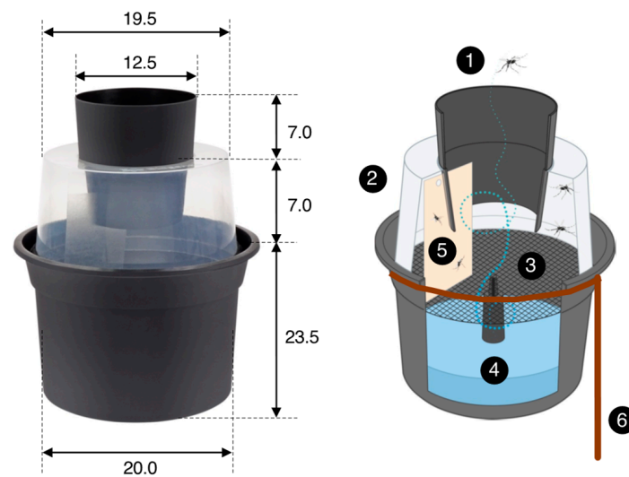
Figure 4. The Gravid Aedes Trap (or BG-GAT trap) is a passive trap that collects mosquitoes ready to lay their eggs. Female mosquitoes enter the trap through a black cone (1) and enter into a translucent chamber (2). A black nylon screen (3) separates the chamber from the oviposition substrate (4) (water with some organic material, e.g., some leaves). Unable to land on the water surface, mosquitoes fly around in the translucent chamber, where they collide with or land on a sticky card (5) (size 8 × 14 cm) on which they become trapped. A rebar wire (diameter 6 mm) ring with a peg (6) was used to position the trap solidly on the ground and prevent it from falling over. All dimensions are in cm. See Eiras et al. [23] for further details; image source: Biogents AG, Germany.
