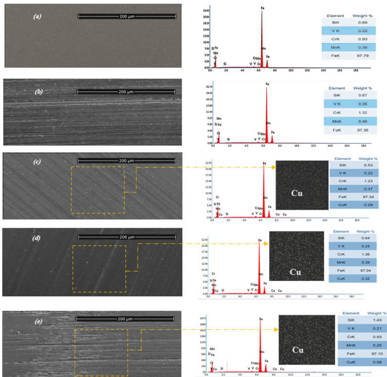
Figure 9. (SEM) micrograph with (EDX) analysis (a) bare sample, (b) Run # 6 (392 N- 0.5 m/s) Base Lubricant, (c) Run # 6 (392 N- 0.5 m/s) 0.2 wt.% CuO, (d) Run # 6 (392 N- 0.5 m/s) 0.5 wt.% CuO, (e) Run # 6 (392 N- 0.5 m/s) 1 wt.% CuO.
