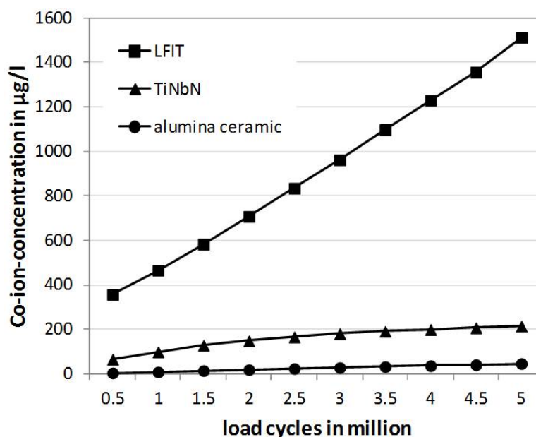
Figure 5. Cumulative cobalt ion concentration over a period of five million cycles analyzed from the used lubricant.
