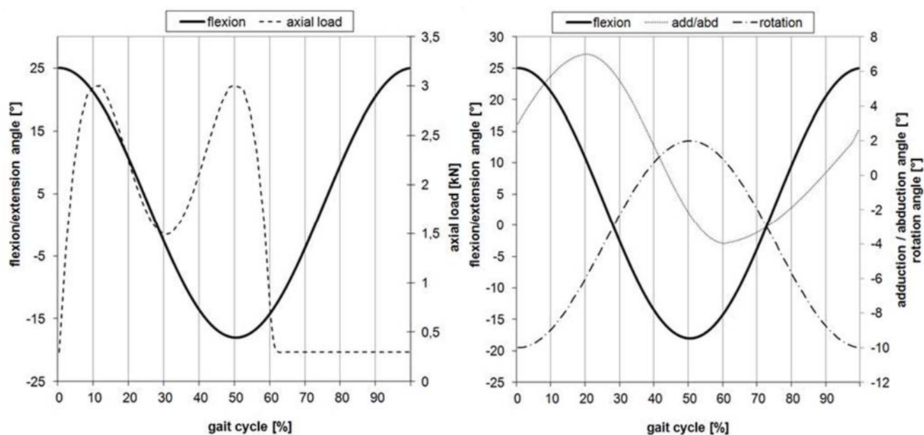
Figure 1. Applied movements throughout the wear simulation as prescribed by the current ISO 14242-1 standard [20].
