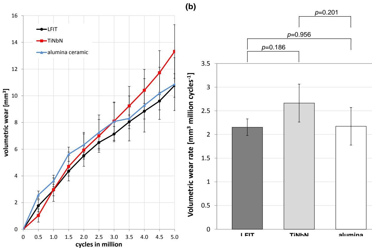
Figure 3. (a) Mean volumetric wear and (b) wear rates of the sequentially cross-linked polyethylene inserts combined with 36 mm diameter femoral heads modified with nitrogen treatment, TiNbN coating, as well as alumina ceramic [19].
