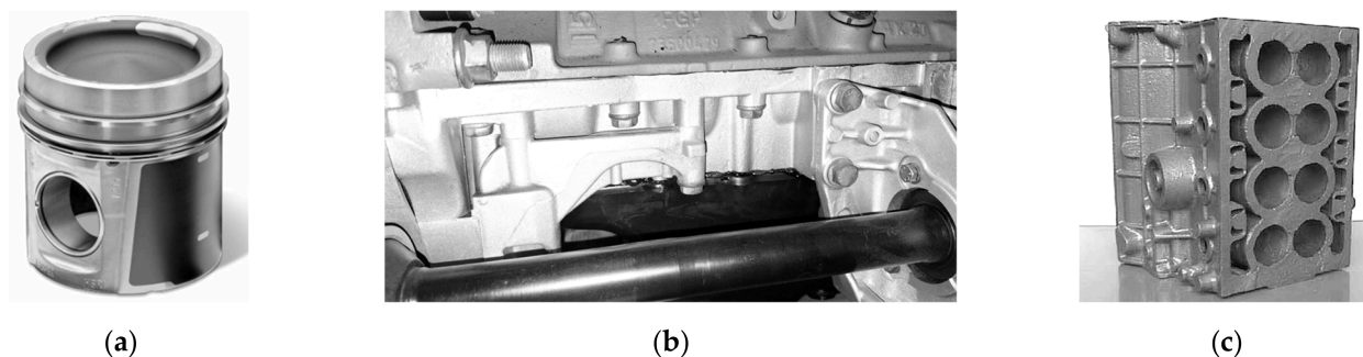
Figure 6. Applications of Eutectic and Hypereutectic Al–Si Alloys: (a) 4032 aluminium alloy piston with a coated piston skirt; (b) upper oil pan made of AlSi12 aluminium alloy; and (c) linerless engine block made from a hypereutectic Al–Si (Alusil-type) alloy for a VCR engine prototype.
