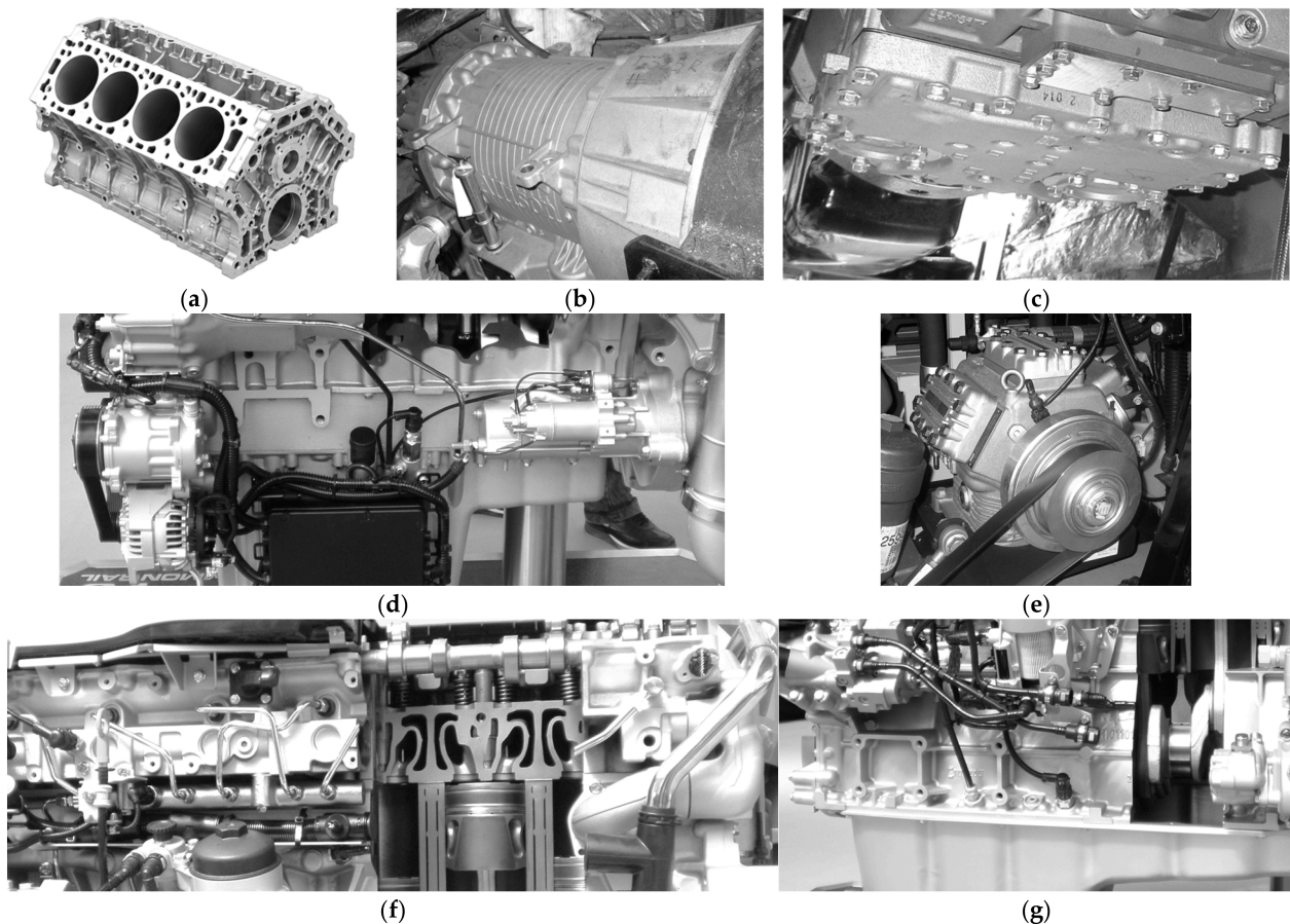
Figure 5. Photographs of Automotive Applications of Hypoeutectic Al-Si Alloys: (a) 3D model and cross-sectional view of a closed-deck V8 engine block made of A319 aluminium alloy; (b) A356 aluminium alloy housing of a six-speed automatic gearbox used in a city bus; (c) ADC12 aluminium alloy hydraulic valve body housing with internal channels and separator plate for an automatic gearbox; (d) A380 aluminium alloy alternator and starter motor housings mounted on a truck engine; (e) A356 aluminium alloy cylinder block of a reciprocating A/C compressor used in a city bus; (f) cross-section of the A356/A357 aluminium alloy cylinder head and cylinder of a six-cylinder truck engine; and (g) A380 aluminum alloy oil pan of a truck engine.
