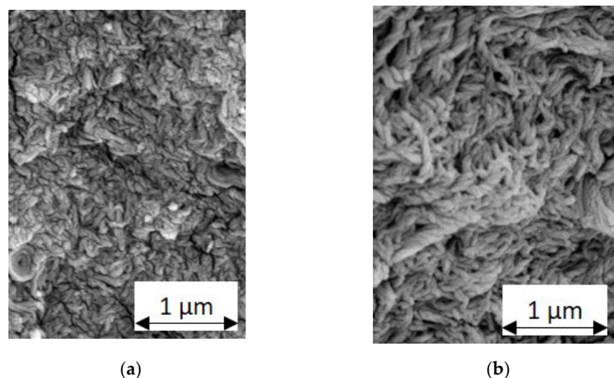
Figure 4. SEM images of the greases with 15 wt % lithium 12-hydroxystearate as thickener and mineral oil as base oil: (a) base oil viscosity \eta_{MO} = 0.12 Pas; (b) base oil viscosity \eta_{MO2} = 2 Pas.
