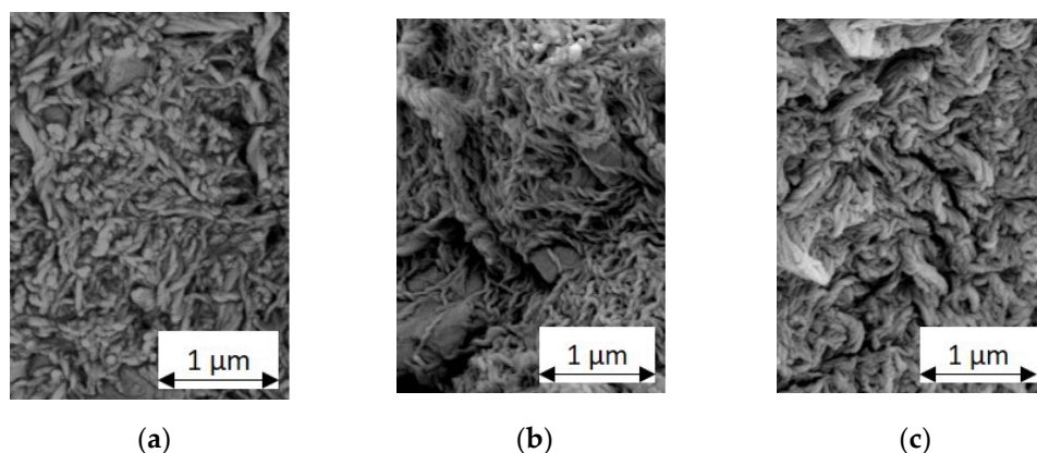
Figure 6. SEM images of the greases with mineral oil as base oil and lithium 12-hydroxystearate as thickener at different concentrations: (a) 11 wt %; (b) 13 wt %; and (c) 15 wt %.
