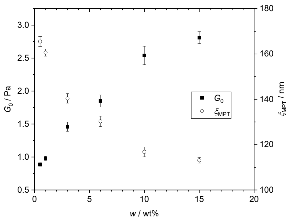
Figure 11. Concentration series with paraffinic mineral oil as base oil and lithium 12-hydroxystearate as thickener. Shear modulus G_0 and mesh size as functions of concentration as obtained from MPT measurements.
