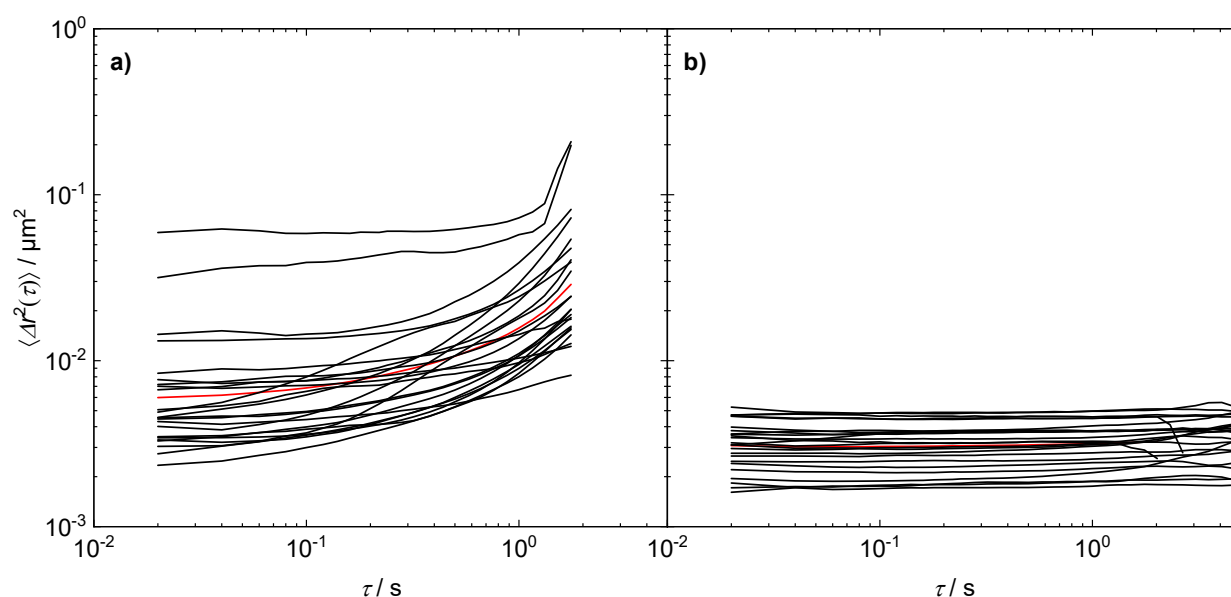
Figure A2. MSDs of two MPT single measurements of the grease with 0.5 wt % lithium 12-hydroxystearate as thickener and MO as base oil: (a) single measurement in which the tracers ( N = 23 ) diffuse freely in the oil and the MSDs are correspondingly time-dependent; (b) single measurement in which the tracers ( N = 24 ) are trapped in a network and the MSDs are correspondingly time-independent.
