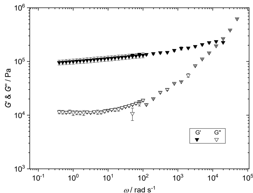
Figure A1. Moduli G' and G'' of the grease with 15 wt % lithium 12-hydroxystearate and MO2 as base oil.
