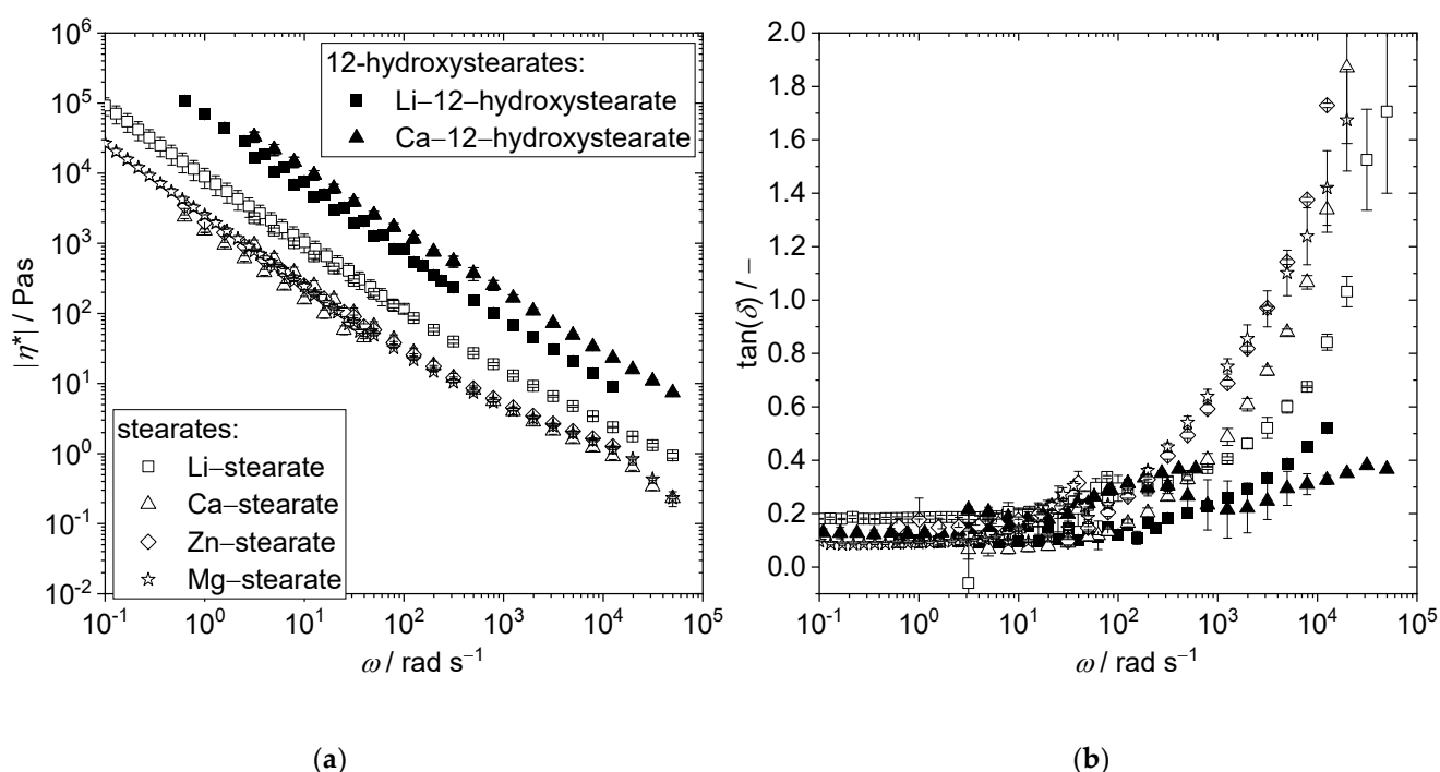
Figure 7. Influence of thickener type on rheological grease properties. (a) Absolute value of complex viscosity |\eta^*| as a function of the angular frequency \omega of lubricating greases made from mineral oil
