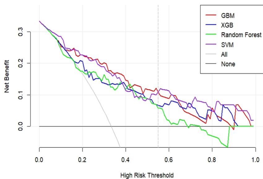
(b) Decision curves
