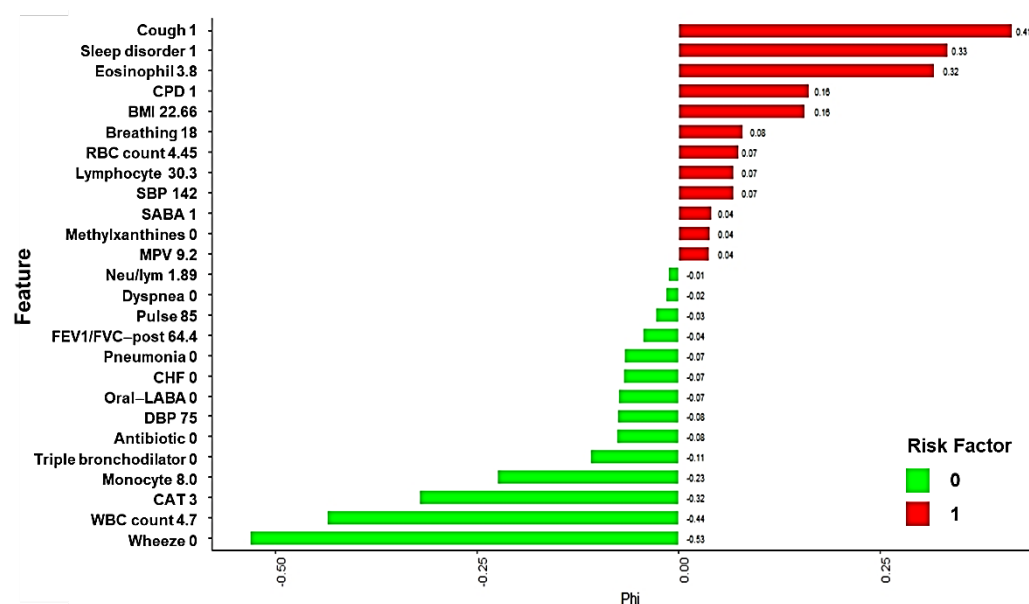
(c) AECOPD but AI predicted non-AECOPD ( P_{\text{AECOPD}} = 0.173 )
