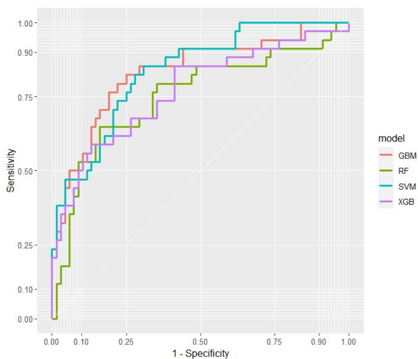
(a) ROC curve
