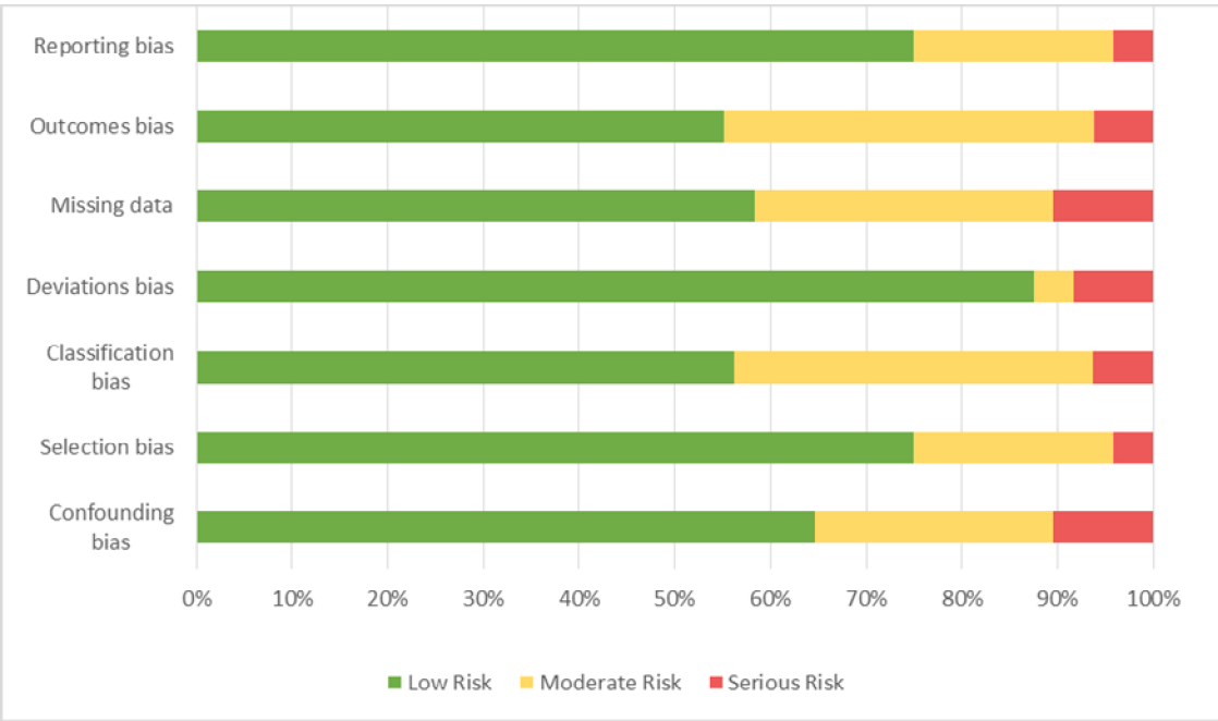
Supplementary Figure 2: Quality scores for the risk of bias using the ROBINS tool.
