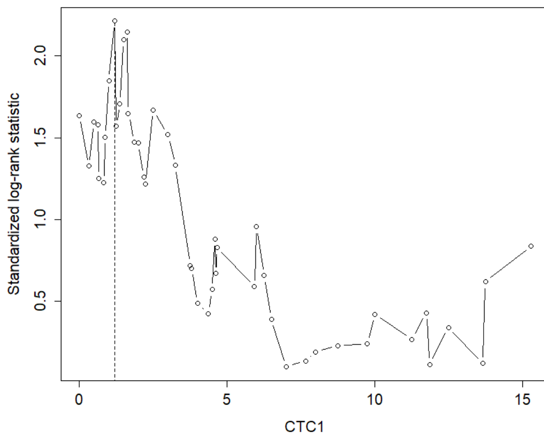
Supplementary Figure S1. Lausen and Schumacher method to determine the best cut-off point for CTC1
