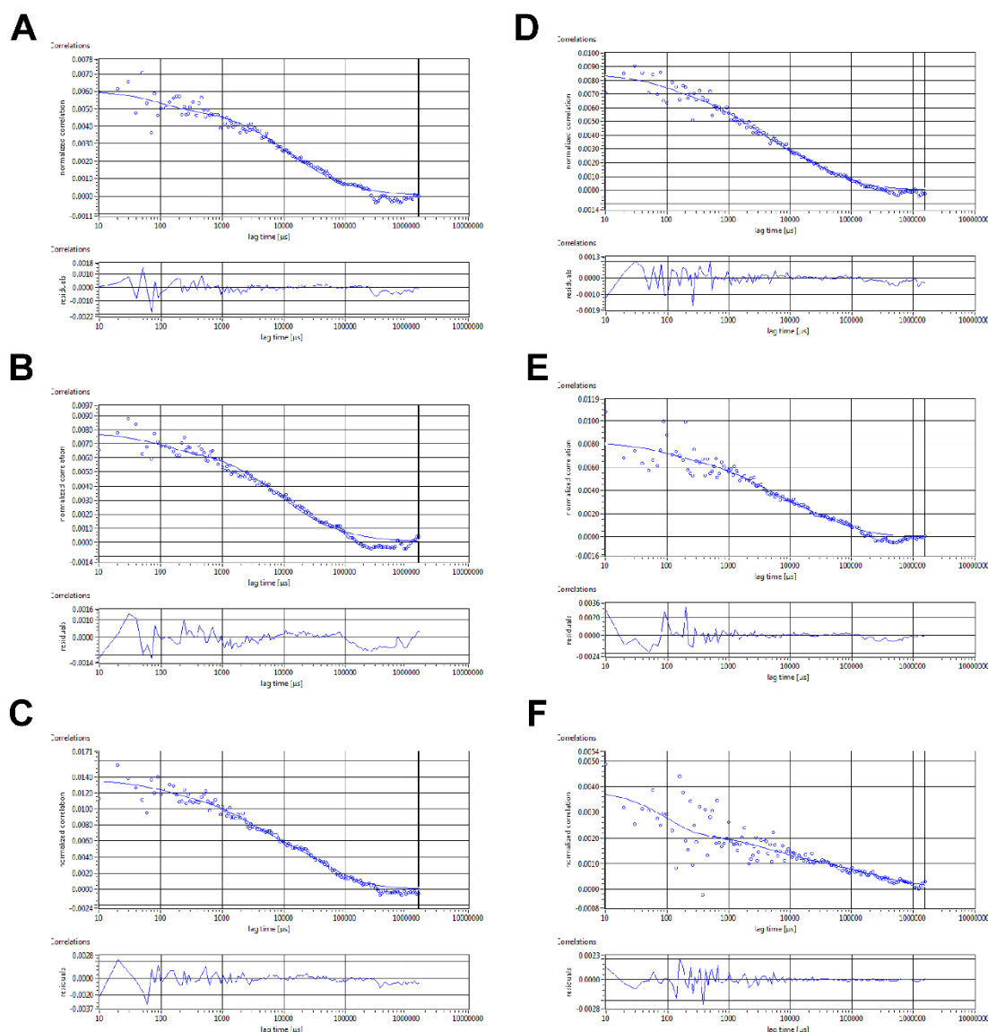
Supplemental Figure 1. Several examples of normalized autocorrelation functions of PetC1-GFP protein in several cells of Synechocystis . Points represent experimental data of calculated autocorrelation functions, lines show fit by 2D model of diffusion for PetC1-GFP. Residual values from the fit are shown below the main figures.
