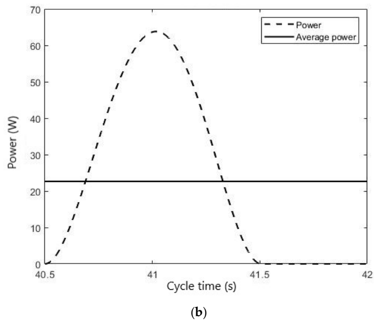
Figure 16. Wheelchair speed (a) and user's power (b) in a complete cycle during the steady-state phase.
