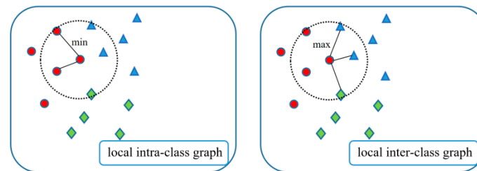
Figure 1. Example of local graph construction, where k = 5 and different shapes represent different classes of samples.
