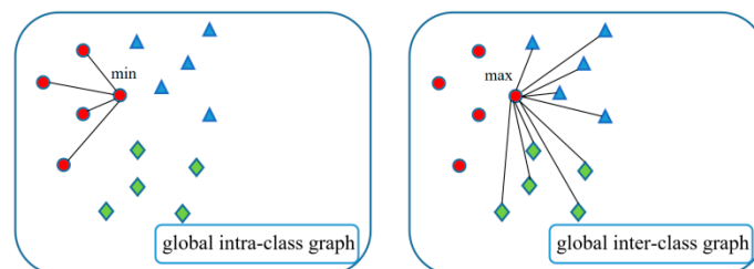
Figure 2. Example of global graph construction.
