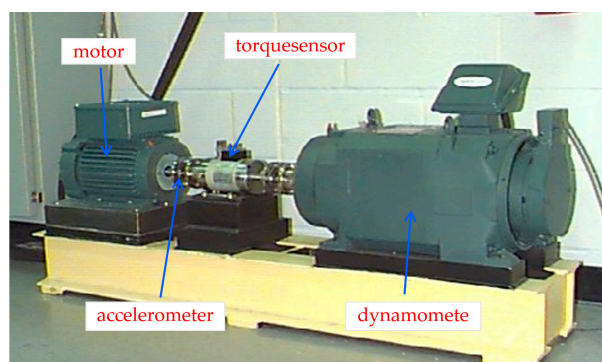
Figure 4. Bearing test platform.
