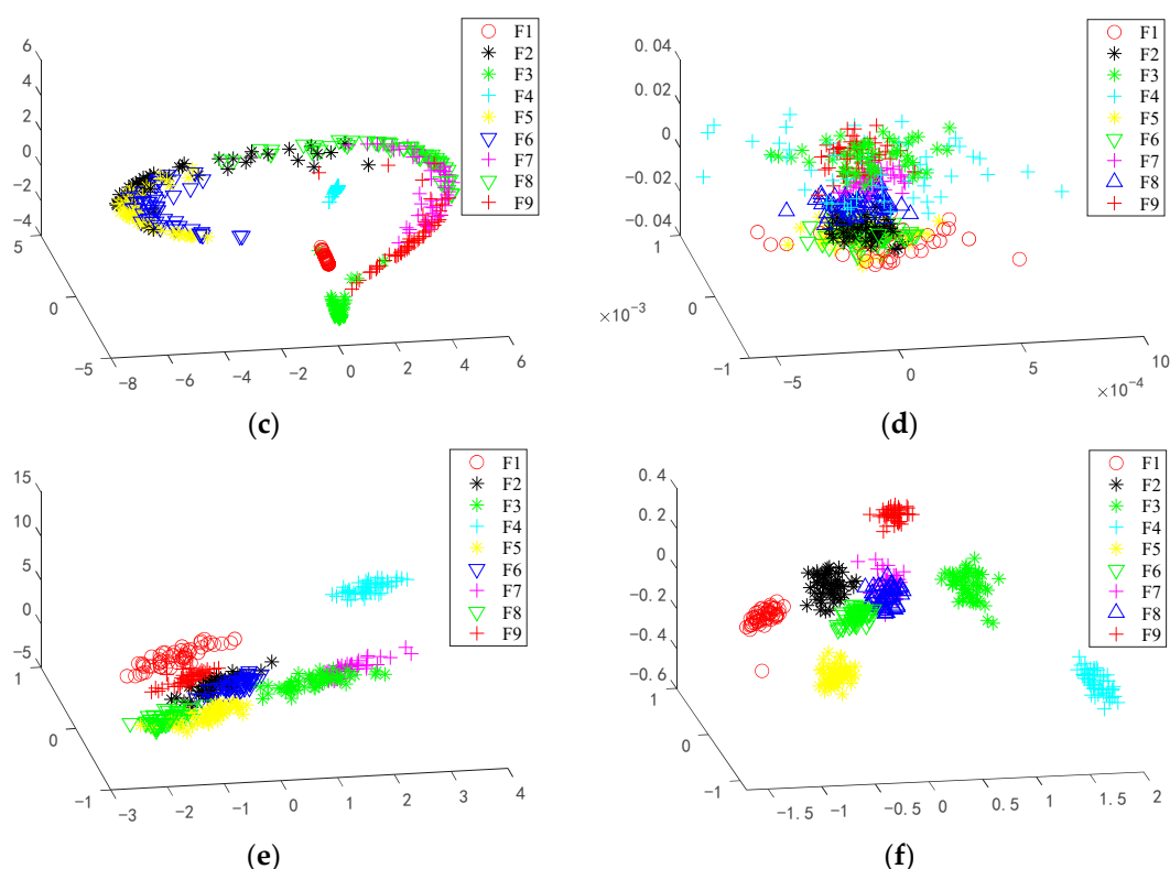
Figure 13. Three-dimensional distribution of test gear samples: (a) LLE; (b) LPP; (c) KPCA; (d) OLGPP; (e) LSPD; (f) ESB DP.
