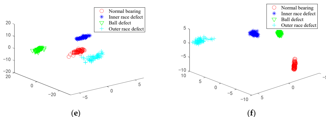
Figure 6. Three-dimensional distribution of test bearing samples: (a) LLE; (b) LPP; (c) KPCA; (d) OLGPP; (e) LSPD; (f) ESBP.
