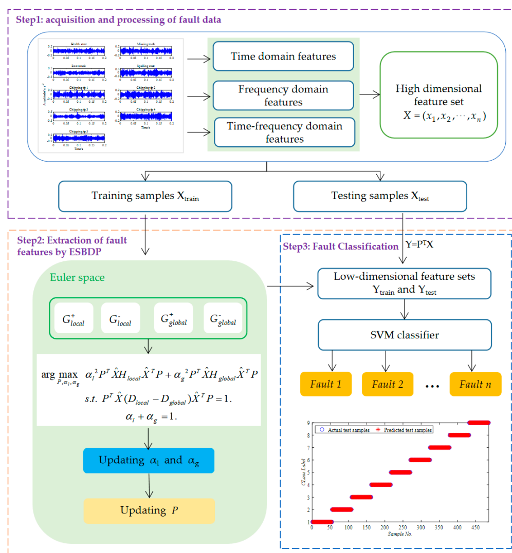
Figure 3. Procedure of fault diagnosis based on ESBDP.
