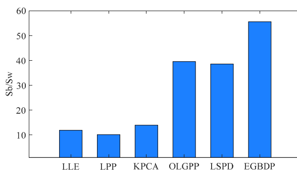
Figure 7. Low-dimensional feature separability index based on different algorithms.
