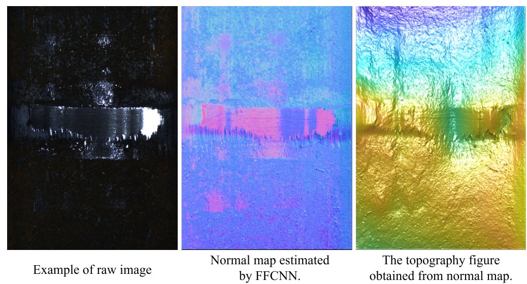
Figure 10. The normal map of upper surface of the rail estimated by FFCNN and the corresponding topographic map. The color of the topographic map represents the height of the surface.
