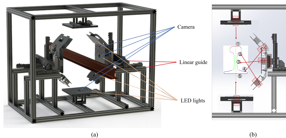
Figure 9. Illustration of the equipment. (a) Overall illustration of the equipment. It mainly contains four information acquisition systems (IASa, IASb, IASc, IASd) and two linear guides and profiles. (b) Each camera corresponds to a range of shots.
