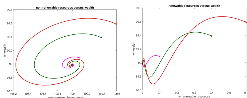
Figure 1. Case 3. Phase diagram related to the analysis of the stable point P_2 . (left): non-renewable resources versus wealth. (right): renewable resources versus wealth.
