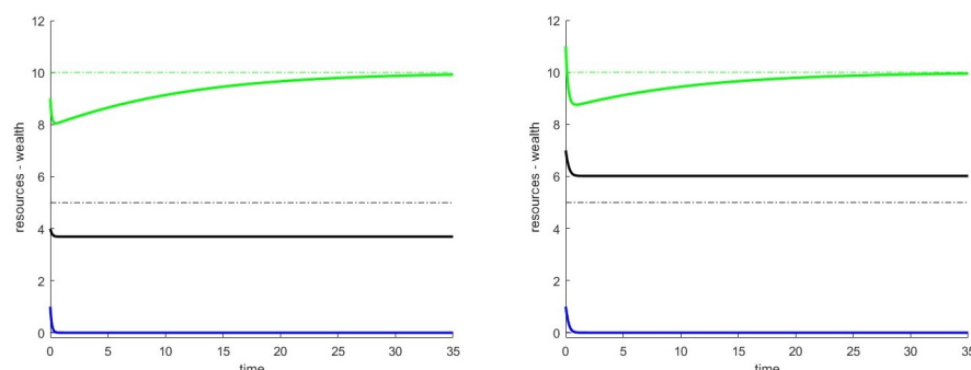
Figure 2. Case 4. The variable z stabilizes at a value different from the critical one. (left): negative perturbations on y(t) and z(t) . (right): all initial perturbations are positive.
