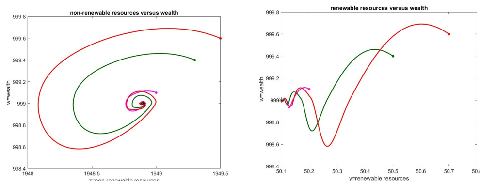
Figure 3. Case 6. Phase diagram related to the analysis of the stable point P_2 . (left): non-renewable resources versus wealth. (right): renewable resources versus wealth.
