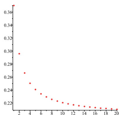
Figure 5. Value of the probability \pi_2 of saturation when R has the gamma distribution defined in Equation (58), for \alpha = 1, 2, \dots, 20 .
