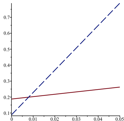
Figure 4. E[J_2(2)] for q_0 \in [0, 0.05] when s = 3 , \lambda = 1 , \mu = 1 (solid line), and \mu = 2 (dotted line).
