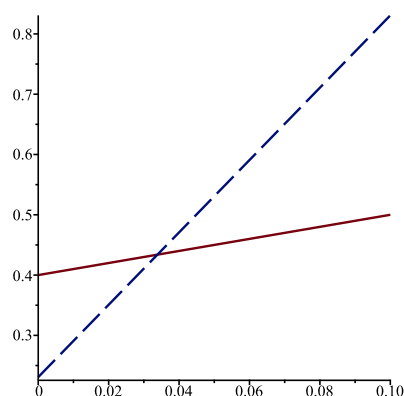
Figure 2. E[J_2(1)] for q_0 \in [0, 0.1] when s = 2 , \lambda = 1 , \mu = 1 (solid line), and \mu = 2 (dotted line).
