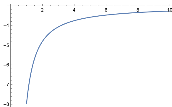
Figure 1. Value function F(0) for q_0 \in [0, 10] when s = 3 ; \theta = -1 ; and \lambda = 1 .
