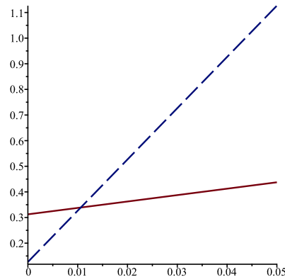
Figure 3. E[J_2(1)] for q_0 \in [0, 0.05] when s = 3 , \lambda = 1 , \mu = 1 (solid line), and \mu = 2 (dotted line).
