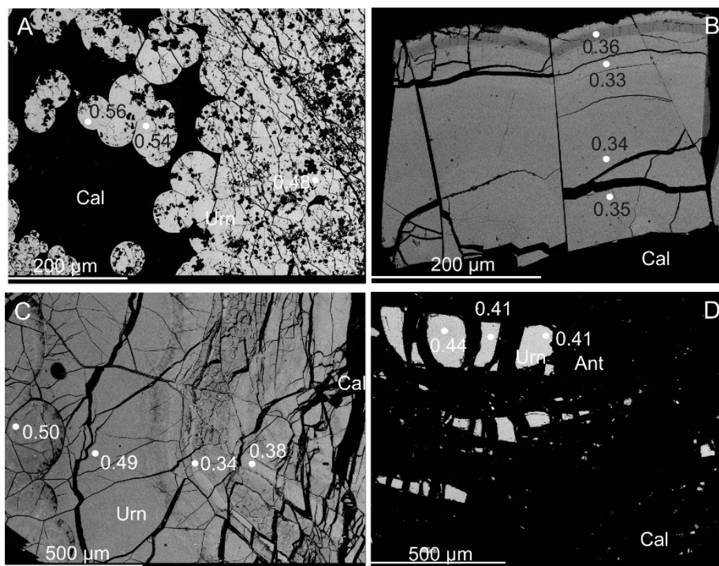
Figure 6. Back-scattered electron (BSE) images of uranium mineralization with distribution of Ca ( apfu , O = 4) in uraninite. Příbram uranium district. Urn—uraninite, Cal—calcite, Ant—anthraxolite.
