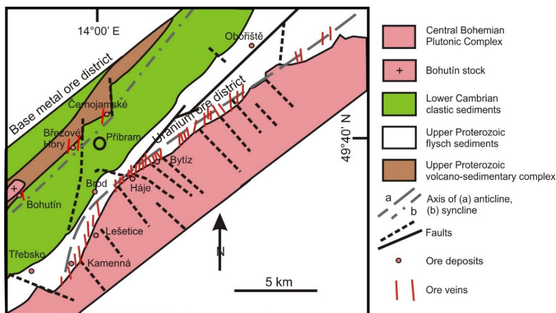
Figure 2. Schematic geological map of the Příbram base metal and uranium ore districts (modified from Kříbek et al. [17]).
