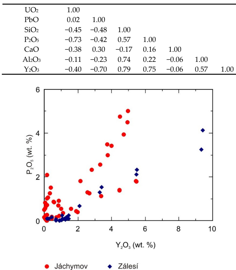
Figure 14. Distribution of P and Y in coffinite from the Jáchymov uranium district and the Zálesí uranium deposit.
