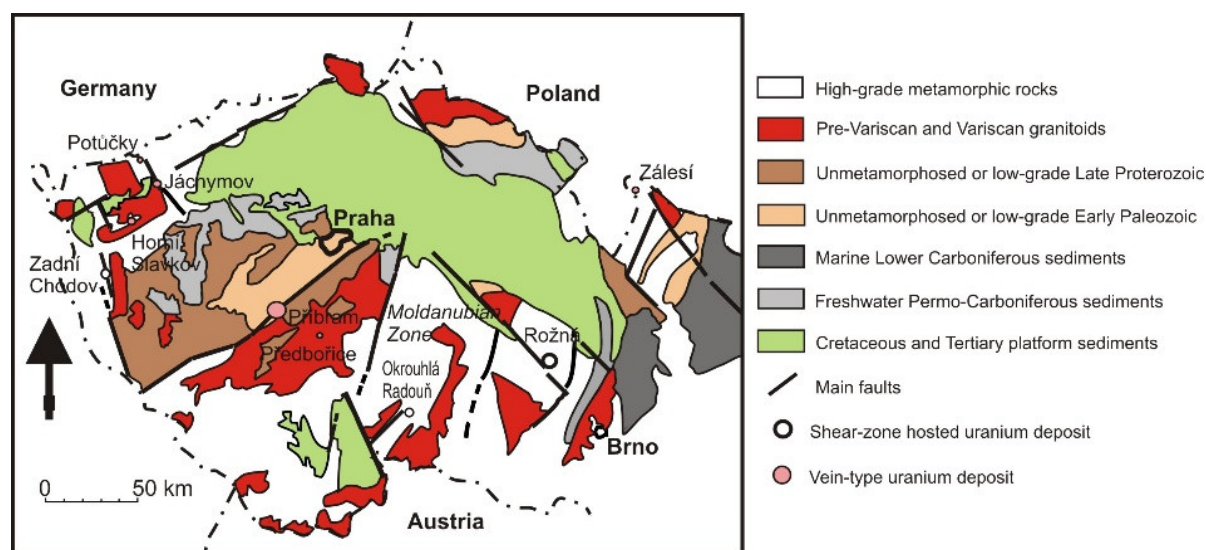
Figure 1. Simplified geological map of the Bohemian Massif showing the position of the most significant Czech basement-hosted uranium deposits.
