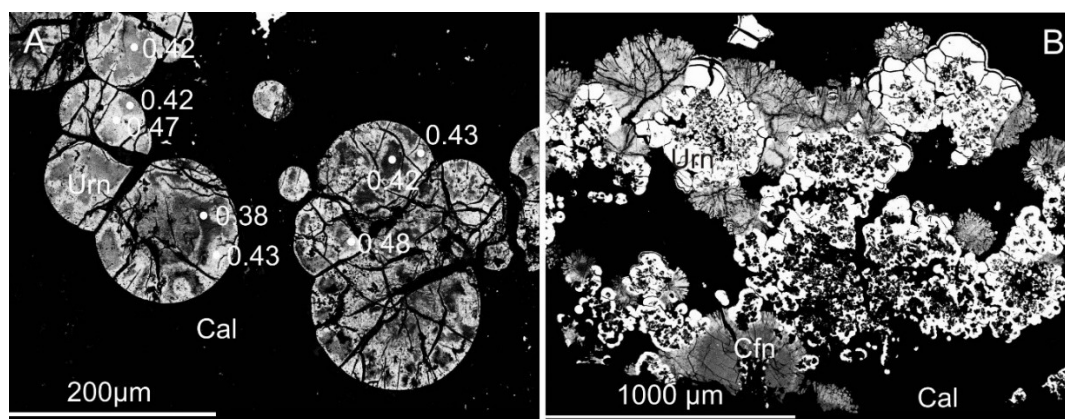
Figure 8. BSE images of uranium mineralization with distribution of Ca ( apfu , O = 4) in uraninite, Zálesí uranium deposit. Urn—uraninite, Cfn—coffinite, Cal—calcite.
