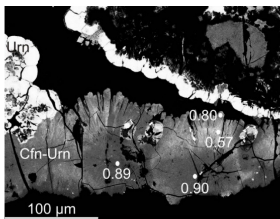
Figure 11. BSE image of coffinitized uraninite with distribution of Si ( apfu , O = 4), Zálesí uranium deposit. Urn—uraninite, Cfn-Urn—coffinitized uraninite.
