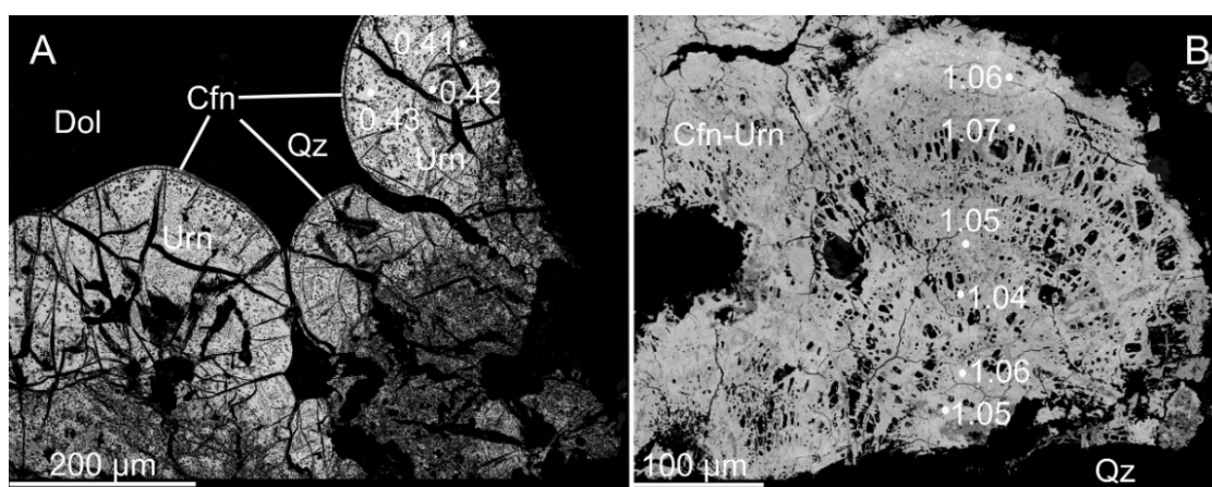
Figure 10. BSE images of coffinite and coffinitized uraninite with distribution of Si ( apfu , O = 4), Jáchymov uranium district. Urn—uraninite, Cfn—coffinite, Cfn-Urn—coffinitized uraninite, Dol—dolomite, Qz—quartz.
