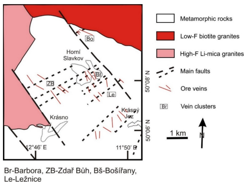
Figure 4. Schematic geological map of the Horní Slavkov uranium district (modified from Komínek et al. [24]).
