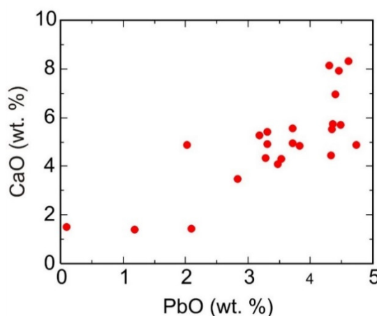
Figure 13. Distribution of Ca and Pb in uraninite from the Horní Slavkov uranium district.
