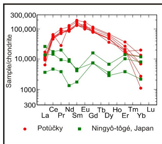
Figure 15. Chondrite-normalised rare earth element patterns for ningyoite from the Potůčky and Ningyô-tôgé uranium deposits. Chondrite values are from Anders and Grevesse [68], data for Ningyô-tôgé deposit are from Muto [67].
