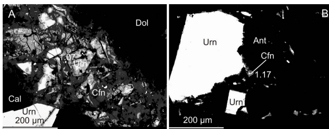
Figure 9. BSE images of uranium mineralization with distribution of Si ( apfu , O = 4) in coffinite, Příbram uranium district. Urn—uraninite, Cfn—coffinite, Ant—anthraxolite, Cal—calcite, Dol—dolomite.
