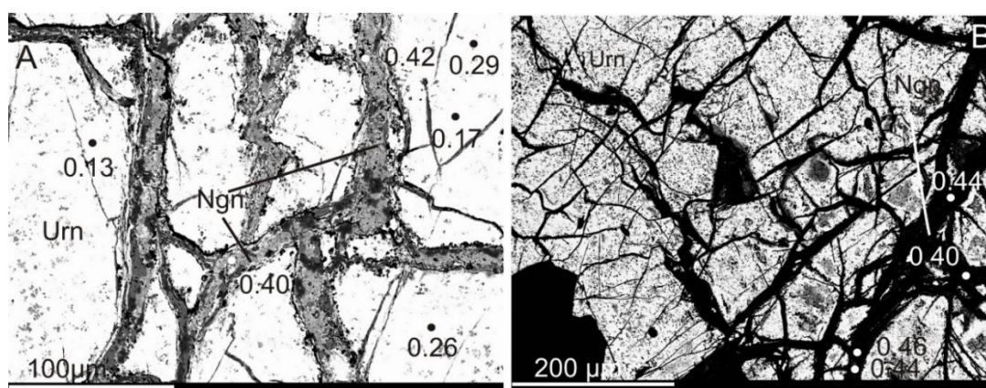
Figure 12. BSE images of uranium mineralization with distribution of Ca ( apfu , O = 4) in ningyoite and uraninite, Potůčky uranium deposit. Urn—uraninite, Ngn—ningyoite.
