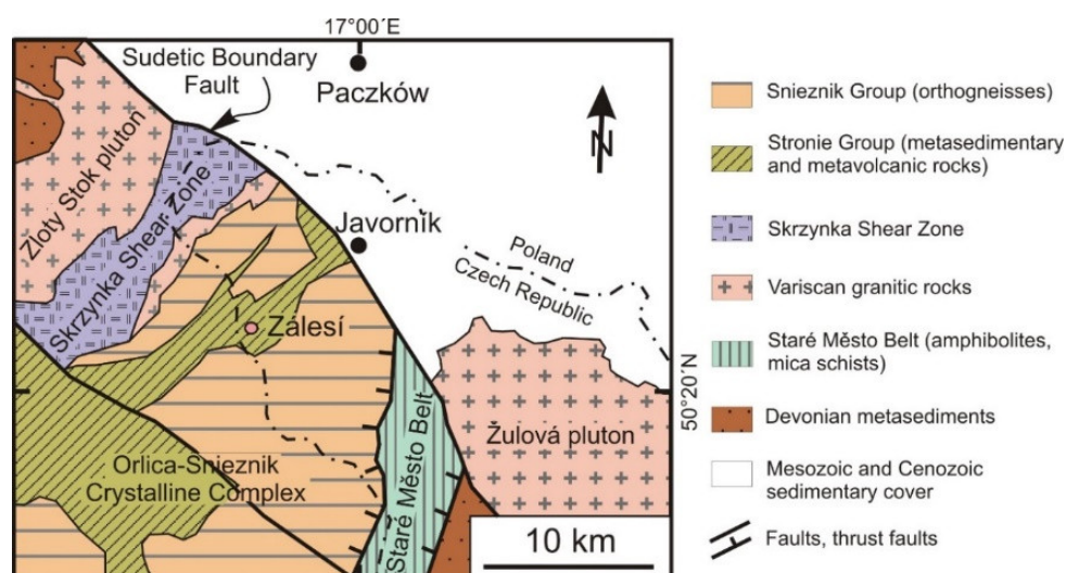
Figure 5. Geological position of the Zálesí uranium deposit (modified from Dolníček et al. [32]).
