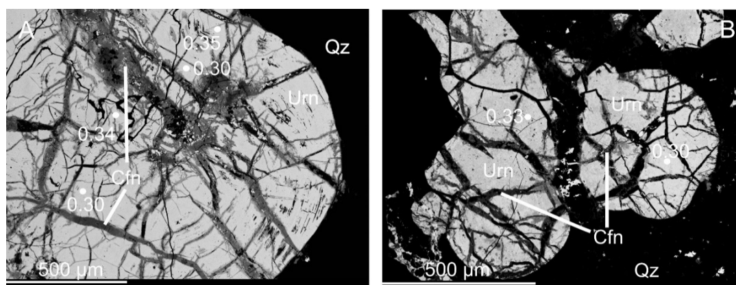
Figure 7. BSE images of uranium mineralization from the Jáchymov uranium district with distribution of Ca ( apfu , O = 4). Urn—uraninite, Cfn—coffinite, Qz—quartz.
