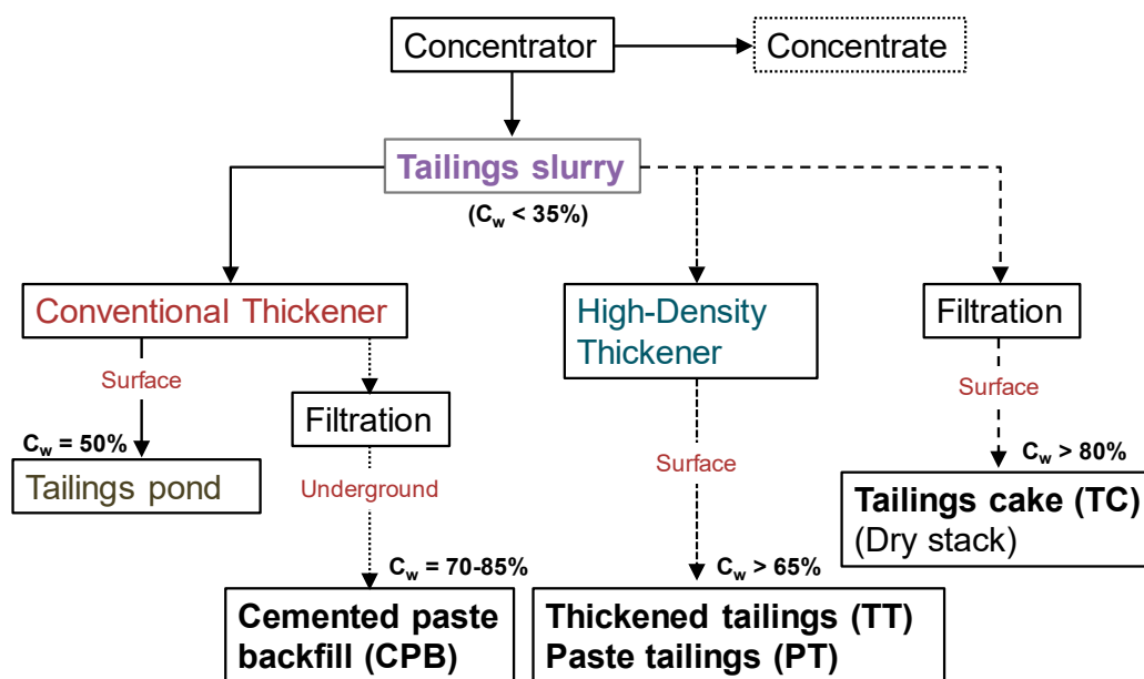
Figure 1. General scheme of conventional methods of the tailings management.
