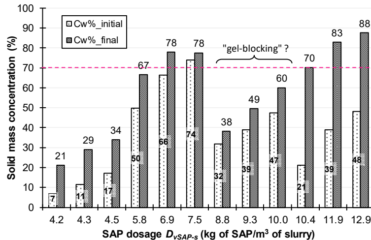
Figure 13. Results of tailings slurry dewatering using D_{vSAP-s} in the range 4.2–12.9 kg/m³ of grade 1 SAP and after 72 h residence time.
