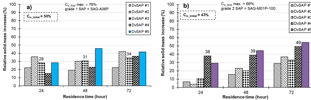
Figure 17. Tailings slurry relative solids mass concentration increase regarding the residence time and five SAP dosages: (a) grade 1 SAP (SAG-A06P), (b) grade 2 SAP (SAG-M01P-100).
