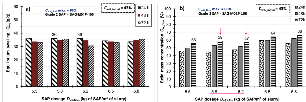
Figure 12. Tailings slurry at C_{w\%\_initial} = 43\% dewatered at different dosages of grade 2 SAP (SAG-M01P-100): (a) equilibrium swelling Q_{eq} for three different residence times, (b) final solids concentration C_{w\%\_final} .
