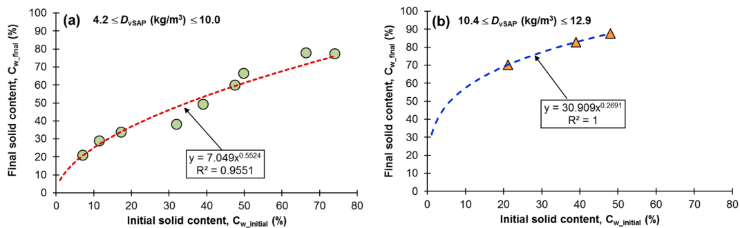
Figure 18. Power law empirical correlations between C_{w\%\_initial} and C_{w\%\_final} using grade 1 SAP (SAG-A06P): (a) for D_{vSAP} in the range 4.2–10 kg of SAP/ \text{m}^3 of slurry, (b) for D_{vSAP} in the range 10.4–12.9 kg of SAP/ \text{m}^3 of slurry.
