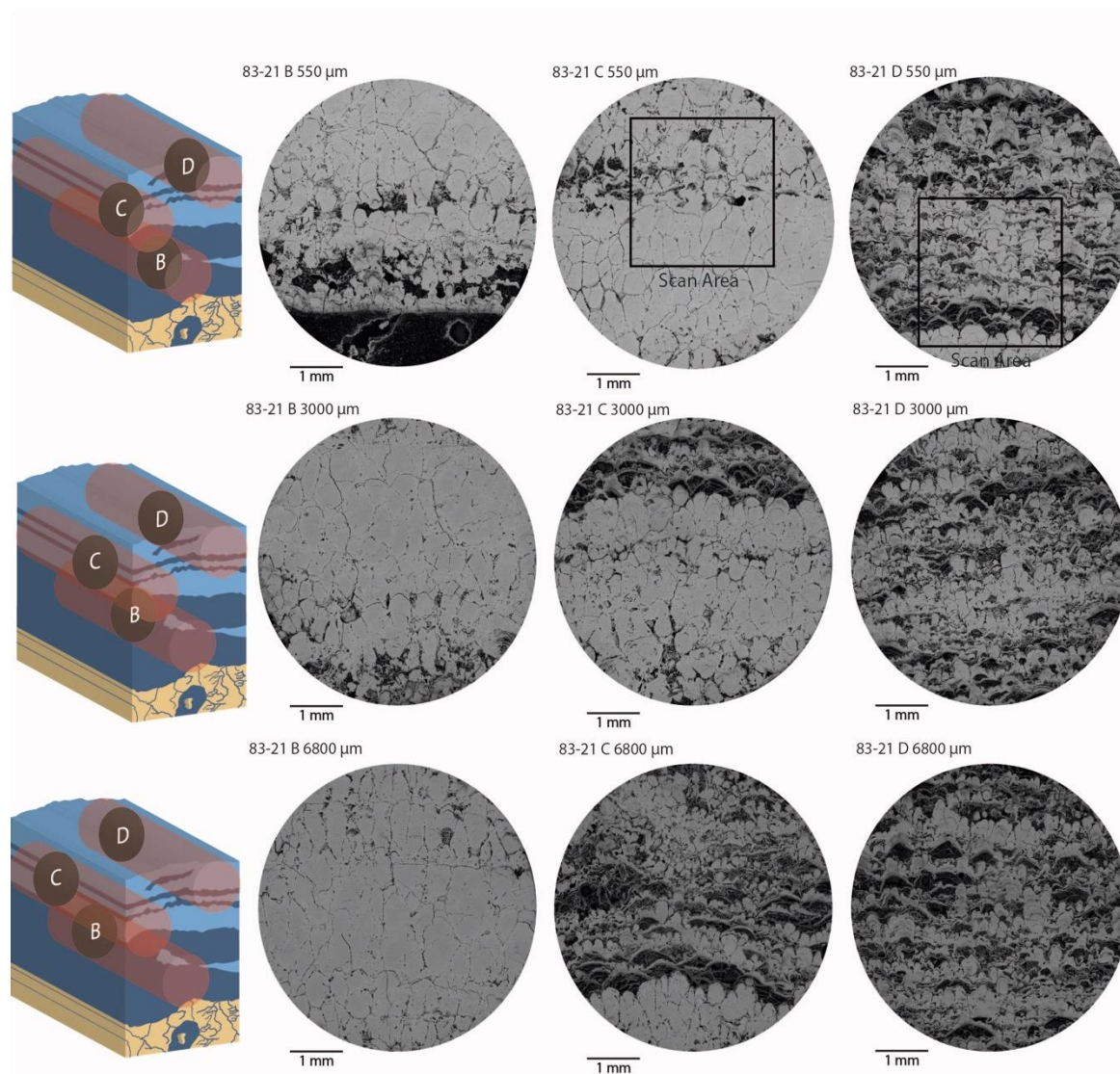
Figure 4. Cross sections through all cores 83-21 B, C, and D made using the SEM. All cores are 4 mm across. The black squares on 83-21 C and 83-21 D show the areas used to measure bulk composition using SEM energy dispersive X-ray spectroscopy (SEM-EDS). Again, good examples of pillared and cusplate textures are visible, as well as erosional (83-21 B 3000 \mu\text{m} ) and gradational (83-21 C 6800 \mu\text{m} ) contacts between them. The block diagrams show their position relative to the sample and each other.
