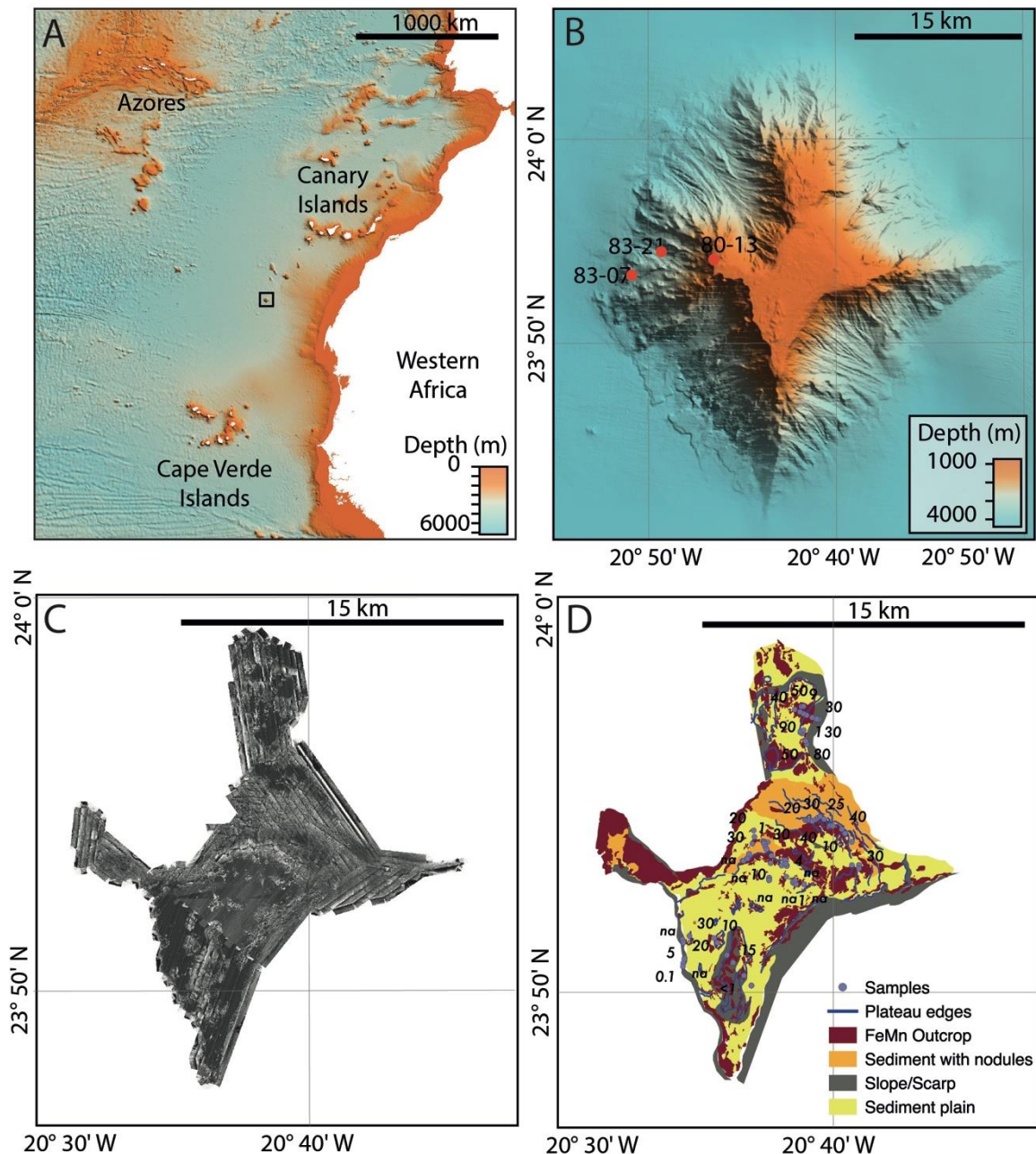
Figure 1. (A) Regional setting. Bathymetry data is taken from GEBCO [27]. The black square shows the location of panel B; (B) EM120 data collected off Tropic Seamount, gridded at 50 m, overlaid on the GEBCO background. The three sample locations are shown with red dots; (C) autonomous underwater vehicle (AUV) side-scan sonar data collected by the AutoSUB6000. Pixel size is 2 m, bright colors represent areas of high backscatter; (D) Simplified geological map of the summit from side-scan sonar, bathymetry, and remotely operated vehicle (ROV) groundtruthing. The numbers represent crustal thicknesses measured on samples collected during the ROV dives in mm. na is given where there was no FeMn material on the sample. The FeMn crustal outcrop is mapped in maroon. Nodules were generally sparse in the areas where they were found and are not included in the calculations. The map was produced using QGIS 3 [28].
