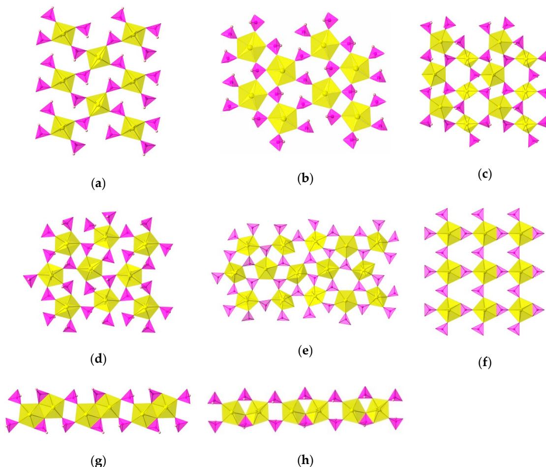
Figure 3. The eight different uranyl phosphite structure types are shown. The letter label corresponds with the “Structure Type” shown in Table 6. Labels (a)–(f) are all sheet topologies, whereas (g) and (h) are chains. (Please note images (c)–(h) are adapted from their original publication. (c) and (d) adapted with permission from Villa et al. [16]. (e) adapted with permission from Villa et al. [18]. (f)–(h) adapted from Villa et al. [56].
