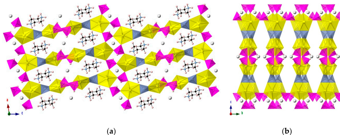
Figure 4. [(\text{H}_2\text{PZ})\text{Cs}][(\text{UO}_2)_2(\text{HPO}_3)_2(\text{PO}_4)] (2): (a) The 3D framework structure of (2) is shown in the ac -plane, where the oblong channels can be observed; (b) These channels are fairly narrow when viewed in the bc -plane (the piperazinium cations are omitted for clarity). Color scheme is the same as in Figure 1, save the cesium cations shown in light grey and the phosphate anions shown in blue-grey.
