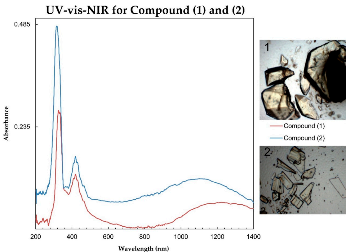
Figure A1. UV-vis-NIR spectra for both Compound (1) and (2) showing the characteristic peaks for U(VI) between 370–500 nm. Inset photos show the crystalline phases obtained for both compounds. The top photo is of compound (1) and the bottom photo is of compound (2).
