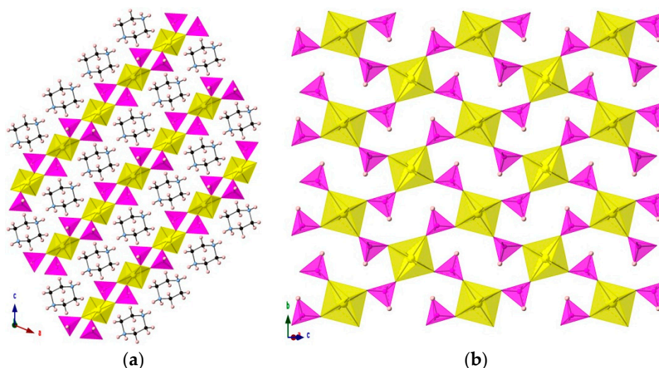
Figure 1. [\text{H}_2\text{PZ}][\text{UO}_2(\text{HPO}_3)_2] (1): (a) A view of (1) in the ac -plane shows the layers of uranyl phosphite charged balanced by the piperazinium dication; (b) The sheet topology of (1) is shown slightly askew in the [1\ 0\ -1] with each square bipyramid of U(VI) corner sharing to a phosphite ligand through the equatorial oxygen atoms. Here the uranium polyhedra are yellow, phosphites are purple, hydrogen atoms are off-white, carbon atoms are black, and nitrogen atoms are light blue; oxygen atoms are omitted for clarity.
