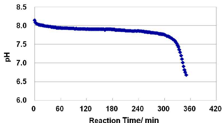
Figure 1. The change in pH of the slurry during the carbonation of \text{Ca(OH)}_2 at 70 °C with the approximate flow rate of 900 mL/min of \text{CO}_2 (30%)-clean air (70%) mixed gas for 100 g of \text{Ca(OH)}_2 , as the function of reaction time.
