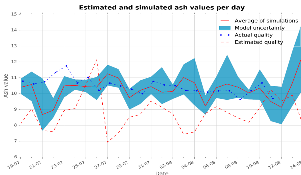
Figure 16. Daily ash values per day, case Profen.
