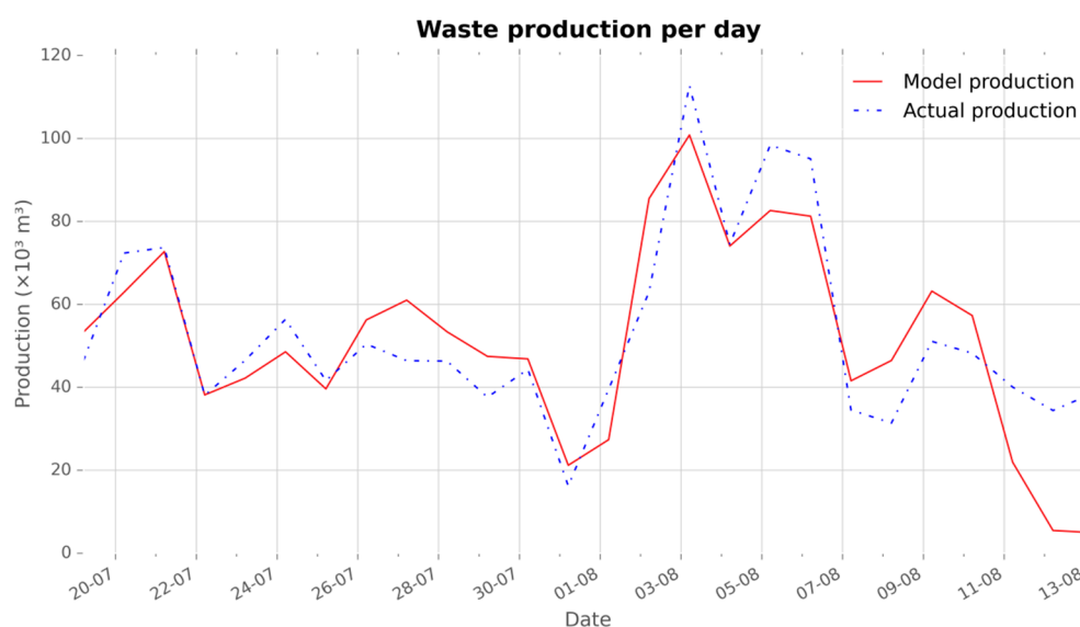
Figure 13. Comparison of daily production of waste, Experiment 1.
