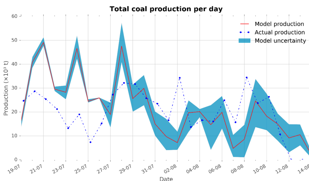
Figure 17. Comparison of daily production of coal, Experiment 3.
