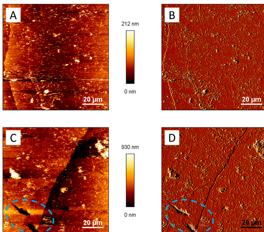
Figure S1. AFM images of pyrite surface. (A,B) are the height and vertical deflection images of clean pyrite surface, respectively; (C,D) are the representative height and vertical deflection images of pyrite surface after abiotic leaching for 10 months, respectively. Circles in (C,D) indicate etch pitches.
