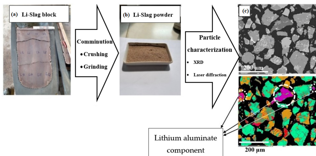
Figure 3. Slag's transformation from (a) solid block to (b) powder form and (c) mineral characterization using an electron probe micro-analyzer (EPMA).
