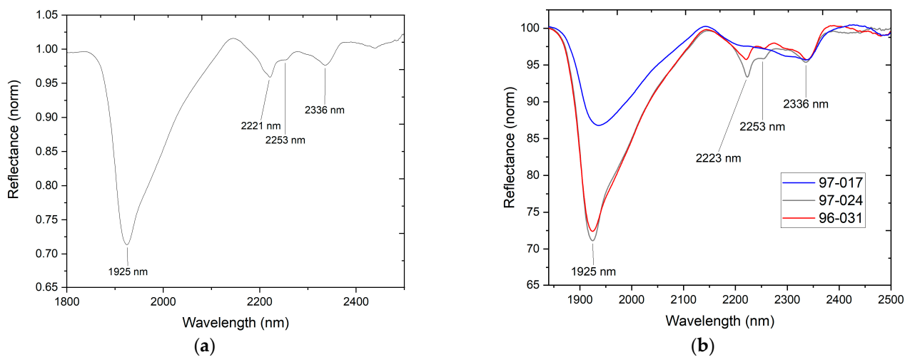
Figure 15. (a) Representative SWIR spectra from the blue pigment on object 96-015 and (b) representative objects for the green pigments. Features associated with \text{CaCO}_3 and clays are indicated.
