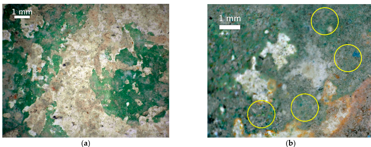
Figure 18. (a) Uniform green layer over stucco at 40× corresponding to green 1, and (b) green region with yellow pigment layer and blue particles (position indicated with yellow circles) at 50×, corresponding to green 2.
