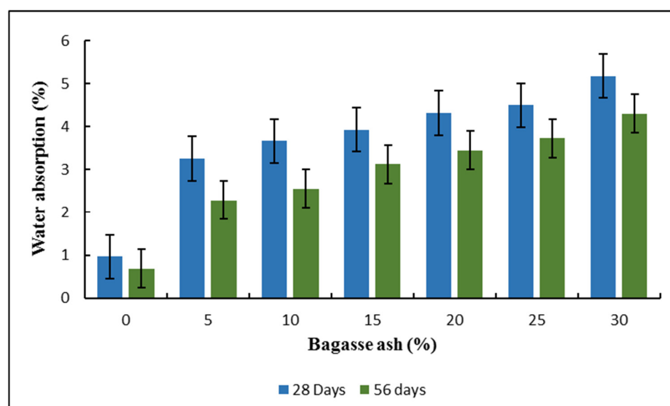
Figure 13. Water absorption of BA-OPC mortar.
