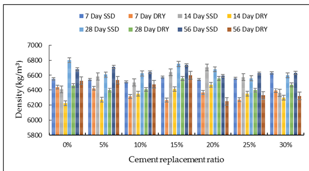
Figure 11. Density in SSD and dry conditions.
