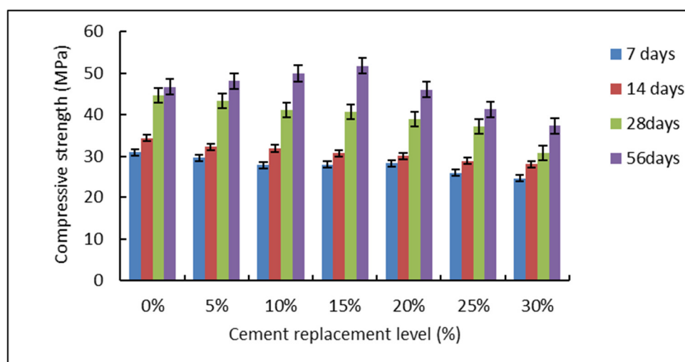
Figure 12. Compressive strength of blended BA mortars.
