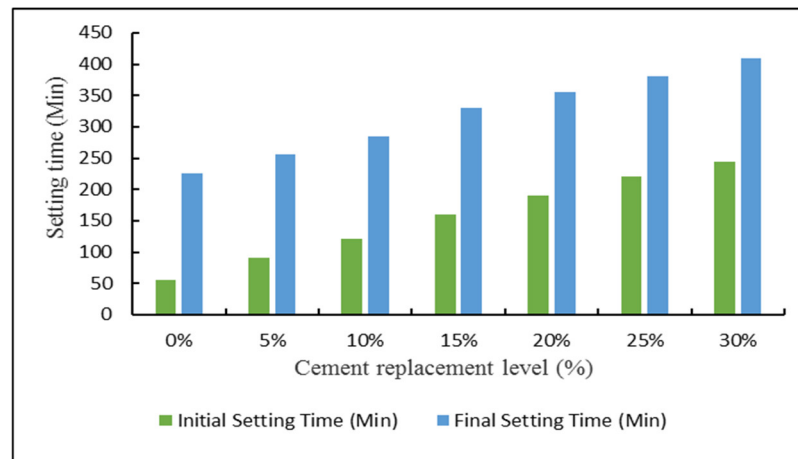
Figure 10. Initial and final setting time of cement paste with BA.
