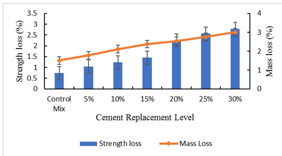
Figure 14. Compressive strength and mass loss in chloride environment (90 days).
