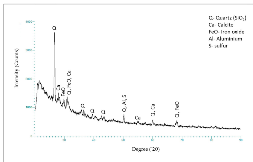
Figure 7. X-ray diffraction (XRD) analysis of BA.
