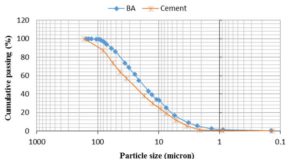
Figure 6. Particle size distribution of ground BA and cement.
