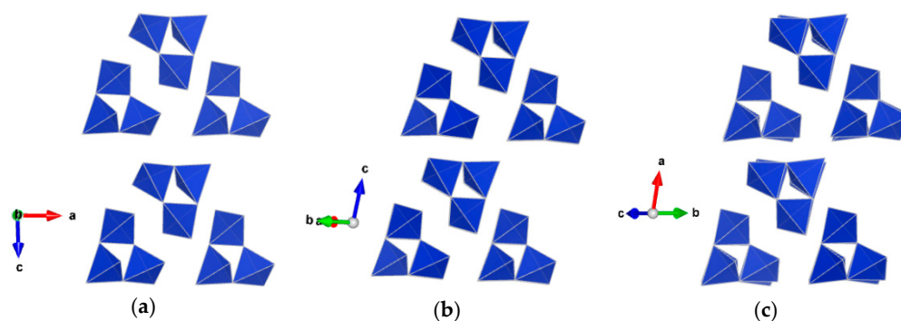
Figure 6. Phase transitions from (a) CaSiO 3 -walstromite-I (b) CaSiO 3 walstromite-II and (c) CaSiO 3 -walstromite-III. The representations of the structure are realized using the program VESTA [17]; a axis is red, the green arrow is the b axis, while the blue arrow is the c axis.
