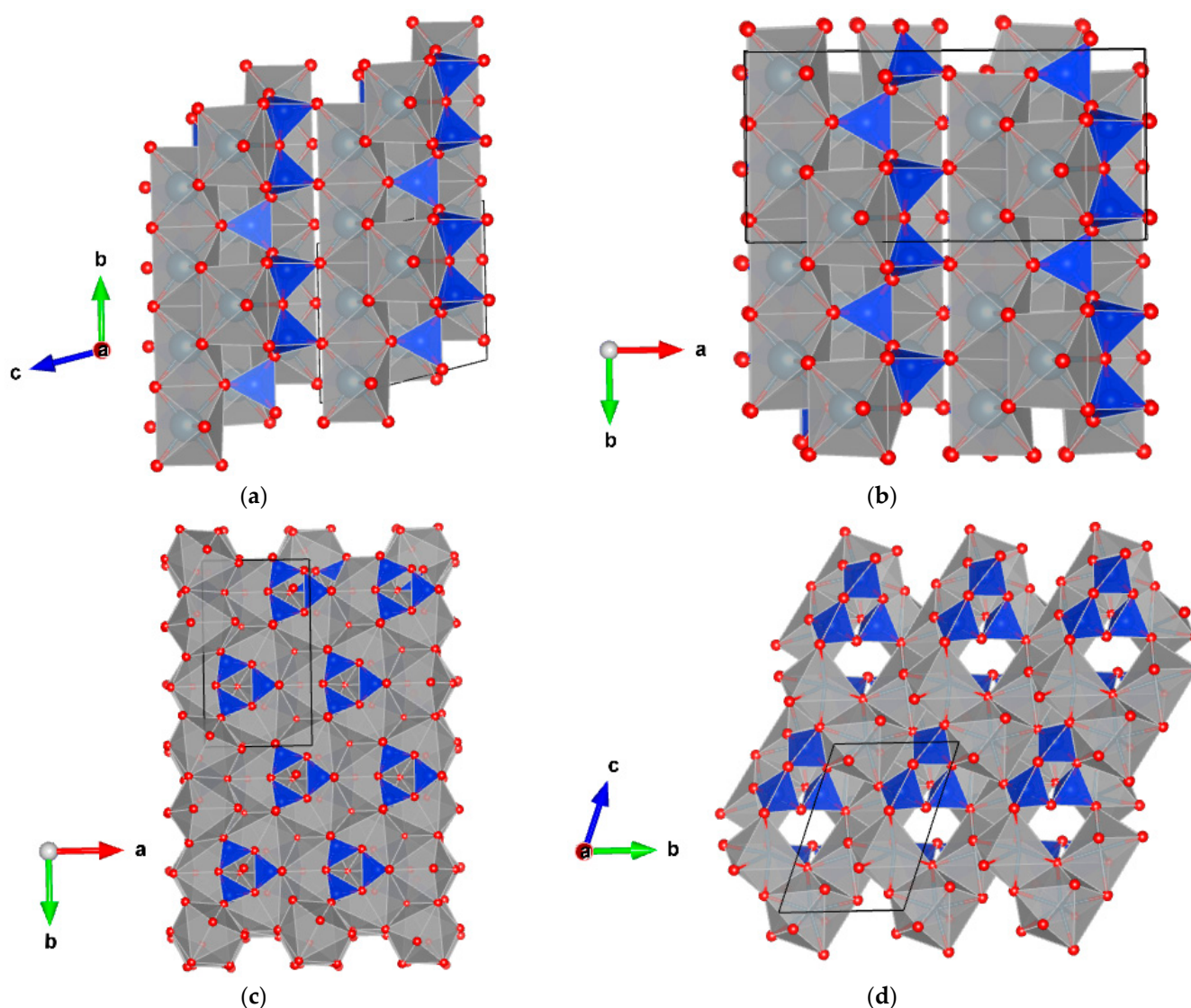
Figure 2. Crystal structure of (a) wollastonite, (b) wollastonite-2M, (c) pseudowollastonite, and (d) breyite. The representations of the structure are realized using the program VESTA [17]. Small red spheres are oxygens, (\text{SiO}_4)^{2-} are blue tetrahedra and grey polygons are Ca cation sites. Black solid lines represent the dimension of the unit cell.
