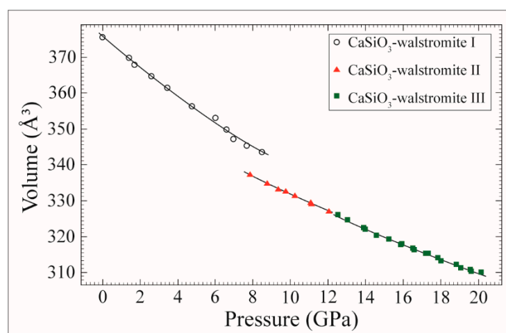
Figure 5. Evolution of the unit-cell volume with pressure of CaSiO 3 -walstromite. Unit-cell volume data of the two HP polytypes have been normalized to the low- P polytype. The solid line represents the 2nd order BM-EoS fit.
