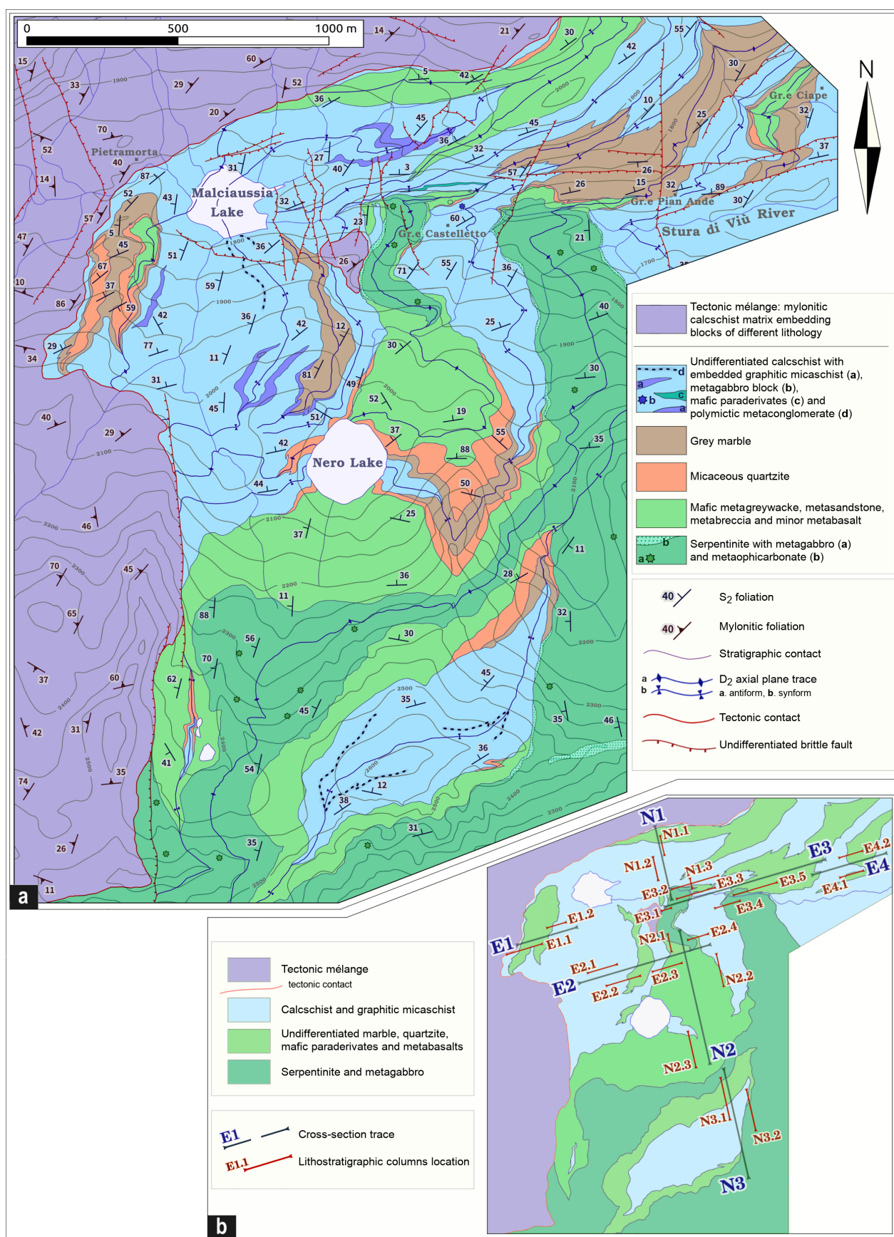
Figure 2. (a) Simplified geological map (1:10,000 scale) of the study area. (b) Schematic map showing the location of cross sections and lithostratigraphic columns. Schematic cross sections are shown in Figure 3. An integrated geological map showing the location of cross sections and lithostratigraphic columns is reported in Figure S1.
