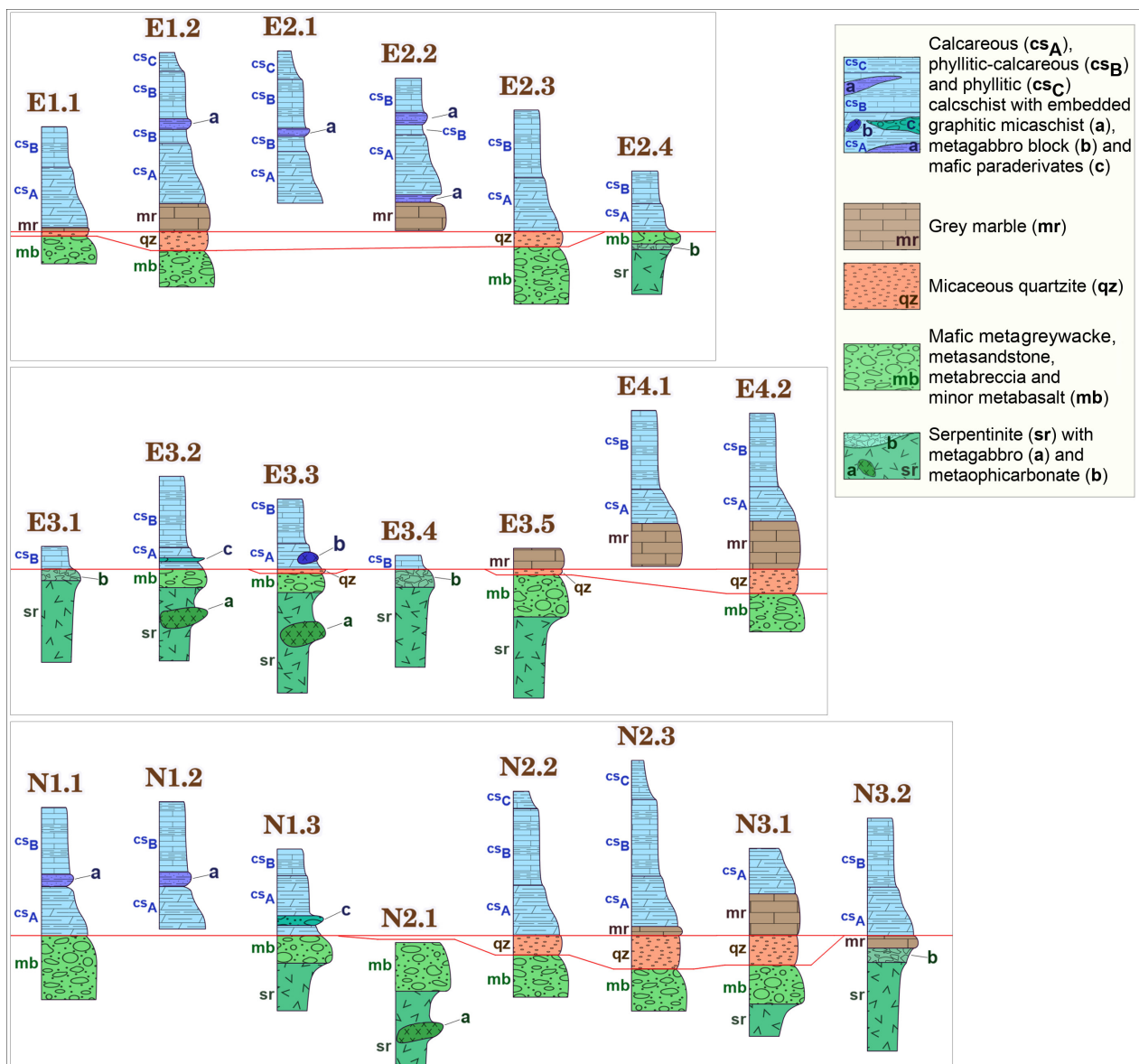
Figure 6. Lithostratigraphic columns (not to scale) reconstructed along the E–W (E1 and E2 above; E3 and E4 middle) and the N–S-oriented (N1, N2, and N3 below) cross sections of Figures 2b and 3. The stratigraphic base of both gray marble and quartzite is correlated throughout all columns with a red line.
