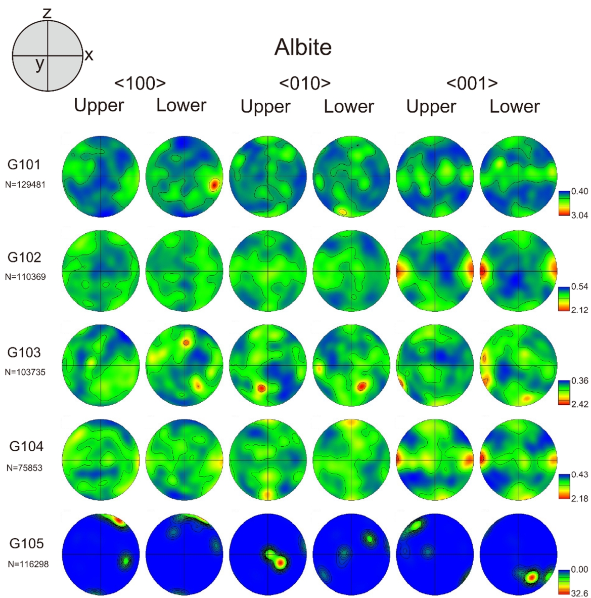
Figure S1. Pole figures of the albite axes presented in the lower hemisphere using equal-area projection.
