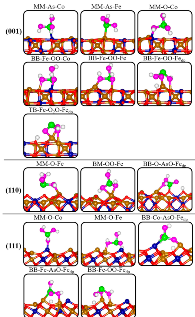
Figure 5. Optimised lowest-energy unique adsorption configurations of H_3AsO_3 on the dry Fe_2CoO_4 (001), (110), and (111) surfaces. H_3AsO_3 molecules enlarged for clarity (Fe = brown, Co = blue, O_{surf} = red, O_{mol} = purple, H = white); dp = deprotonated; MM = monodentate mononuclear; BB = bidentate binuclear.
