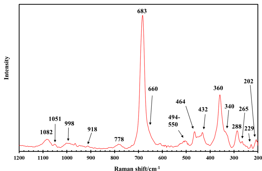
Figure 4. Raman spectrum of natural saponite (Milford) in the region between 1200 and 200 \text{cm}^{-1} .
