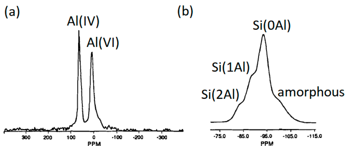
Figure 10. (a) ^{27}\text{Al} magic-angle-spinning nuclear magnetic resonance (MAS-NMR) spectrum of synthetic \text{NH}_4 -saponite and (b) ^{29}\text{Si} MAS-NMR spectrum of synthetic \text{NH}_4 -saponite (modified from [39]).
