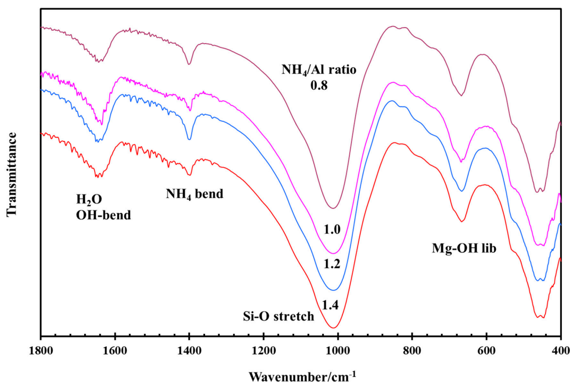
Figure 7. Mid-IR spectra in the region between 1800 and 400\text{ cm}^{-1} of \text{NH}_4 -saponites synthesized with different \text{NH}_4/\text{Al} ratios at 280^\circ\text{C} (modified after [57]).
