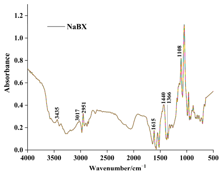
Figure 4. FTIR of NaBX.
