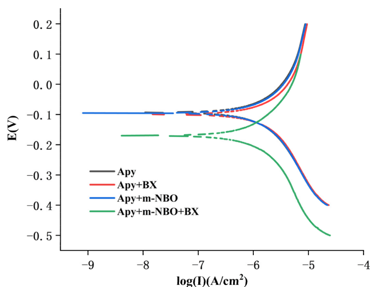
Figure 10. Tafel curves of the arsenopyrite electrode in the presence of m-NBO and NaBX at pH = 9; scanning rate: 10 mV/s, C_{(m-NBO)} = 0.3 \text{ mol}\cdot\text{L}^{-1} , C_{(NaBX)} = 1.6 \times 10^{-3} \text{ mol}\cdot\text{L}^{-1} .
