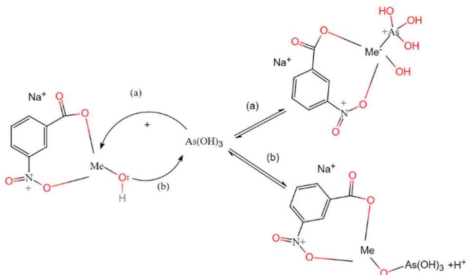
Figure 6. Possible adsorption mechanism of m-NBO on an arsenopyrite surface with two binding mechanisms involving m-NBO: a metal cation and arsenic (Me can be Fe 3+ ). a—is expected to be rather weak due to steric hindrance and repulsion of the OH - ligands and due to a small difference in Pauling’s electronegativity; b—In the case of the Me–O–As bridge, a stable bond is expected.
