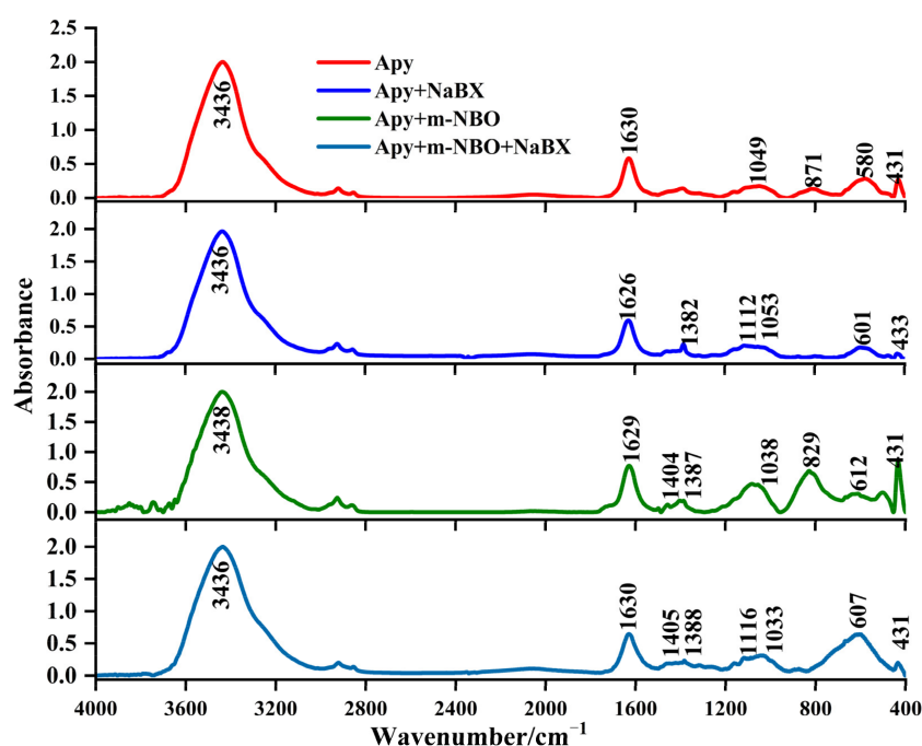
Figure 5. FTIR of arsenopyrite after interaction with m-NBO and NaBX; \text{pH} = 11.5 , C_{(\text{m-NBO})} = 50\text{ mg}\cdot\text{L}^{-1} , C_{(\text{NaBX})} = 1.6 \times 10^{-3}\text{ mol}\cdot\text{L}^{-1} .
