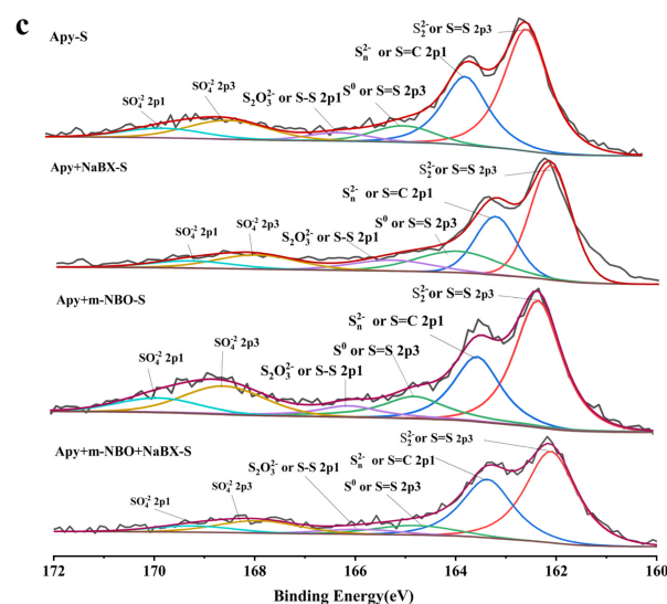
Figure 7. XPS of arsenopyrite after interactions with m-NBO and NaBX; pH = 11.5, C_{(m-NBO)} = 50 \text{ mg} \cdot \text{L}^{-1} , C_{(NaBX)} = 1.6 \times 10^{-3} \text{ mol} \cdot \text{L}^{-1} ; (a) Fe 2p, (b) As 3d, (c) S 2p.
