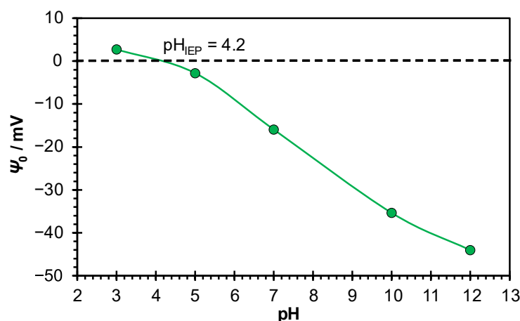
Figure 7. Inner surface potential of \text{Ti}/\text{TiO}_2 ( \Psi_0/\text{mV} ) in 1 \times 10^{-3} \text{ mol dm}^{-3} \text{NaCl} aqueous solutions of different pH, at 25^\circ\text{C} . The isoelectric point of \text{Ti}/\text{TiO}_2 layer ( \text{pH}_{\text{IEP}} = 4.2 [22]) was used to calculate \Psi_0 from E_{\text{oc}} .
