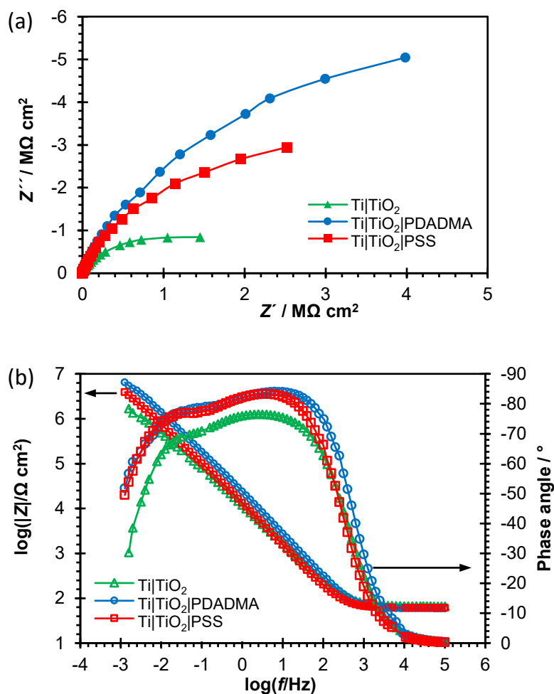
Figure 4. The Nyquist and Bode plots of the unmodified ( \text{Ti}|\text{TiO}_2 ) and polyelectrolyte modified Ti electrodes ( \text{Ti}|\text{TiO}_2|\text{PSS} and \text{Ti}|\text{TiO}_2|\text{PDADMA} ) recorded at the open circuit potential ( E_{oc} ) in 0.1\text{ mol dm}^{-3} NaCl electrolyte solution after 1-h stabilization. Symbols present the experimental data and solid lines present the modeled data.
