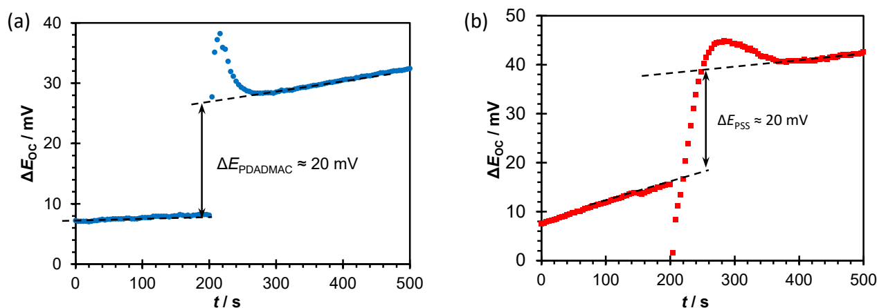
Figure 8. Electrode potential of Ti/TiO 2 -E in 0.001 mol dm −3 NaCl aqueous solution at 25 °C, before, during, and after the addition of polyelectrolyte (a) PDADMA, pH ≈ 11; (b) PSS, pH ≈ 3.
