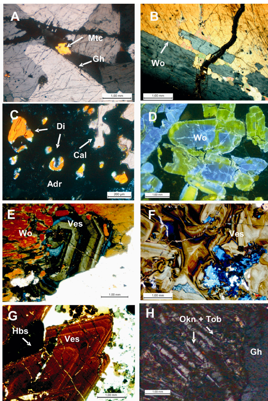
Figure 4. Photomicrographs showing characteristic relationships between minerals in the Măgurea Vaței skarn. (A) Crystal of monticellite (Mtc) engulfed by gehlenite (Gh). Sample Cer-G-5-069, B zone, crossed polars.; (B) Mass of wollastonite-2M (Wo). Sample CE005-c, C zone, crossed polars; (C) Crystals of diopside (Di) and pads of calcite (Cal) in the Ti-andradite (Adr) mass. Sample Cer-G-5-018, A 1 zone, crossed polars; (D) Cathodoluminescence photomicrograph showing zoning in wollastonite (Wo) crystals. Sample 2292, C zone; (E) Zoned vesuvianite (Ves) in the wollastonite (Wo) mass. Sample CE0058-f, B zone, crossed polars; (F) Zoned and brecciate vesuvianite (Ves). Sample Cer-W-6-002. BV zone, crossed polars; (G) “Hibschite” (Hbs) on the fractures of optically zoned vesuvianite (Ves) crystals. Sample 2161, B zone, crossed polars. (H) Aggregates of okenite (Okn) and tobermorite (Tob) on a fissure affecting the gehlenite (Gh) mass. Sample CE 4 b, B zone, crossed polars. When possible, symbols of the rock-forming minerals after [35].
