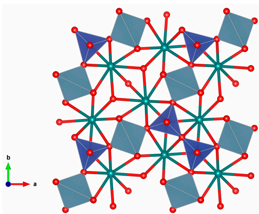
Figure 5. Projection of the structure of gehlenite (sample CE 4 b) along (001). The deep blue tetrahedrons represent \text{SiO}_4 , the gray blue octahedrons represent \text{AlO}_4 , the red circles represent O atoms, and the turquoise circles represent the eight-fold coordinated Ca atoms.
