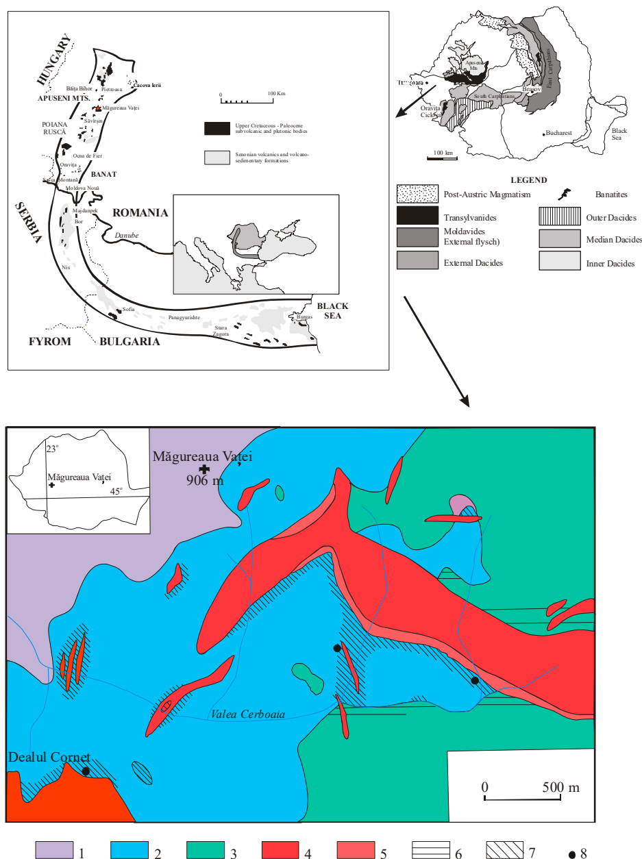
Figure 1. Geological sketch of Măgurea Văței zone (redrawn and modified from [5]) in the regional context: the Banatitic Magmatic and Metallogenetic Belt (top, left: redrawn from [18]) and the structural context of Romania (top, right: redrawn and simplified from) [19]. Symbols in the legend represent: 1—Mesozoic ophiolites; 2—Tithonic–Neocomian limestones (marbles); 3—Senonian clays, sandstones and conglomerates; 4—Quartz monzonites; 5—Monzonites; 6—Pyroxene hornfels; 7—Skarns; 8—Gehlenite occurrences.
