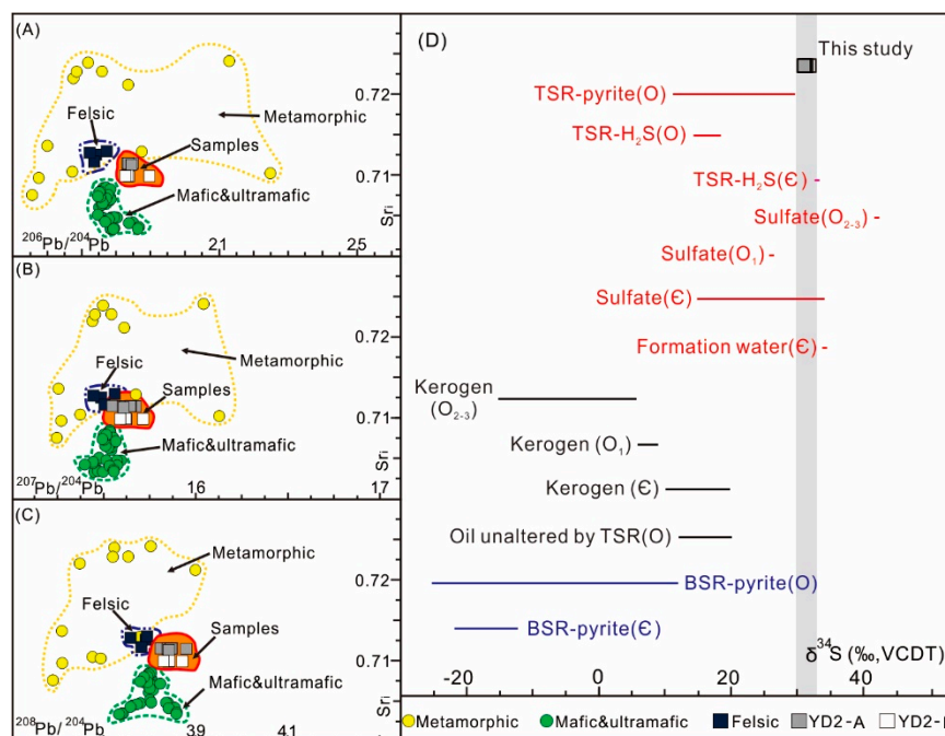
Figure 9. (A): \text{Sr}_i\text{-}^{206}\text{Pb}/^{204}\text{Pb} , (B): \text{Sr}_i\text{-}^{207}\text{Pb}/^{204}\text{Pb} , (C): \text{Sr}_i\text{-}^{208}\text{Pb}/^{204}\text{Pb} and (D): S isotope ratios of the pyrites in this study compared with spatially and temporally associated materials from the literature. Whole-rock Pb isotope ratios were corrected to their initial ratios. €—Cambrian; O—Ordovician; TSR—thermochemical sulfate reduction; BSR—bacterial sulfate reduction; \text{Sr}_i —initial ^{87}\text{Sr}/^{86}\text{Sr} value; VCDT—Vienna Canyon Diablo Troilite. Lead and strontium isotope data sources: (1) felsic rocks: [50,51]; (2) mafic and ultra-mafic rocks: [52–56]; (3) metamorphic rocks: [50,56]. Sulfur isotope data sources: (1) Ordovician BSR-derived pyrites: [14,17–19]; (2) Ordovician TSR-derived pyrites: [13,15,18,19]; (3) Middle-Upper Ordovician sulfates: [17]; (4) Ordovician TSR-derived H 2 S: [57]; (5) Lower Ordovician sulfates: [14]; (6) Lower Ordovician kerogen: [58]; (7) Middle-Upper Ordovician kerogen: [58]; (8) Middle-Upper Ordovician non-degraded oil: [58]; (9) Cambrian BSR-derived pyrites: [16,18]; (10) Cambrian sulfates: [13,14,16,18]; (11) Cambrian formation water: [18]; (12) Cambrian TSR-derived H 2 S: [18]; (13) Cambrian kerogen: [58].
