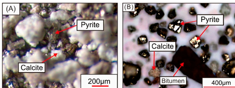
Figure 3. Typical stereo binocular microscope photomicrographs (reflective light) show that pyrites are disseminated in the samples and coexist with calcites in specimen A (A), with bitumen are found to coexist with pyrite and calcite in specimen B (B).
