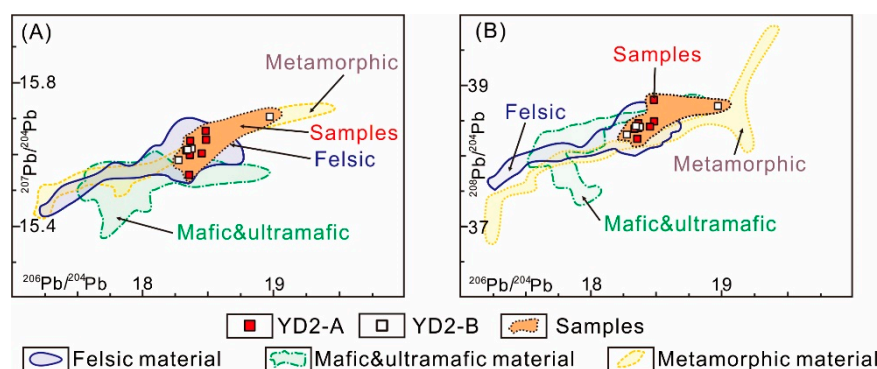
Figure 10. Lead isotope ratios of pyrite sub-samples compared with spatially- and temporally-associated materials ((A): ^{207}\text{Pb}/^{204}\text{Pb} - ^{206}\text{Pb}/^{204}\text{Pb} ; (B): ^{208}\text{Pb}/^{204}\text{Pb} - ^{206}\text{Pb}/^{204}\text{Pb} ). Lead isotope ratios in (A) and (B) are corrected to their initial ratios. The fields of metamorphic, felsic and mafic-ultramafic are drawn according to lead isotope data of material from the literature. Lead isotope data sources: (1) felsic rocks: [50,51]; (2) mafic and ultra-mafic rocks: [52–55]; (3) metamorphic rocks: [50,56].
