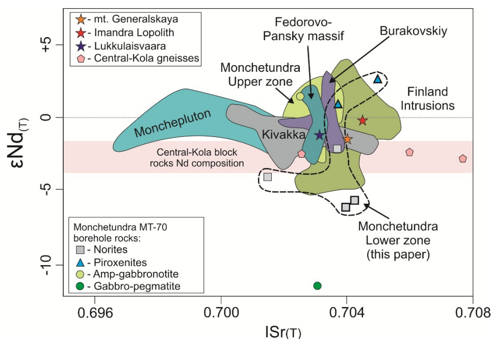
Figure 10. The \epsilon\text{Nd}(i) . \text{ISr}(i) plot for the Monchetundra rocks. Monchetundra massif upper zone, after [4,5,8,29]; Monchepluton massif rocks, after [4,29]; Fedorovo-Pansky massif after [29]; Mt. Generalskaya after [30]; Kivakka after [31,32], Burakovskiy, Lukkulaivaara after [31]; Finland layered intrusions after [29,33] Field of Central-Kola Block rocks, after [26,27]; Central Kola gneisses, after [28]. Ore-bearing rocks are marked in bold.
