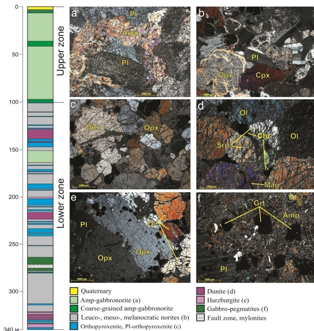
Figure 2. Schematic section of borehole MT-70 modified after [20] and pictures of thin sections of typical rocks from the Loyppishnun area. Pl—plagioclase; Amp—amphibole; Opx—orthopyroxene; Cpx—clinopyroxene; Ol—olivine; Srp—serpentine; Chr—chromite; Mag—magnetite; Grt—garnet; Bt—biotite.
