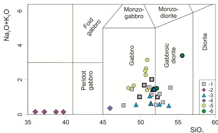
Figure 3. \text{SiO}_2 vs. (\text{Na}_2\text{O} + \text{K}_2\text{O}) plot (wt. %) after [21] for Loypishnun area rocks. 1—norites; 2—dunites; 3—pyroxenites; 4—harzburgite; 5—Amp-gabbro-norite; 6—gabbro-pegmatite. Ore-bearing rocks are marked in bold. Fields of rocks according to [21].
