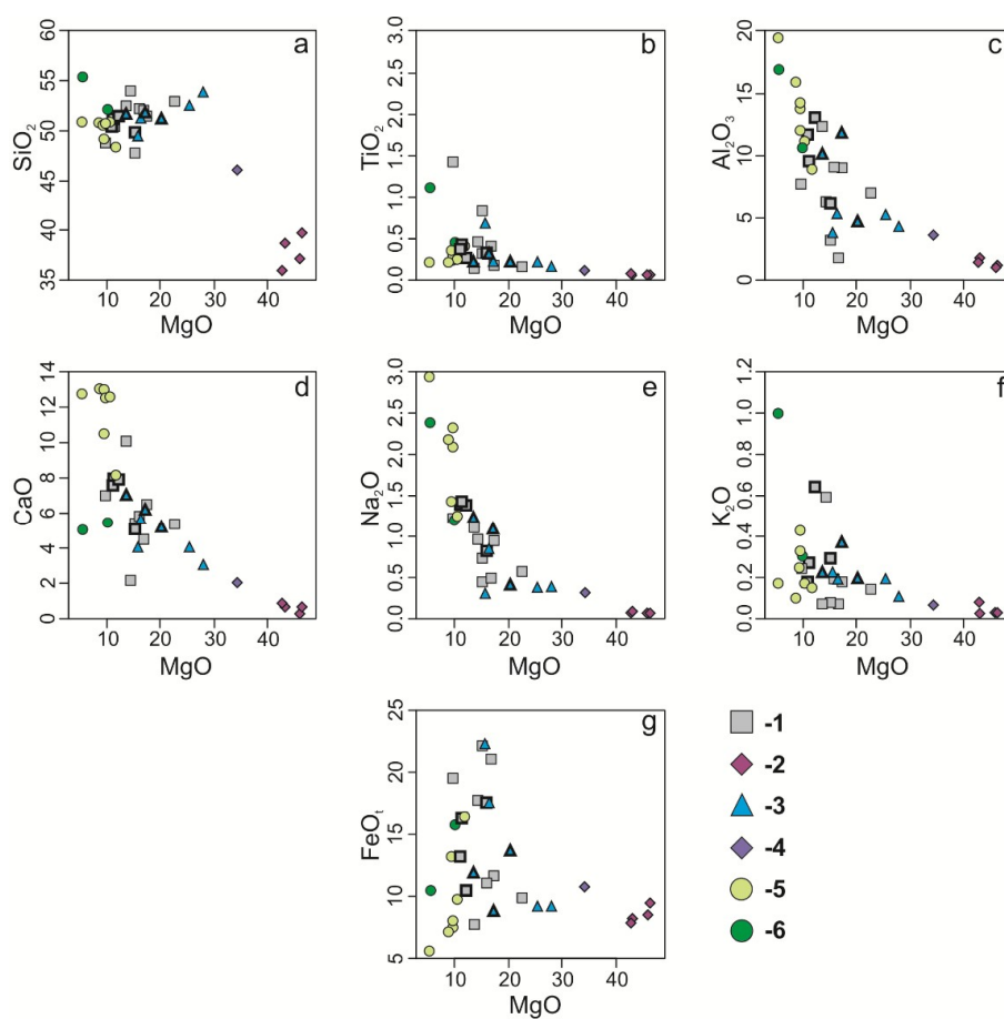
Figure 4. MgO vs. major oxides plot (wt. %) for the Loybishnun area rocks. 1—norites; 2—dunites; 3—pyroxenites; 4—harzburgite; 5—mp-gabbro-norite; 6—gabbro-pegmatite; ore-bearing rocks are marked in bold.
