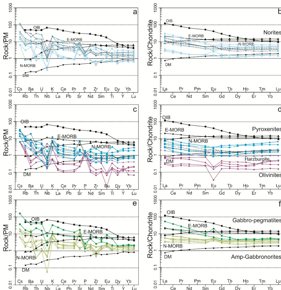
Figure 5. Primitivemantle (PM)-normalized [22] trace elements and chondrite-normalized [23] REE distribution plots for the Loypishnun area rocks. Data on average normal mid-ocean ridge basalt (N-MORB), enriched mid-ocean ridge basalt (E-MORB), oceanic island basalt (OIB), and depleted mantle (DM) shown by black lines are after [22]. Dotted lines indicate the spectra of ore-bearing rocks (PGE > 0.5 ppm).
