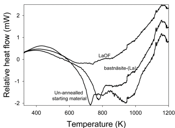
Figure 4. Differential scanning calorimetry (DSC) curves for annealed bastnäsité-(La), unannealed starting material, and LaOF from 325 K to 1223 K. Endotherms can be seen on both the annealed bastnäsité-(La), and unannealed starting material curves from the range near 598 K to 773 K, indicating the decomposition reaction. The LaOF curve does not exhibit this, since it did not decompose. Exotherms at 948 K and endotherms at 1123 K are evident on all three curves, indicating phase transformations.
