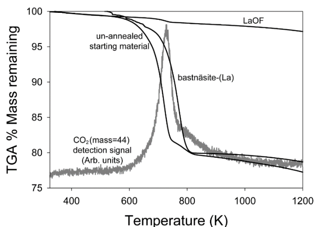
Figure 3. Thermogravimetric analysis (TGA) curves for annealed bastnäsité-(La), unannealed starting material, and LaOF from 325 K to 1223 K. CO 2 detection from the Pfeiffer Vacuum Thermostar Quadrupole mass spectrometer in light gray. Mass loss curves for the starting material and annealed bastnäsité-(La) begin to steepen at 600 K, at the same time CO 2 detection begins. The mass loss curve for LaOF does not show a significant change in slope, indicating that the decomposition reaction did not occur in that sample.
