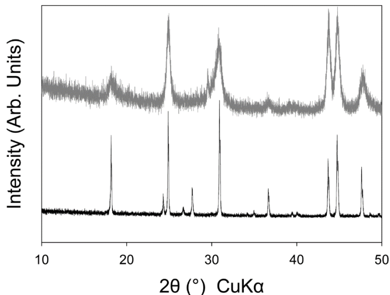
Figure 2. Powder XRD patterns of synthesized bastnäsite-(La) starting material. Top pattern is after washing and drying, bottom pattern is after annealing in the Griggs modified piston cylinder apparatus.
