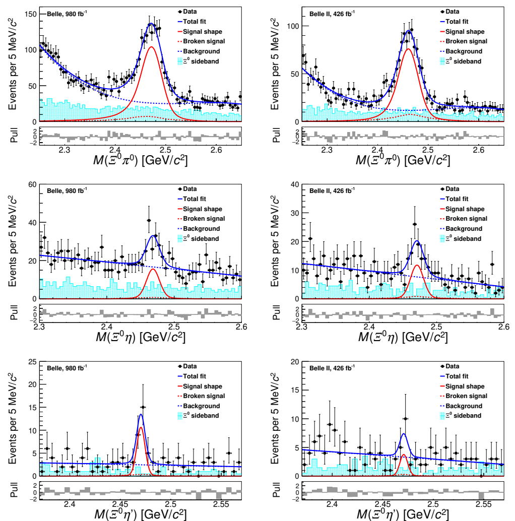
Figure 3. Invariant mass distributions of \Xi_c^0 candidates in data samples for \Xi_c^0 \rightarrow \Xi^0 \pi^0 , \Xi_c^0 \rightarrow \Xi^0 \eta , and \Xi_c^0 \rightarrow \Xi^0 \eta' modes from the (left) Belle and (right) Belle II experiments [9]. The markers with error bars represent the data. The solid blue curves, solid red curves, dashed red curves, and dashed blue curves show the total fit, signal shape, broken-signal shape, and smooth backgrounds, respectively. The cyan histograms show the data from the \Xi^0 mass sidebands.
