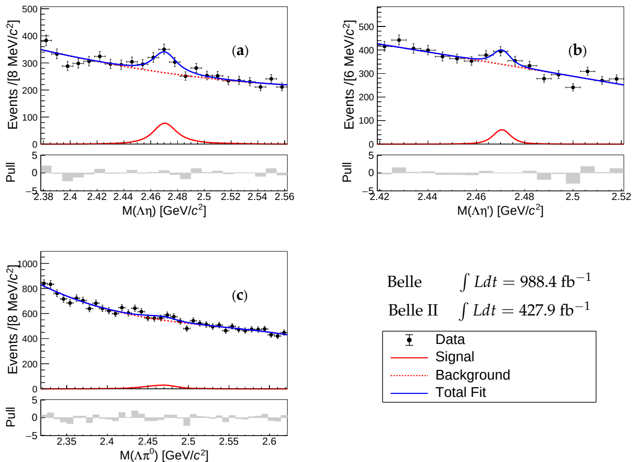
Figure 5. The invariant mass spectra of (a) \Lambda\eta , (b) \Lambda\eta' , and (c) \Lambda\pi^0 candidates overlaid with the fit results obtained using the Belle and Belle II data samples [10]. Dots with error bars represent the number of events in data; solid red curves indicate the signal probability density functions; dashed red lines denote the fitted combinatorial backgrounds; solid blue curves illustrate the fit results. The gray bars show the pull distributions of the fit results.
