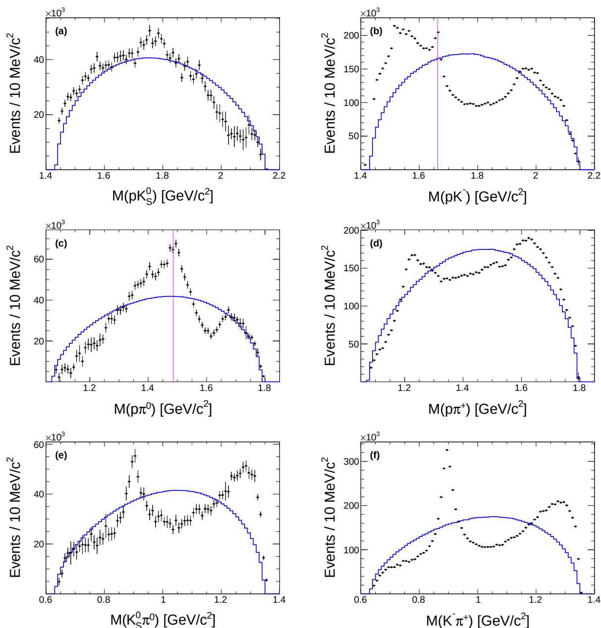
Figure 15. Invariant mass projection spectra for the decays \Lambda_c^+ \rightarrow p K_S^0 \pi^0 (a,c,e) and \Lambda_c^+ \rightarrow p K^- \pi^+ (b,d,f) after subtraction of background contributions and correction for reconstruction efficiency [13]. The expectations from signal Monte Carlo simulations generated according to a phase-space model are overlaid and shown as blue histograms. A pronounced enhancement close to the p\eta mass threshold is observed in panel (c), while the \Lambda\eta and p\eta thresholds are indicated in panels (b,c), respectively. In addition, a distinct resonance peak corresponding to the K^* is visible in the K_S^0 \pi^0 invariant mass distribution shown in panels (e,f).
