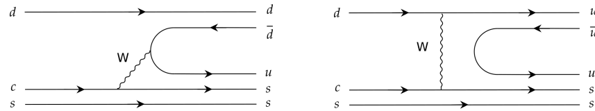
Figure 1. The Feynman diagrams for (left) internal W -emission and (right) W -exchange in \Xi_c^0 \rightarrow \Xi^0 h^0 decays [5].
