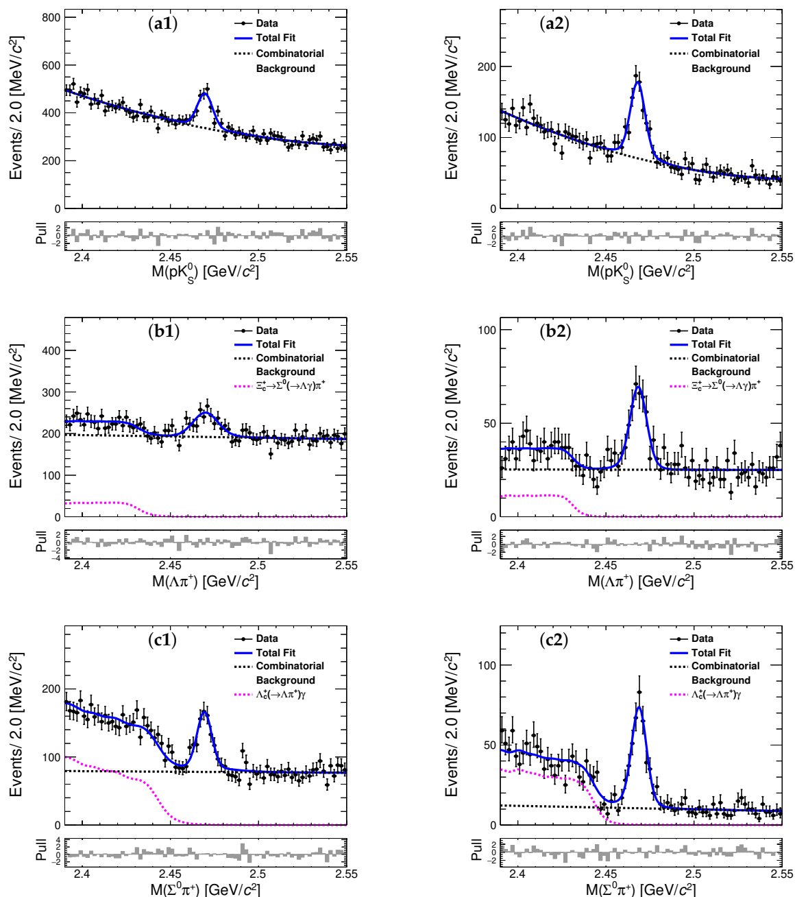
Figure 8. Invariant mass spectra of (a1,a2) pK_S^0 , (b1,b2) \Lambda\pi^+ , and (c1,c2) \Sigma^0\pi^+ in the (1) Belle and (2) Belle II data [11]. The points with error bars represent the data, the solid blue curves show the best-fit results, and the black dashed curves represent the fitted combinatorial backgrounds. In the M(\Lambda\pi^+) and M(\Sigma^0\pi^+) distributions, the pink dashed curves indicate the fitted feed-down backgrounds from the \Xi_c^+ \rightarrow \Sigma^0(\rightarrow \Lambda\gamma)\pi^+ and \Lambda_c^+ \rightarrow \Lambda\pi^+ decays, respectively.
