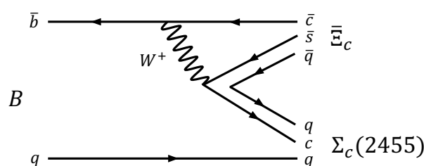
Figure 16. Diagram representing the internal W -boson emission amplitude for the decays B^+ \rightarrow \Sigma_c(2455)^{++}\bar{\Xi}_c^- and B^0 \rightarrow \Sigma_c(2455)^0\bar{\Xi}_c^0 , corresponding to q = u and q = d , respectively.
