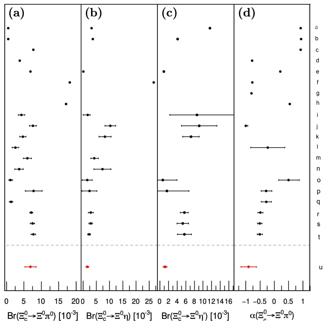
Figure 4. Comparisons of the measured (a) \mathcal{B}(\Xi_c^0 \rightarrow \Xi^0 \pi^0) , (b) \mathcal{B}(\Xi_c^0 \rightarrow \Xi^0 \eta) , (c) \mathcal{B}(\Xi_c^0 \rightarrow \Xi^0 \eta') , and (d) \alpha(\Xi_c^0 \rightarrow \Xi^0 \pi^0) with theoretical predictions. The dots and error bars represent the central values and uncertainties, respectively. Dots without error bars indicate that no theoretical uncertainty is available. The theoretical results correspond to: (a) Körner and Krämer [37], (quark model); (b) Ivanov et al. [38], (quark model); (c) Xu and Kamal [39], (pole model); (d) Cheng and Tseng [40], (pole model); (e) Żenczykowski [41], (pole model); (f) Zou et al. [42], (pole model); (g) Sharma and Verma [43], (current algebra); (h) Cheng and Tseng [40], (current algebra); (i) Geng et al. [44], ( SU(3)_F symmetry (IRA)); (j) Geng et al. [45], ( SU(3)_F symmetry (IRA)); (k) Zhao et al. [50], ( SU(3)_F symmetry (TDA)); (l) Huang et al. [46], ( SU(3)_F symmetry (IRA)); (m) Hsiao et al. [51], ( SU(3)_F symmetry (TDA)); (n) Hsiao et al. [51], ( SU(3)_F -breaking (TDA)); (o) Zhong et al. [47], ( SU(3)_F symmetry (IRA)); (p) Zhong et al. [47], ( SU(3)_F -breaking (IRA)); (q) Xing et al. [49], ( SU(3)_F symmetry (IRA)); (r) Geng et al. [53], ( SU(3)_F symmetry (KPW)); (s) Zhong et al. (I) [52], ( SU(3)_F (TDA)); (t) Zhong et al. (II) [52], ( SU(3)_F (IRA)); and (u) the Belle and Belle II combined measurements. Throughout this review, TDA refers to the topological diagram approach, and IRA is the irreducible representation amplitude. The KPW impose the Körner–Pati–Woo theorem, which restricts certain decay amplitudes due to the antisymmetry of diquark configurations.
