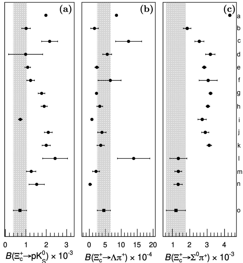
Figure 9. Comparisons of the measured (a) \mathcal{B}(\Xi_c^+ \rightarrow pK_S^0) , (b) \mathcal{B}(\Xi_c^+ \rightarrow \Lambda\pi^+) , and (c) \mathcal{B}(\Xi_c^+ \rightarrow \Sigma^0\pi^+) with theoretical predictions. The dots and error bars represent the central values and uncertainties of the theoretical predictions, respectively. The dots without error bars indicate that no theoretical uncertainty is available. The squares and error bars denote the measured central values and uncertainties in this work. The meanings of the vertical coordinates (a)–(o) in the figure: (a) Zou et al. [42], (pole model); (b) Geng et al. [44], (SU(3) F symmetry (IRA)); (c) Geng et al. [45], (SU(3) F symmetry (IRA)); (d) Huang et al. [46], (SU(3) F symmetry (IRA)); (e) Zhong et al. (I) [47], (SU(3) F symmetry (IRA)); (f) Zhong et al. (II) [47], (SU(3) F -breaking (IRA)); (g) Xing et al. [48], (SU(3) F symmetry (IRA)); (h) Geng et al. [53], (SU(3) F with KPW constraint); (i) Liu [54], (SU(3) F symmetry (IRA)); (j) Zhong et al. (I) [52], (SU(3) F (TDA)); (k) Zhong et al. (II) [52], (SU(3) F (IRA)); (l) Zhao et al. [50], (SU(3) F symmetry (TDA)); (m) Hsiao et al. (I) [51], (SU(3) F symmetry (TDA)); (n) Hsiao et al. (II) [51], (SU(3) F -breaking (TDA)); (o) Belle and Belle II combined.
