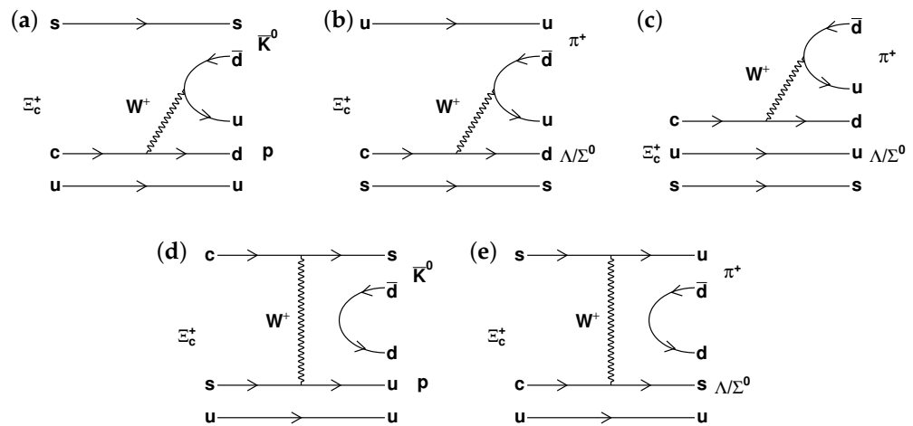
Figure 7. Typical decay diagrams from (a,b) internal W -emission, (c) external W -emission, and (d,e) W -exchange contributions for the SCS decays \Xi_c^+ \rightarrow pK_S^0 , \Xi_c^+ \rightarrow \Lambda\pi^+ , and \Xi_c^+ \rightarrow \Sigma^0\pi^+ .
