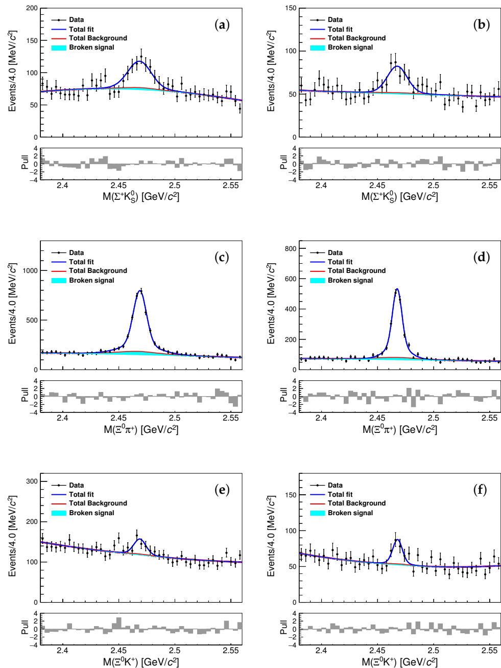
Figure 10. Invariant mass distributions of \Xi_c^+ candidates from \Xi_c^+ \rightarrow \Sigma^+ K_S^0 , \Xi_c^+ \rightarrow \Xi^0 \pi^+ , and \Xi_c^+ \rightarrow \Xi^0 K^+ decays reconstructed in the (a,c,e) Belle and (b,d,f) Belle II data [12]. The black dots with error bars represent the distributions from data. The solid blue and red curves show the total fit and total background, respectively. The cyan areas indicate the broken-signal component.
