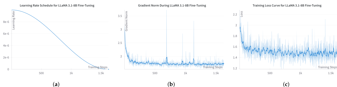
Figure 6. Fine-tuning performance metrics for LLaMA 3.1-8B. This figure showcases the (a) learning rate dynamics, (b) gradient norm fluctuations, and (c) training loss progression.
