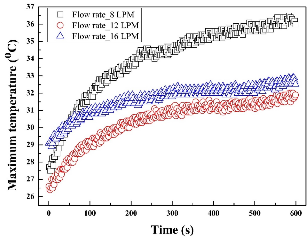
(a) Overload operating power of 8.28 kW
