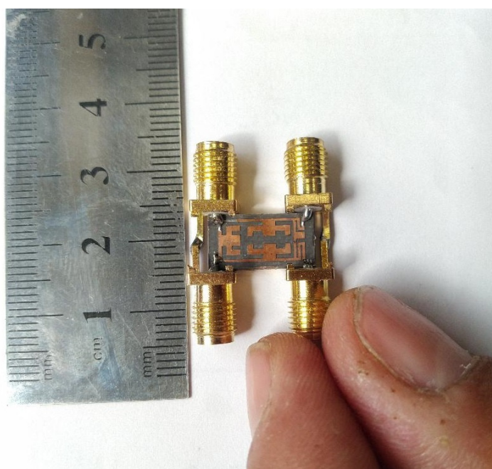
Figure 11. Fabricated Coupler.
