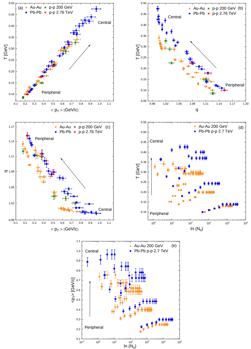
Figure 5. Plots (a–e) show the correlation of T and \langle p_T \rangle , T and q , q and \langle p_T \rangle , T and \ln(N_0) , and \langle p_T \rangle and \ln(N_0) , respectively, in different centrality bins in Au–Au collision at \sqrt{s_{NN}} = 200 GeV and in Pb–Pb collision at \sqrt{s_{NN}} = 2.76 TeV, plots (a–c) also show the results from p–p collision at these collision energies which are comparable to the results of peripheral A–A collision at the same energy.
