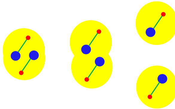
Figure 6. The spatial configuration. Left: compact molecule state; middle: hydrogen molecule-like state; right: deuteron-like state. Big blue ball and small red ball represent Q and \bar{q} , respectively. A large yellow ball represents a subcluster. Taken from Ref. [154].
