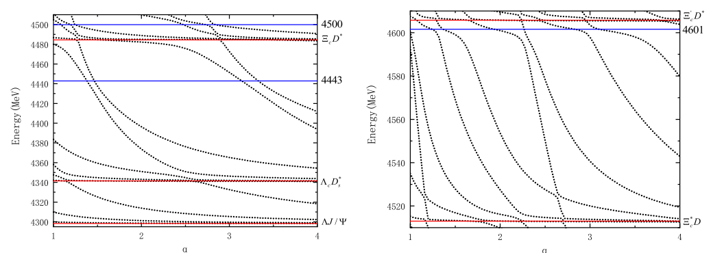
Figure 10. Energy spectrum of the I(J^P) = 0(\frac{3}{2}^-) system. Taken from Ref. [319].
