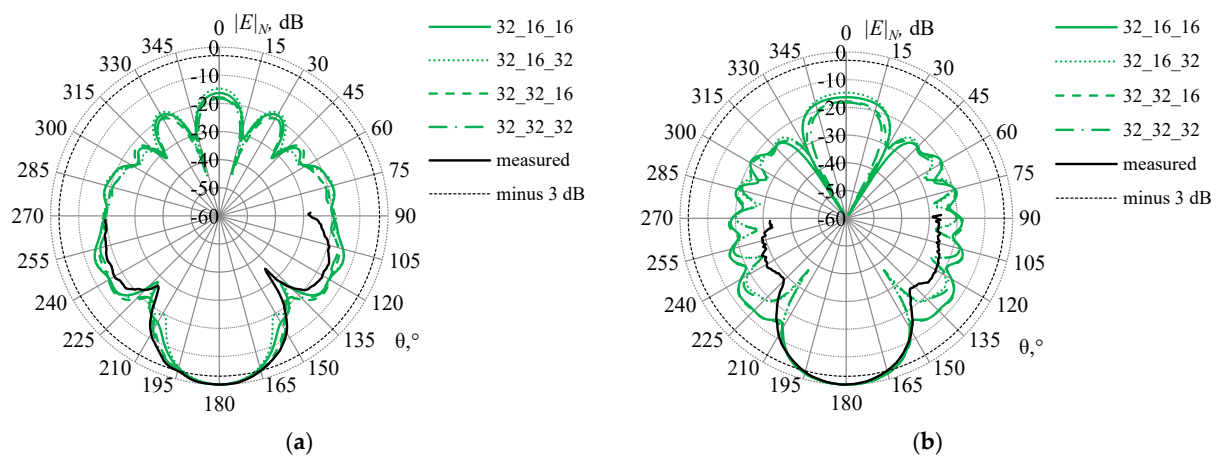
Figure 23. The measured and the calculated RPs ( |E|_N , dB) of the horn AE at the frequency of 8 GHz in the \varphi = 90^\circ (a) and \varphi = 0^\circ (b) planes in the wire-grid with L_r = 32 , n = 40 , L_e = 16, 32 , and SZ_e = SX_e or equal to SX_e * 2^{\pm 1} . The level of -3 dB (—).
