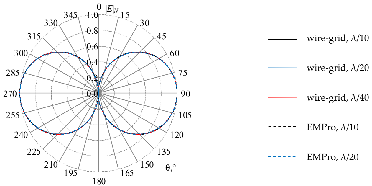
Figure 11. The normalized RP ( |E|_N , times) of the biconical AE with a = 508 mm and \Theta_1 = \Theta_2 = 53.1^\circ when ka_1 = 1.0640 ( f_1 = 0.1 GHz), calculated by the wire-grid and EMPro.
