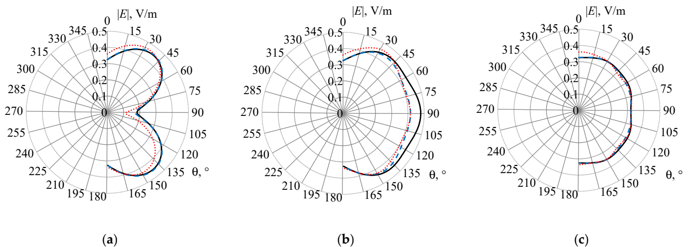
Figure 8. The RP of a dipole on a conducting plate at \theta = 0, 1, \dots, 180^\circ , \varphi = 0^\circ (a), 45^\circ (b), and 90^\circ (c) using the wire-grid by (1) (—), by (3) (—), and EMPro (·····).
