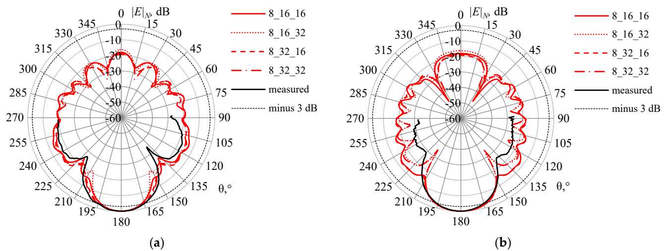
Figure 21. The measured and the calculated RPs ( |E|_N , dB) of the horn AE at the frequency of 8 GHz in the \varphi = 90^\circ (a) and \varphi = 0^\circ (b) planes in the wire-grid with L_r = 8 , n = 40 , L_e = 16, 32 , and SZ_e = SX_e or equal to SX_e * 2^{\pm 1} . The level of -3 dB (—).
