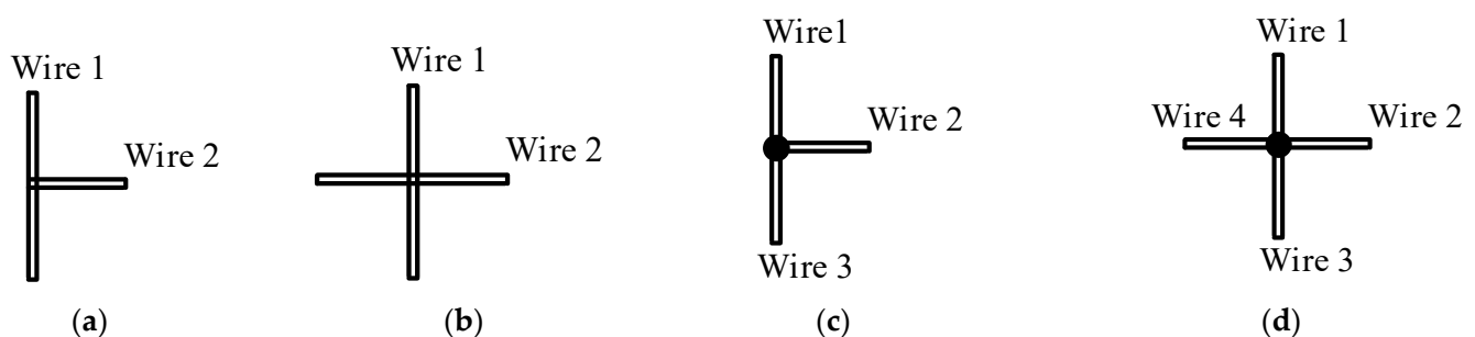
Figure 1. Incorrect (a,b) and correct wire intersections (c,d).
