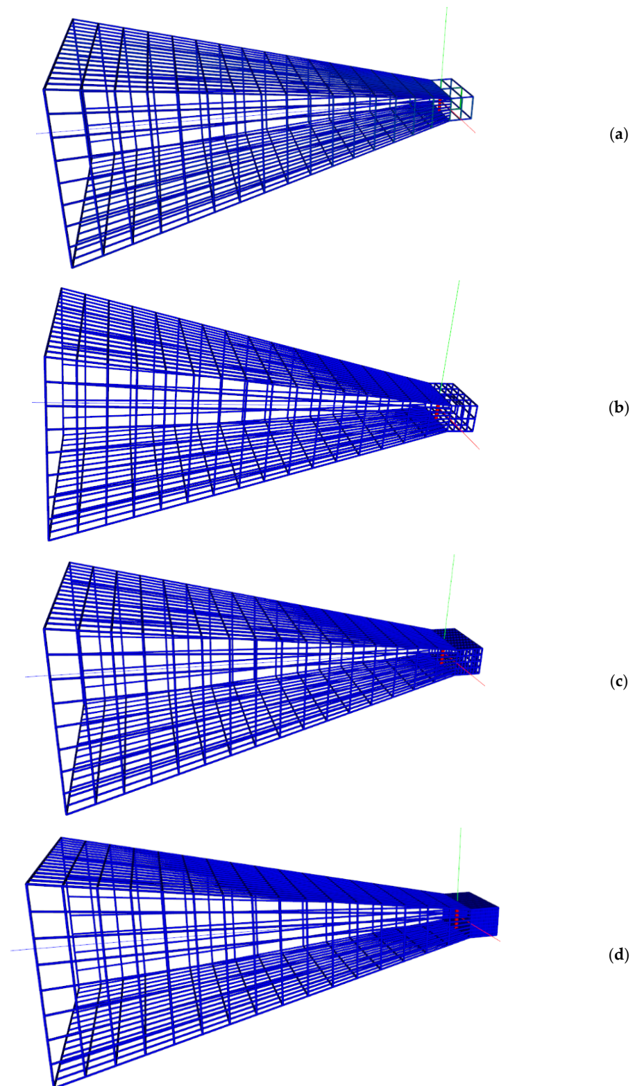
Figure 18. General views of AEs with the wire used as an excitation source built in the wire-grid using L_e = 16 and L_r = 2 (a), 4 (b), 8 (c), and 16 (d).
