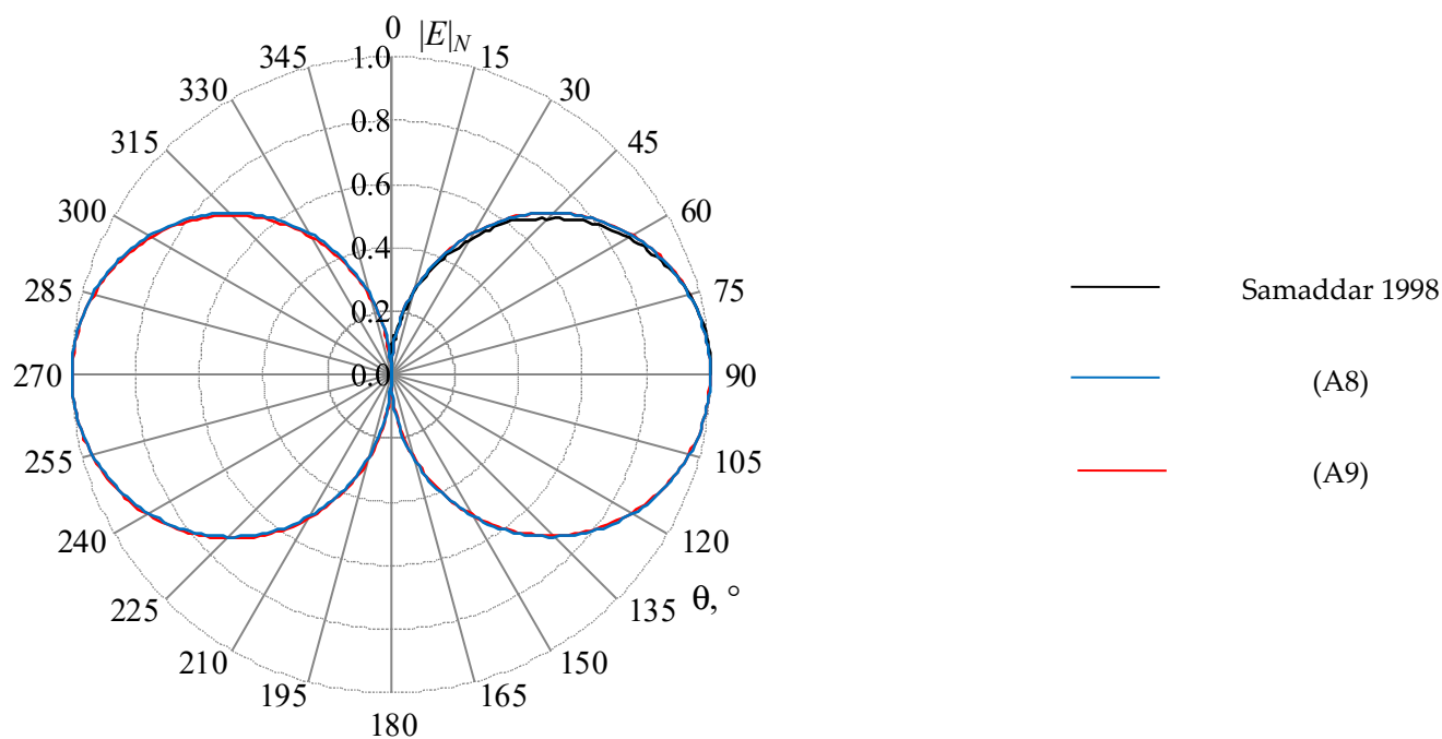
Figure A2. The normalized RP ( |E|_N , times) of the biconical AE with a = 508 mm and \Theta_1 = \Theta_2 = 53.1^\circ with ka_1 = 1.0640 ( f_1 = 0.1 GHz), calculated analytically [62].
