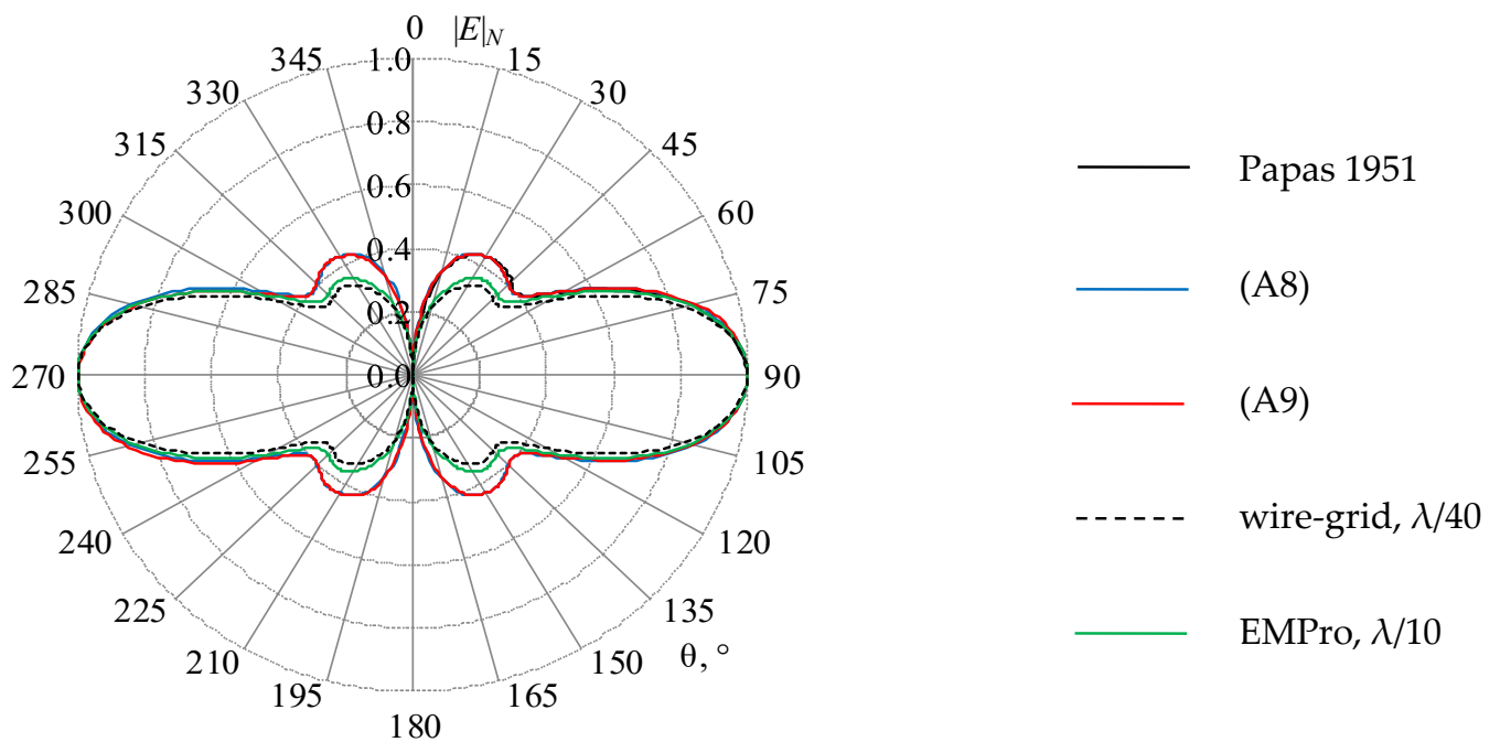
Figure 15. The normalized RP ( |E|_N , times) of the biconical AE when ka_2 = 5.3198 ( f_1 = 0.5 GHz), calculated analytically [61] and by the wire-grid and EMPro at different mesh sizes.
