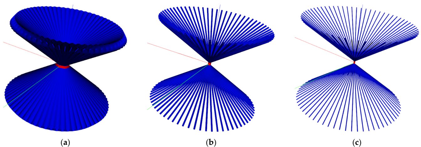
Figure 10. A general view of the biconical AE at frequencies of 0.1 (a), 0.5 (b), and 1 GHz (c) (the view is changing because the wire radius reduces with the frequency growth).
