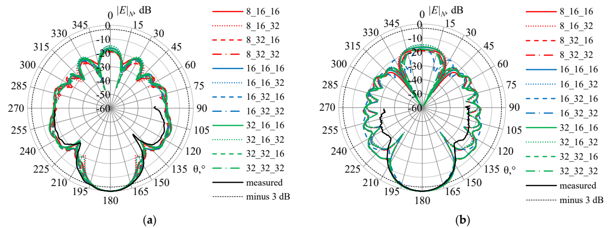
Figure 24. The measured and the calculated RPs ( |E|_N , dB) of the horn AE at the frequency of 8 GHz in the \varphi = 90^\circ (a) and \varphi = 0^\circ (b) planes in the wire-grid with L_r = 8, 16, 32 , n = 40 , L_e = 16, 32 , and SZ_e = SX_e or equal to SX_e * 2^{\pm 1} . The level of -3 dB (—).
