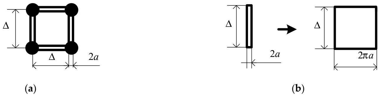
Figure 3. A wire-grid element (a) and the area of one wire surface (b).
