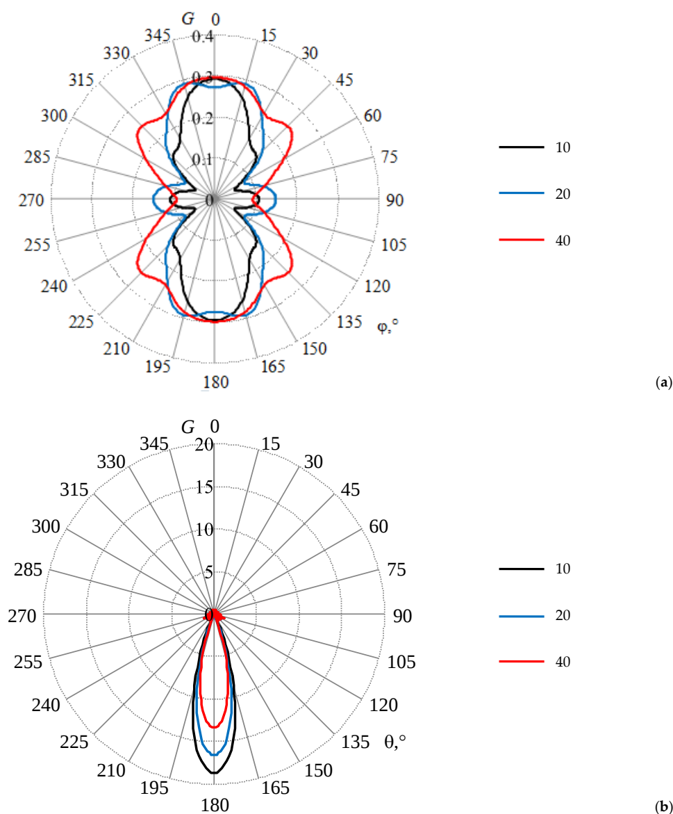
Figure A5. The gain ( G , times) of the horn AE at the frequency of 8 GHz in \theta = 90^\circ (a) and \phi = 90^\circ planes (b), calculated in the wire-grid, with L_r = 2 and n = 10, 20 , and 40.
