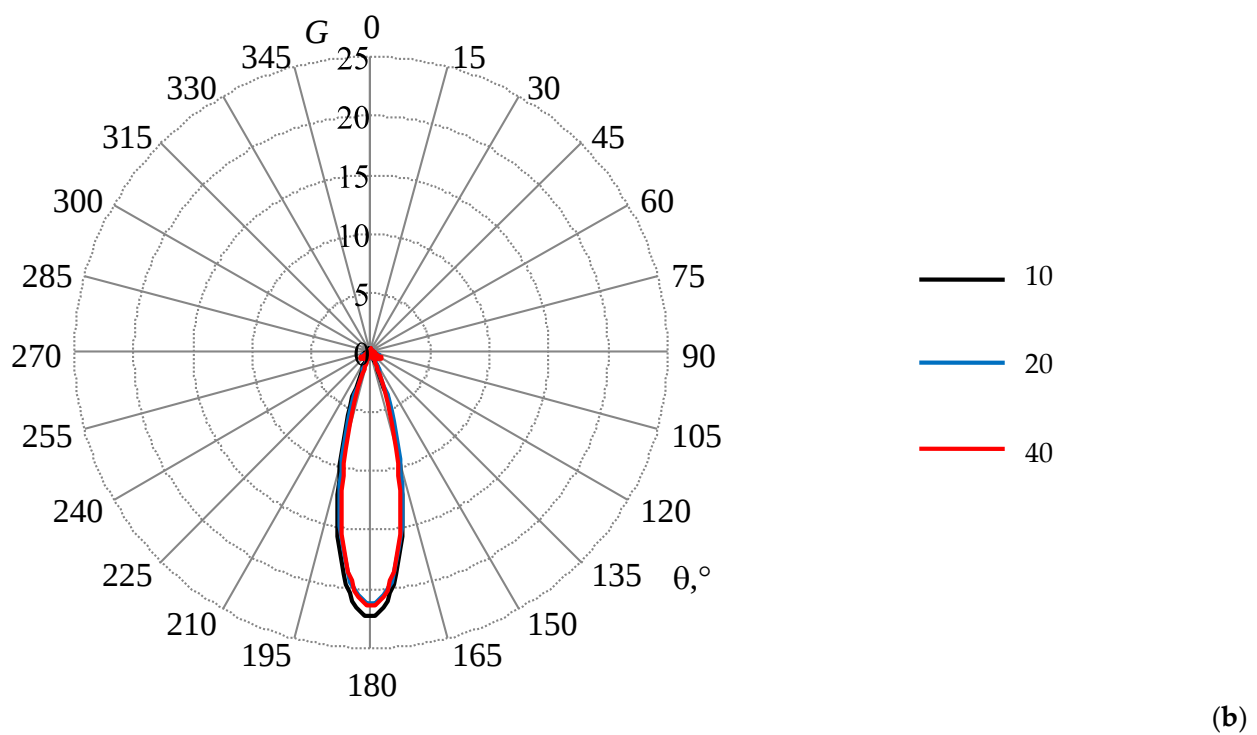
Figure A8. The gain ( G , times) of the horn AE at the frequency of 8 GHz in \theta = 90^\circ (a) and \varphi = 90^\circ planes (b), calculated in the wire-grid, with L_r = 16 and n = 10, 20 , and 40 .
