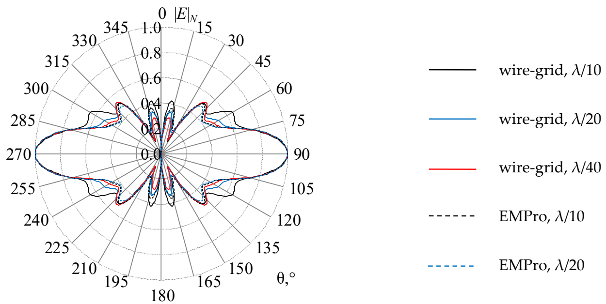
Figure 13. The normalized RP ( |E|_N , times) of the biconical AE with a = 508 mm and \Theta_1 = \Theta_2 = 53.1^\circ when ka_3 = 10.6395 ( f_1 = 1 GHz), calculated by the wire-grid and EMPro.
