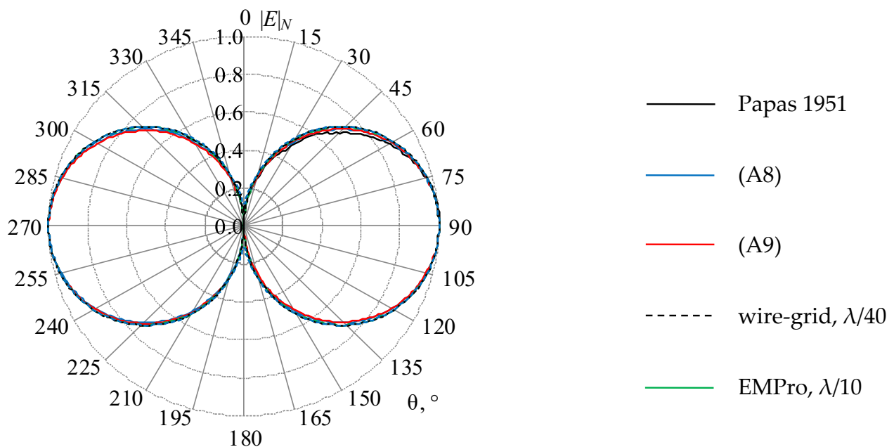
Figure 14. The normalized RP ( |E|_N , times) of the biconical AE when ka_1 = 1.0640 ( f_1 = 0.1 GHz), calculated analytically [61] and by the wire-grid and EMPro at different mesh sizes.
