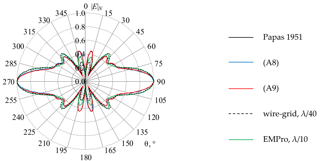
Figure 16. The normalized RP ( |E|_N , times) of the biconical AE when ka_3 = 10.6395 ( f_1 = 1 GHz), calculated analytically [61] and by the wire-grid and EMPro at different mesh sizes.
