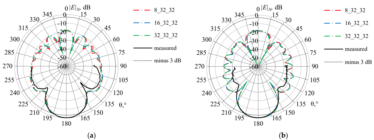
Figure 25. The measured and the calculated RPs ( |E|_N , dB) of the horn AE at the frequency of 8 GHz in the \varphi = 90^\circ (a) and \varphi = 0^\circ (b) planes in the wire-grid with L_r = 8, 16, 32 , n = 40 , L_e = 32 , and SZ_e = SX_e . The level of -3 dB (—).
