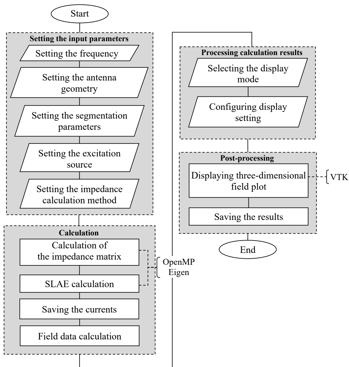
Figure 5. The workflow of the developed module (wire-grid).
