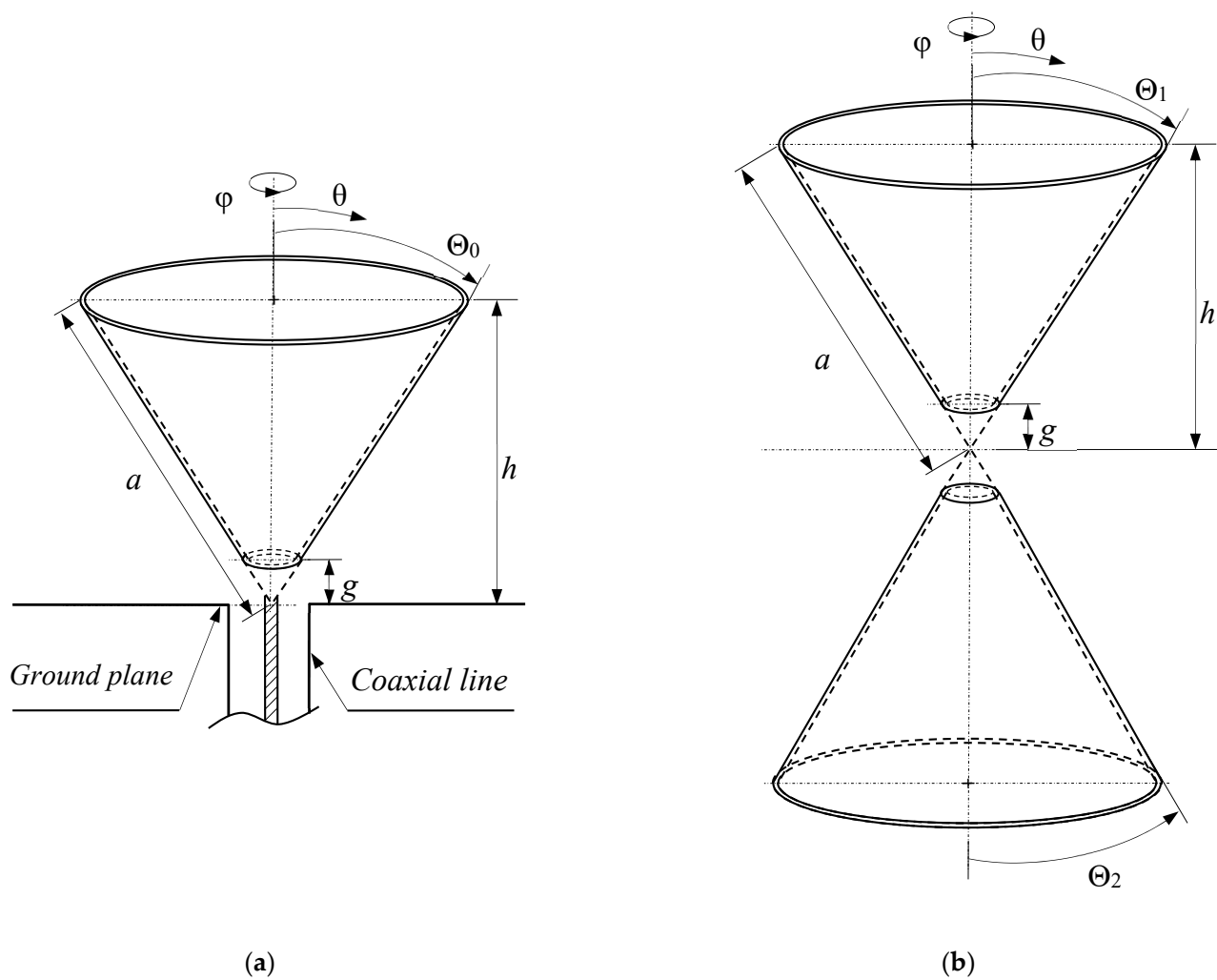
Figure 9. The conical (a) and the biconical (b) AEs.
