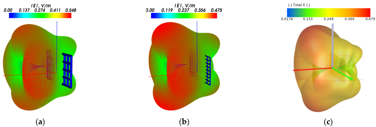
Figure 7. The RP of a dipole on a conducting plate modeled using the wire-grid by (1) (a), by (3) (b), and EMPro (c).
