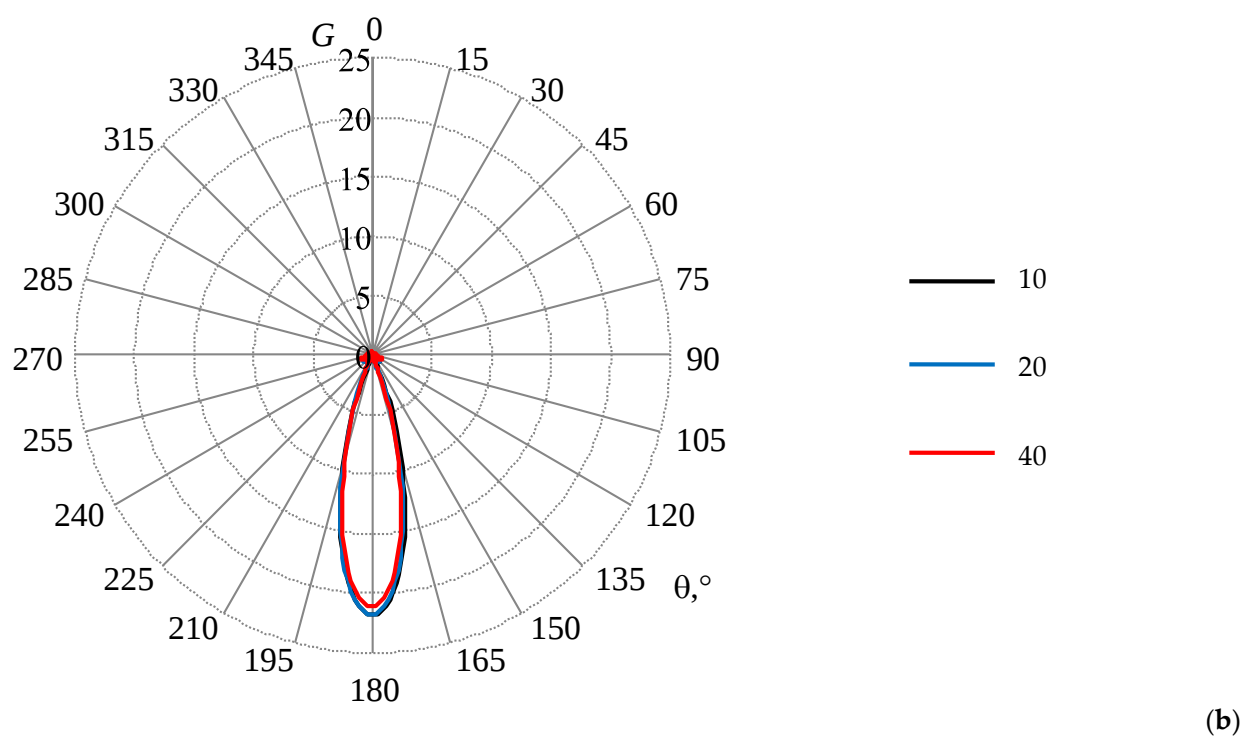
Figure A7. The gain ( G , times) of the horn AE at the frequency of 8 GHz in \theta = 90^\circ (a) and \varphi = 90^\circ planes (b), calculated in the wire-grid, with L_r = 8 and n = 10, 20 , and 40.
