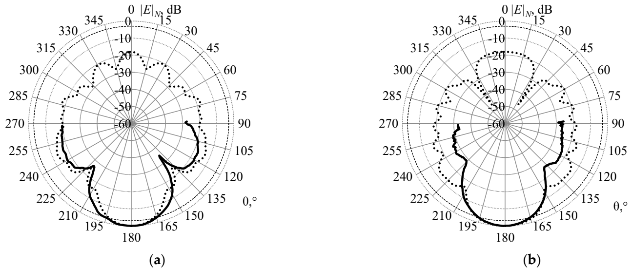
Figure 20. The measured (—) and the calculated (····) RPs ( |E|_N , dB) of the horn AE at the frequency of 8 GHz in the \varphi = 90^\circ (a) and \varphi = 0^\circ (b) planes in the wire-grid with L_e = 16 and L_r = 8 , n = 40 . The level of -3 dB (—).
