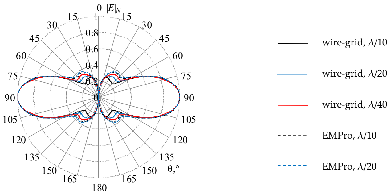
Figure 12. The normalized RP ( |E|_N , times) of the biconical AE with a = 508 mm and \Theta_1 = \Theta_2 = 53.1^\circ when ka_2 = 5.3198 ( f_1 = 0.5 GHz), calculated by the wire-grid and EMPro.
