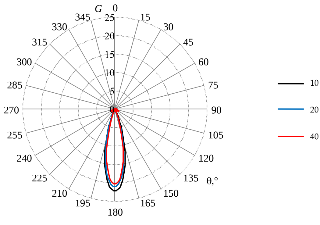
Figure A6. The gain ( G , times) of the horn AE at the frequency of 8 GHz in \theta = 90^\circ (a) and \varphi = 90^\circ planes (b), calculated in the wire-grid, with L_r = 4 and n = 10, 20 , and 40 .
