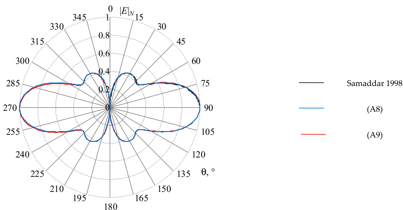
Figure A3. The normalized RP ( |E|_N , times) of the biconical AE with a = 508 mm and \Theta_1 = \Theta_2 = 53.1^\circ with ka_1 = 5.3198 ( f_2 = 0.5 GHz), calculated analytically [62].
