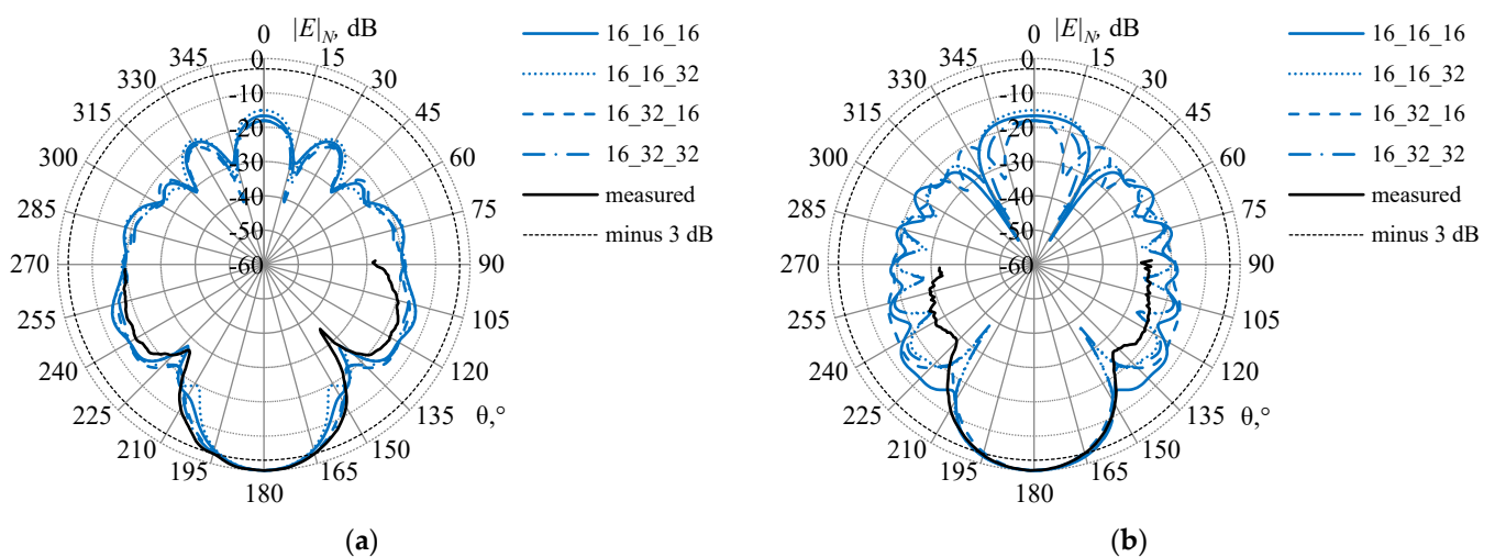
Figure 22. The measured and the calculated RPs ( |E|_N , dB) of the horn AE at the frequency of 8 GHz in the \varphi = 90^\circ (a) and \varphi = 0^\circ (b) planes in the wire-grid with L_r = 16 , n = 40 , L_e = 16, 32 , and SZ_e = SX_e or equal to SX_e * 2^{\pm 1} . The level of -3 dB (—).
