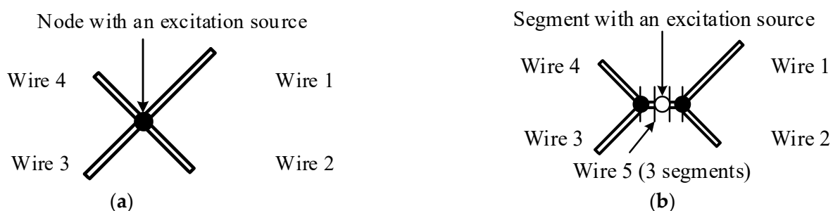
Figure 2. Incorrect (a) and correct (b) setting of the excitation source at the wire intersection.
