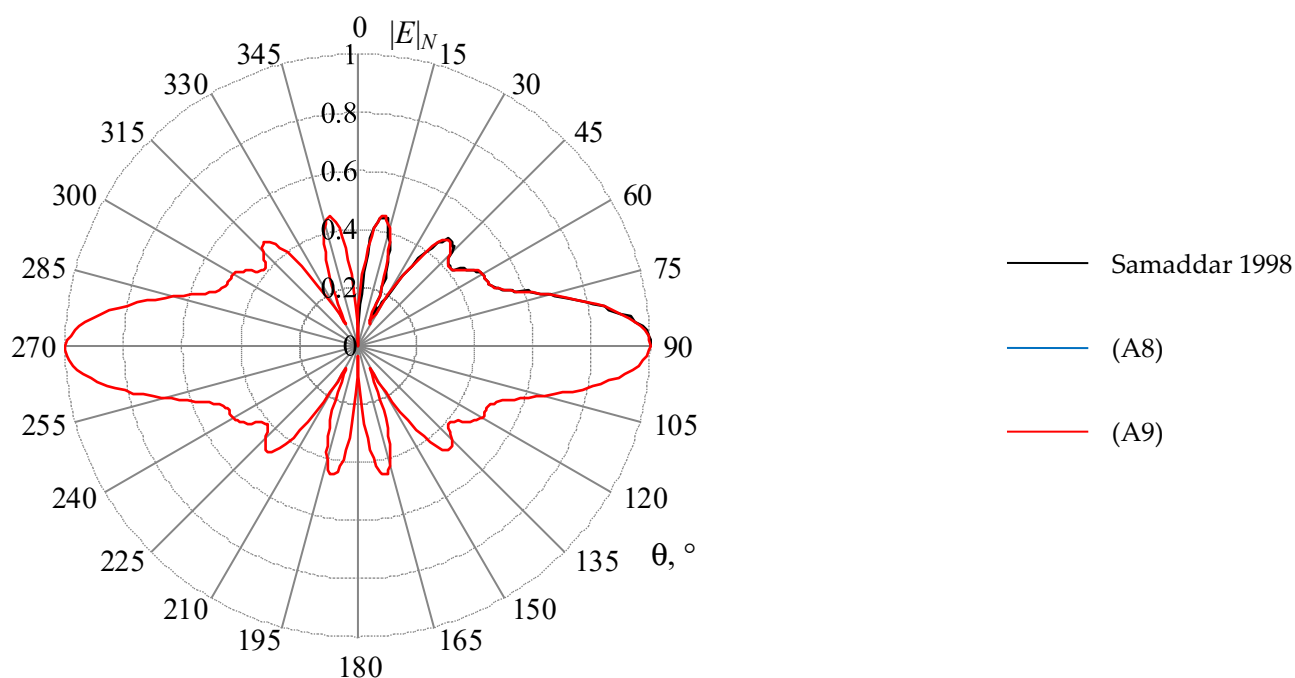
Figure A4. The normalized RP ( |E|_N , times) of the biconical AE with a = 508 mm and \Theta_1 = \Theta_2 = 53.1^\circ with ka_3 = 10.6395 ( f_3 = 1 GHz), calculated analytically [62].
