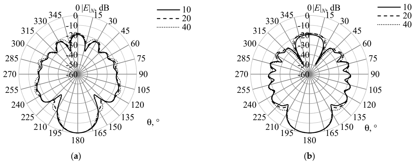
Figure 19. The RPs ( |E|_N , dB) of the horn AE at the frequency of 8 GHz in the \varphi = 90^\circ (a) and \varphi = 0^\circ (b) planes in the wire-grid with L_e = 16 and L_r = 8 , n = 10, 20, 40 .
