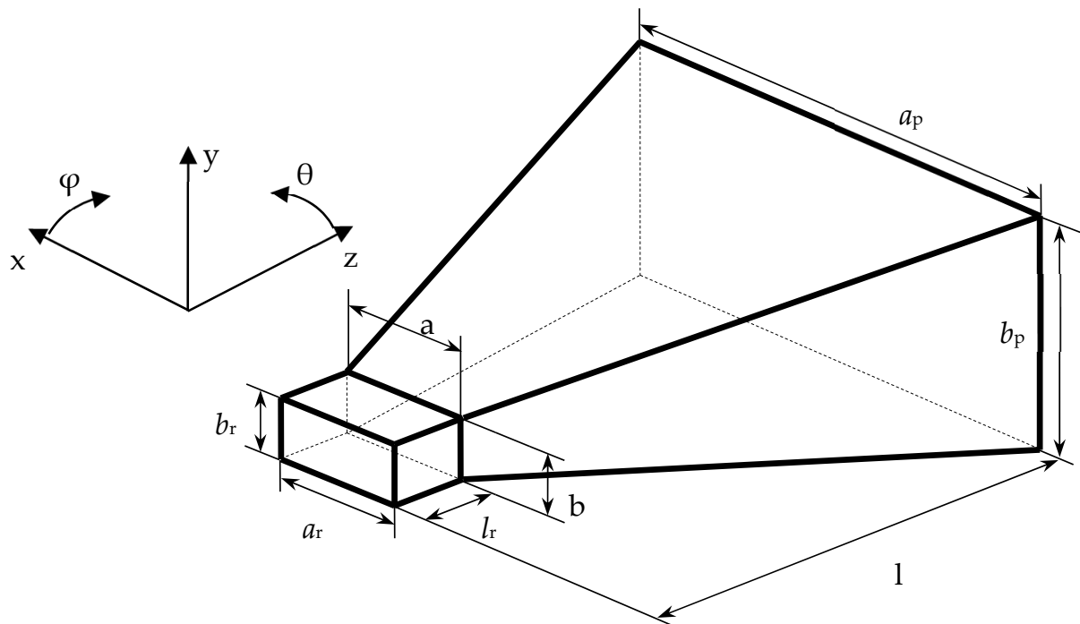
Figure 17. The isometric view of the inner surface of the horn AE.
