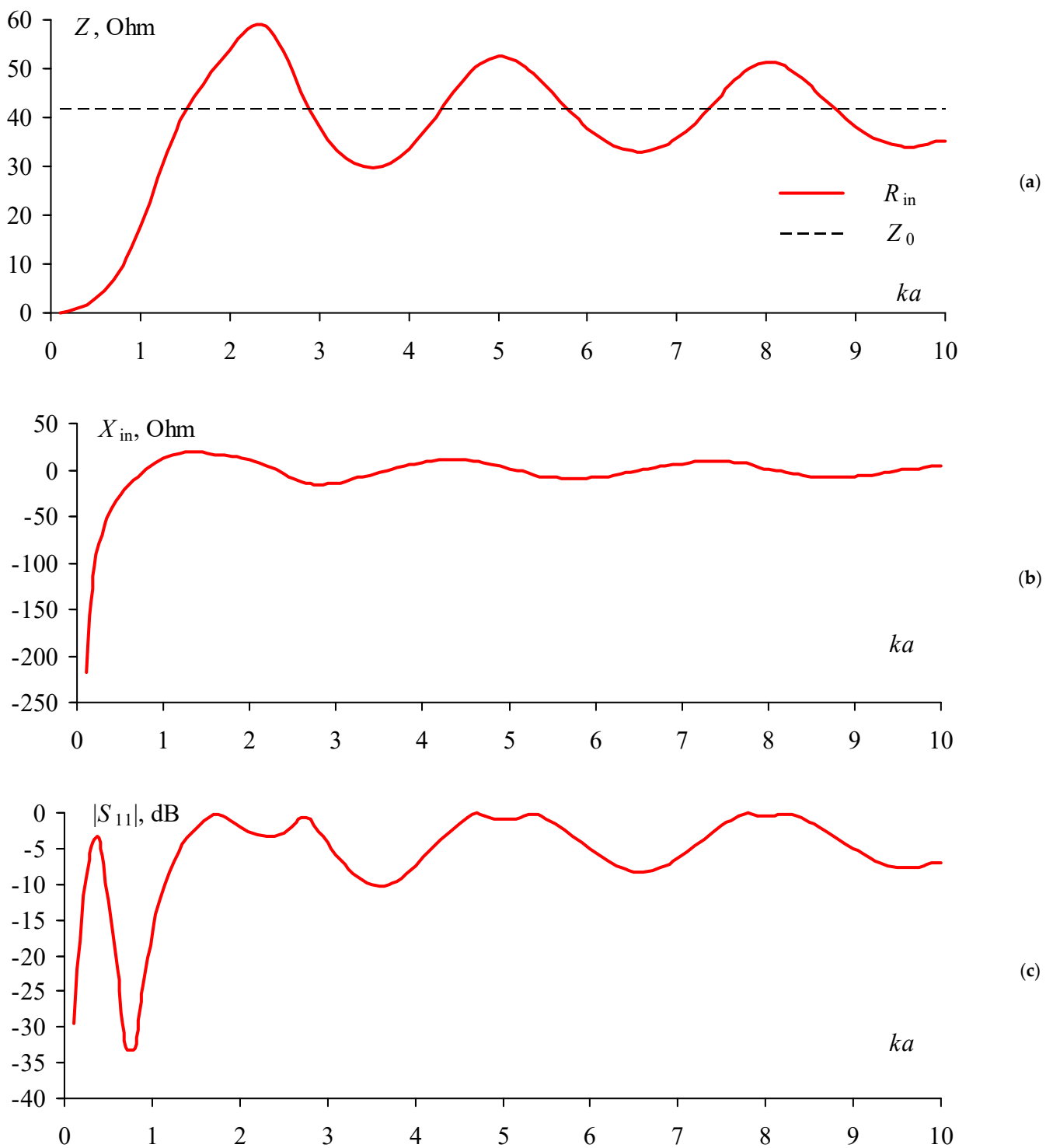
Figure A1. The dependences on ka of: characteristic impedance Z_0 , the real R_{in} and the imaginary X_{in} parts of the input impedance Z_{in} , as well as |S_{11}| for the conical AE from Figure 9a with \Theta_0 = 53.1^\circ .
