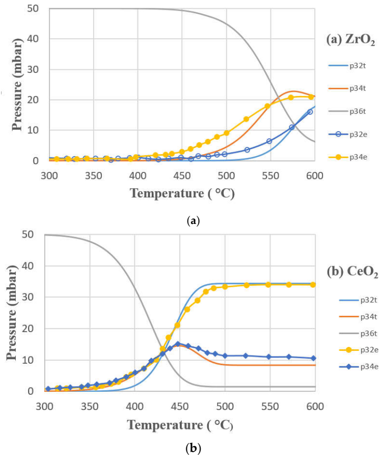
Figure 2. Calculated (lines) and experimental (points+line) [35,36] dependencies of partial pressures of oxygen species on temperature for catalyst ZrO 2 (a) and CeO 2 (b) during TPIE.
