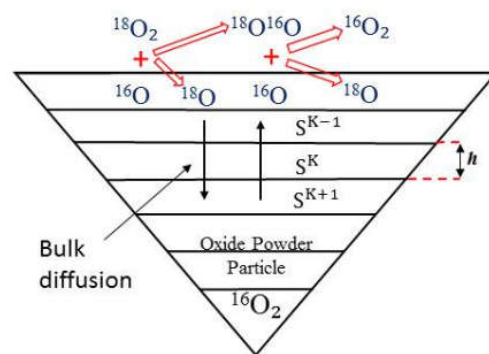
Figure 1. Scheme of the layers introduced for bulk diffusion calculations in particle of powder catalyst.
