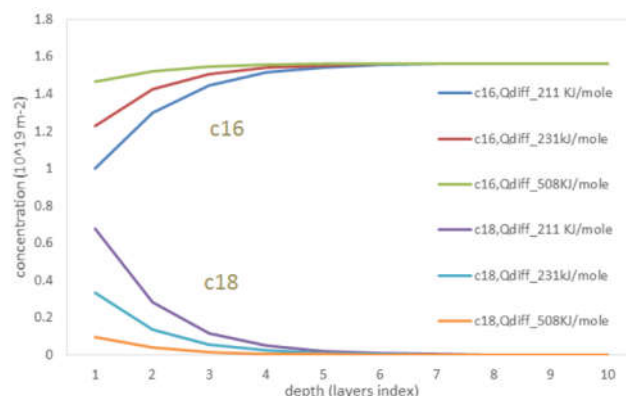
Figure 9. The depth profiles of oxygen atoms calculated at different values of Q_{diff} .
