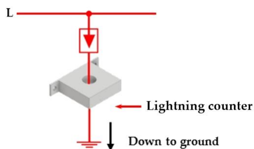
Figure 8. The lightning counter.
