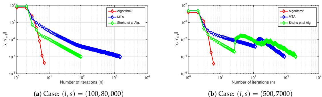
Figure 1. Illustration the behavior of \|y_n - y_{n-1}\| for Algorithm 2, MTA, and Shehu et al.'s algorithm in Equation (3).
