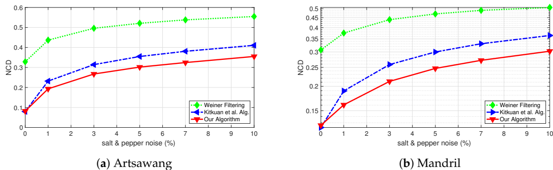
Figure 6. (a,b) The behavior of NCD in motion blur and different different salt and pepper noise from 0% to 10%.
